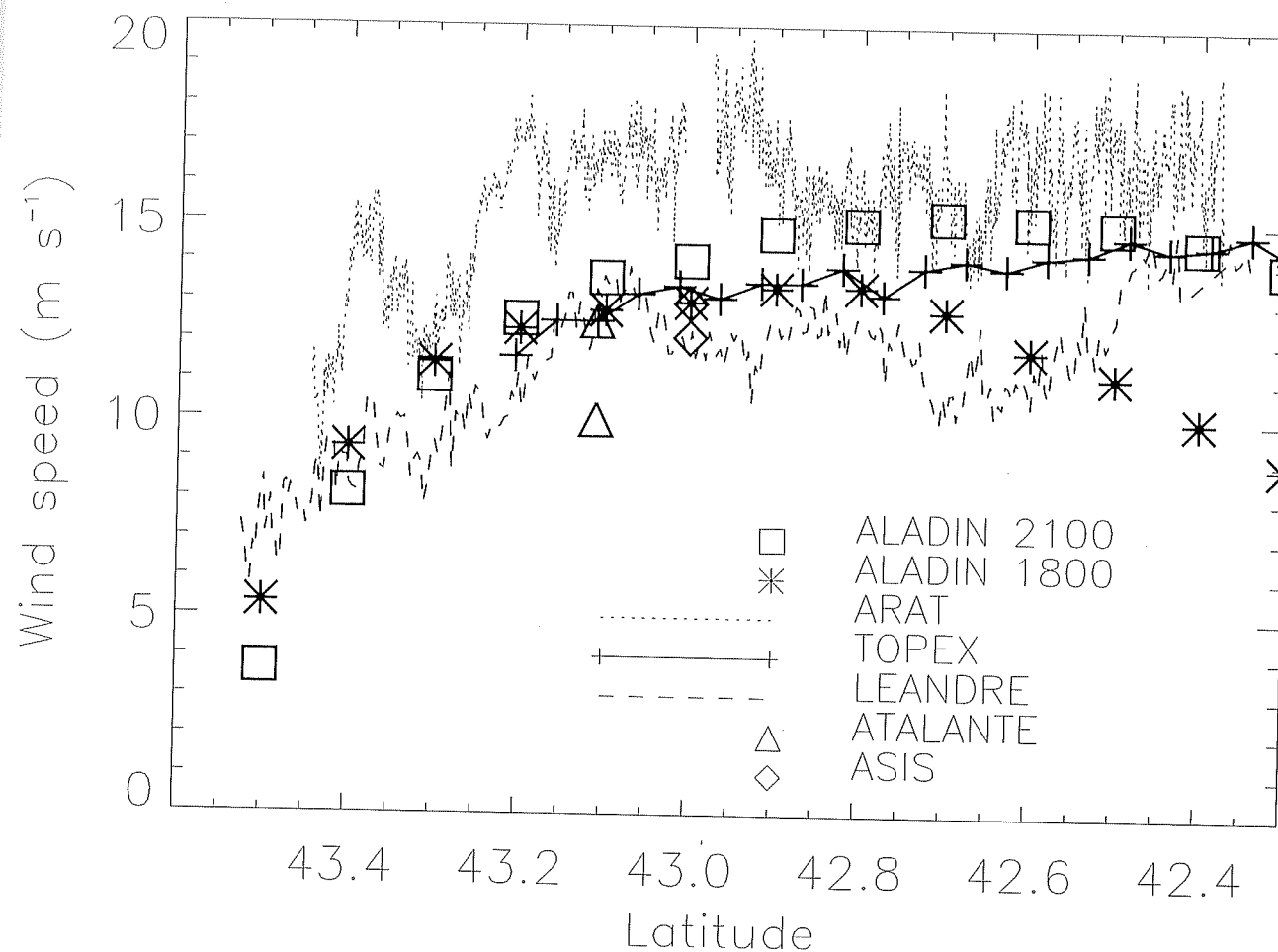
Figure 8. Comparison of sea-borne (7 m ASL, diamonds), ship-borne (17 m ASL, triangles), airborne lidar (12.4 m ASL, dashed line), airborne in situ (100 and 300 m ASL, connected crosses) SWS measurements along leg AF with SWS simulated by ALADIN at 1800 UTC (10 m ASL, asterisks) and 2100 UTC (squares).
