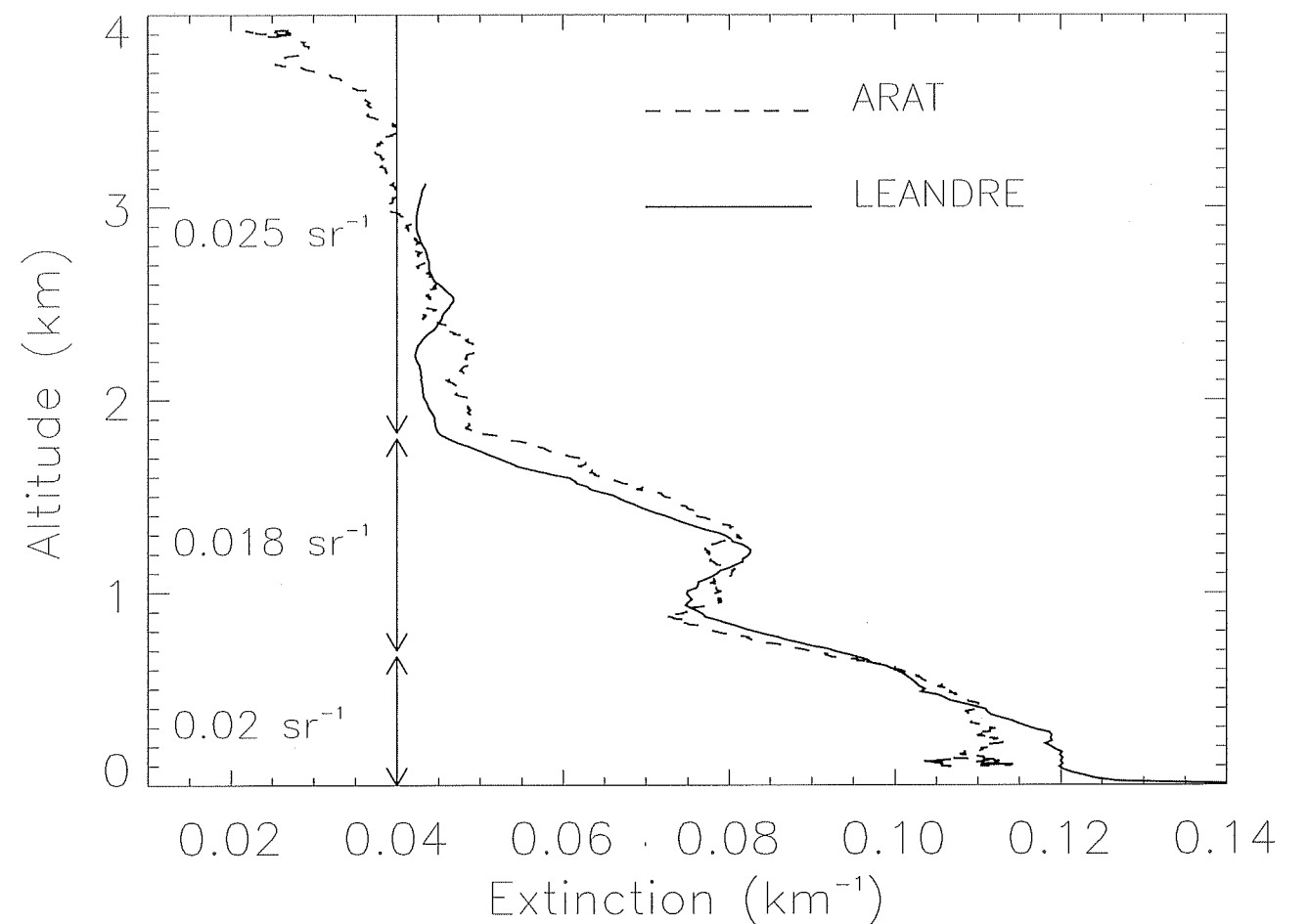
Figure 15. Comparison between the lidar-derived (solid line) and in situ nephelometer (dashed line) total extinction coefficient profile at 550 nm. Also indicated are the BER values (0.02, 0.018 and 0.025 sr -1 ) used to derived the particle extinction coefficient from lidar data.
