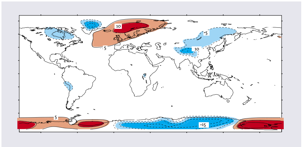
Figure 3.1.1. Deviation of the annual average surface air temperature from its zonal average. Note the anomalously high temperatures over the Northeast Atlantic and northern Europe, and anomalously cold areas over Greenland. (Source: Potsdam Institute for Climate Impact Research, 1999).
