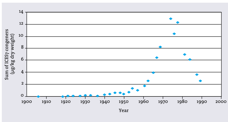
Figure 3.5.5. PCB concentrations in a dated saltmarsh core from Banks Marsh, Northwest England ( \mu\text{g}/\text{kg} dry weight). (Source: Matthiessen and Law, 2002. In Environmental Pollution).
