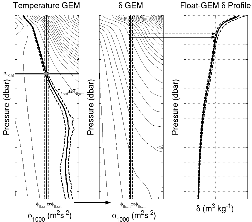
Figure 5. Diagram illustrating the float-GEM technique. The streamfunction value ( \phi_{float} ) corresponding to a given float station is found by looking up the ( p_{float}, T_{float} ) pair on the temperature GEM field (left panel). Once \phi_{float} is known, it is used to estimate the specific volume anomaly profile from its respective GEM field (middle panel). Then, the estimated specific volume anomaly profile is obtained and plotted in the right panel. The diagram also illustrates the float-GEM error associated with errors in the float temperature measurement ( \epsilon T_{float} ) generating an uncertainty in the determination of the streamfunction value ( \phi_{float} \pm \epsilon \phi_{float} ) (left panel), which in turn generates an uncertainty in the estimate of the specific volume anomaly profile (middle and right panels). See Appendix B for details on the float-GEM errors.
