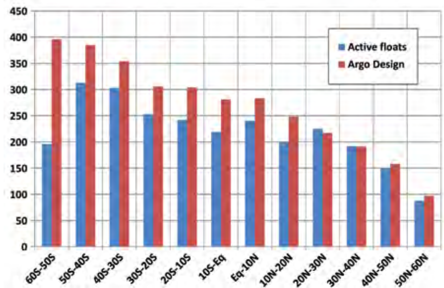
Figure 2. Blue bars show the number of Argo floats per 10° of latitude providing good profile data as of March 2009, excluding those in marginal seas. Red bars show Argo's design requirement for 3° x 3° open ocean sampling.
