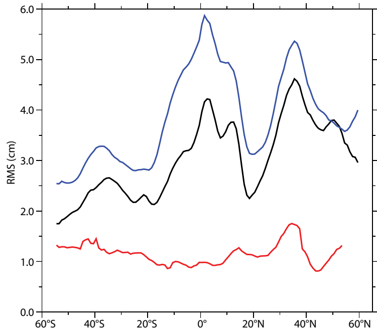
Figure 5. Zonally averaged large-scale ( 10^{\circ} \times 10^{\circ} \times 3 -month) nonseasonal sea surface height signal (blue) and Argo sampling noise (red) for 15 years of sustained Argo sampling at the 2007 level, estimated from satellite altimetry (see text). The black line shows how the apparent signal is reduced in a shorter (four-year) record. Results adapted from Roemmich and Gilson (2009)
