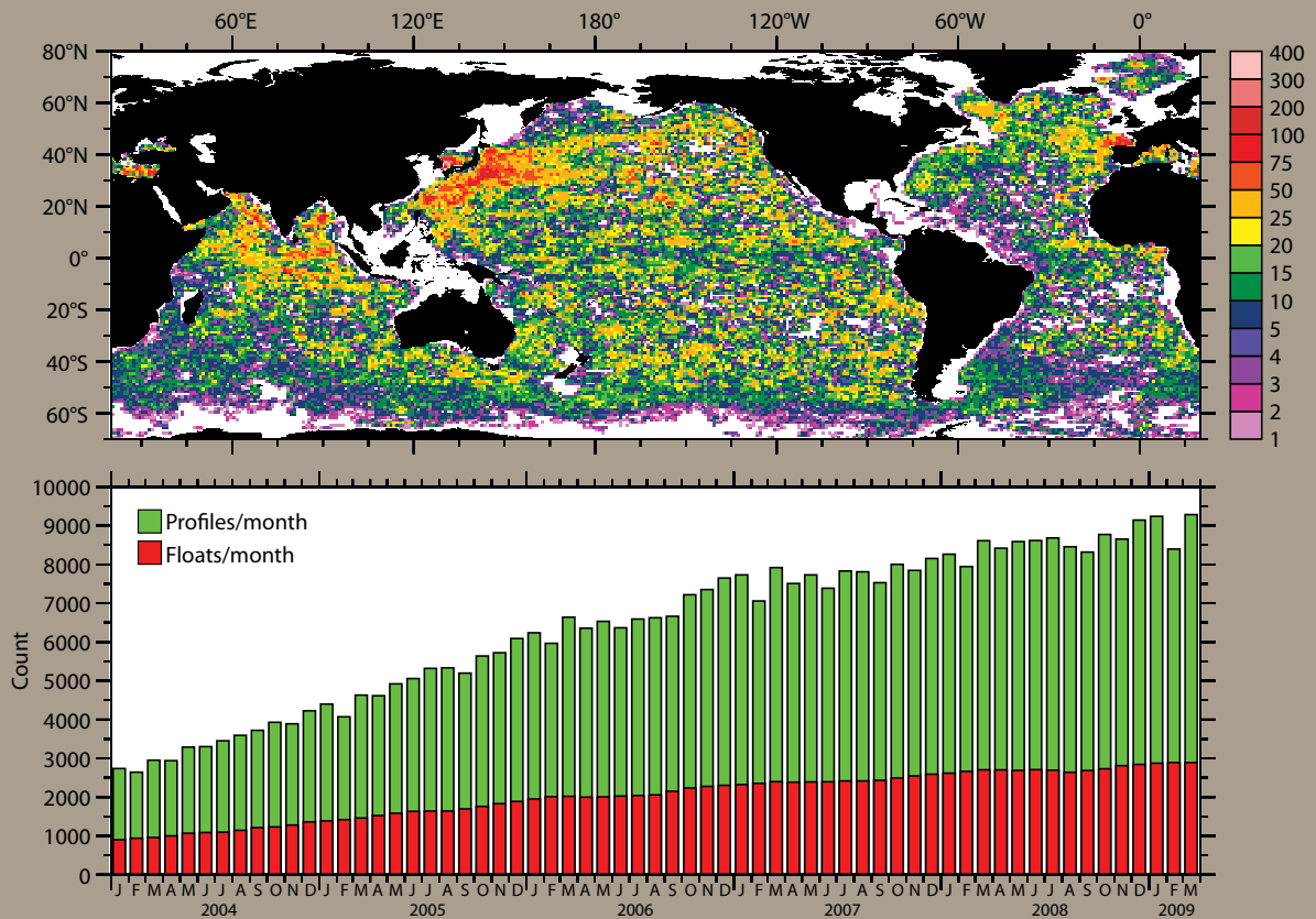
Figure 1. (Top) Map of the number of good Argo profiles obtained in each 1^\circ \times 1^\circ box during the period January 2004 to March 2009. (Bottom) Number of floats per month (red) providing good data and number of good profiles per month (green).
