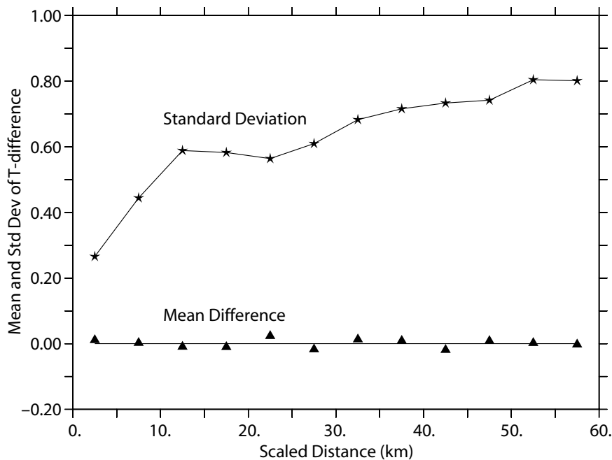
Figure 6. Argo-minus-surface-drifter mean and standard deviation of temperature difference ( ^{\circ}\text{C} ) as a function of “scaled distance” (see text), in 5-km bins, for 21,100 nearby pairs of observations.
