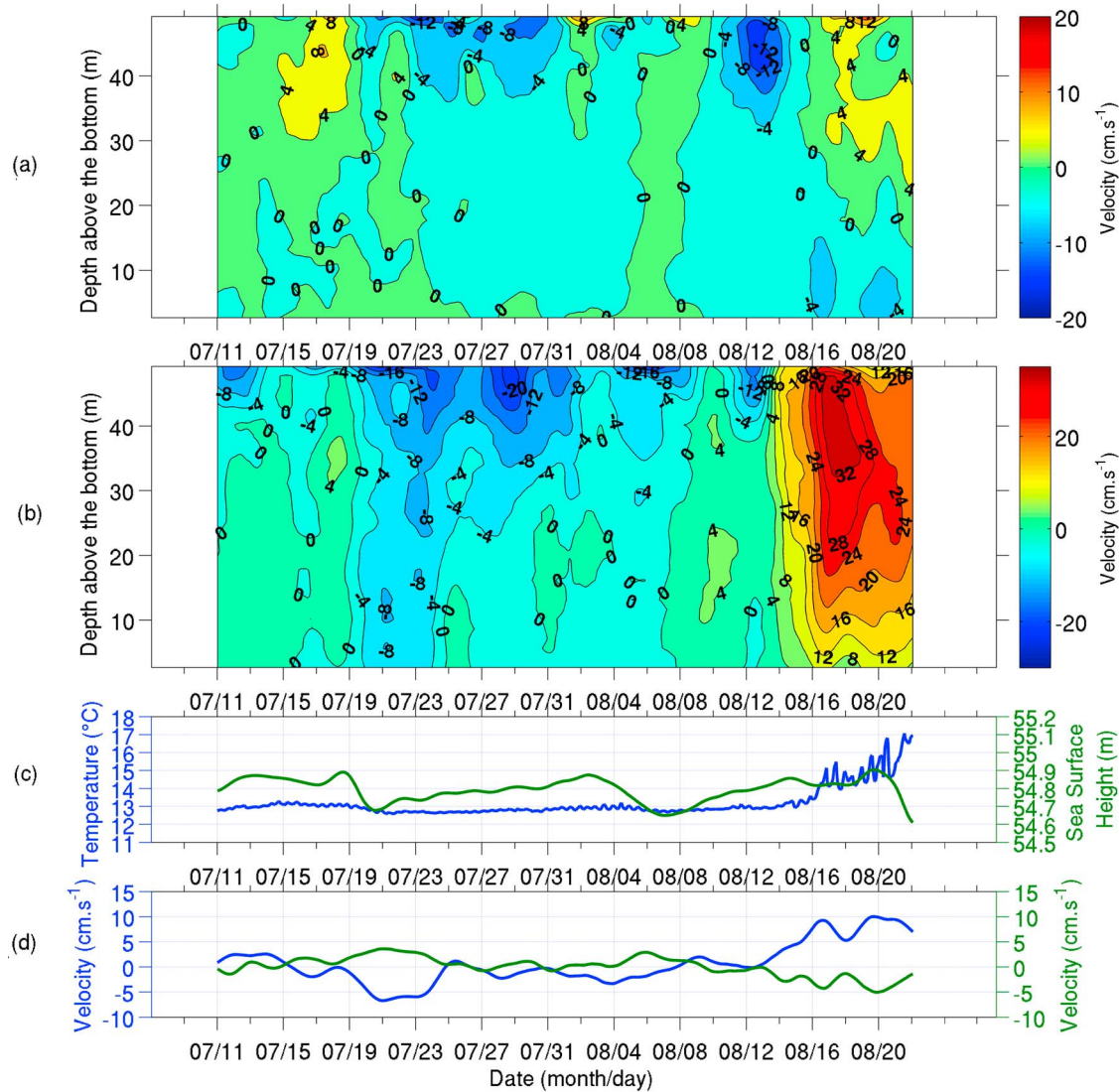
Figure 3. Acoustic Doppler current profiler (ADCP) 2008 data: (a) cross-shore velocity, U ; (b) longshore velocity, V ; (c), bottom temperature (54 m depth) and sea surface height (SSH); and (d) cross-shore (in green) and longshore (in blue) bottom velocities.
