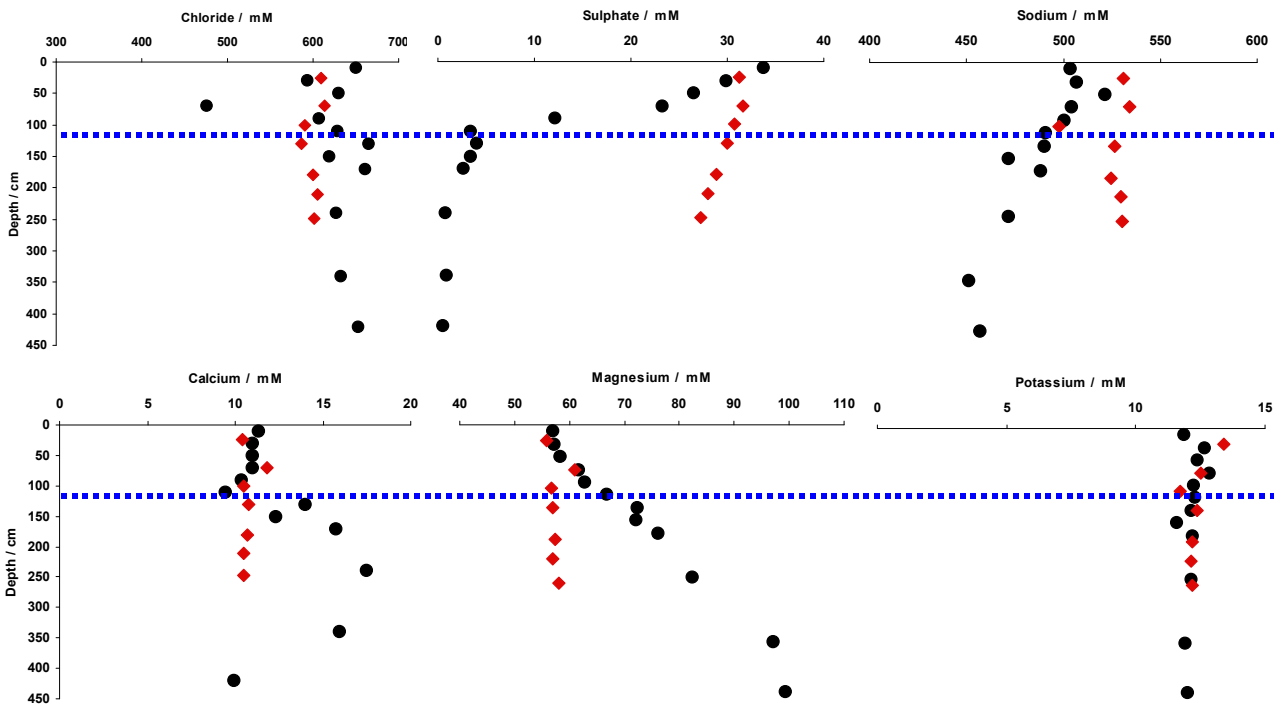
Fig. 7. Pore-fluid concentration profiles of selected dissolved-elements. The red diamonds correspond to MARM_1 and the black dots to MARM_2. The dashed blue line corresponds to the SML.
