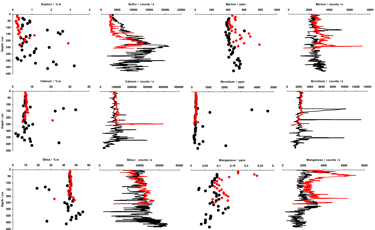
Fig. 9. Sedimentary profiles of selected elements determined with a laboratory XRF instrument (symbols, where the red diamonds are for MARM_1 and black dots for MARM_2) and a XRF core scanner (full line).
