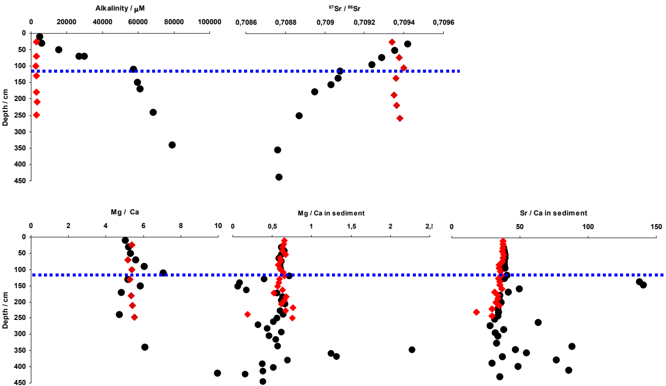
Fig. 8. Alkalinity and strontium isotope profiles in the pore fluid, and Mg/Ca and Sr/Ca in both the pore fluid and the sediment.
