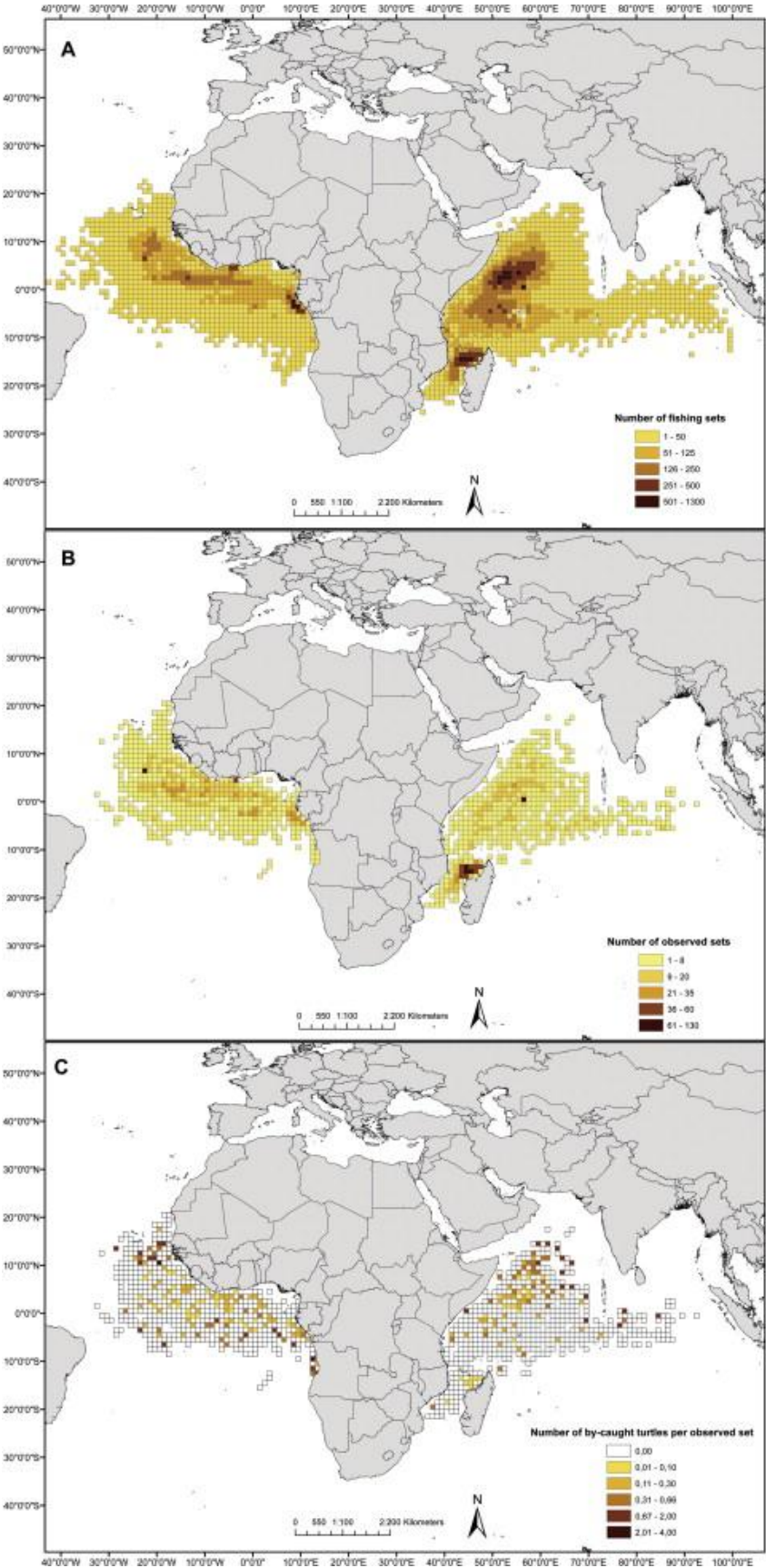
Figure 2: Total number of purse-seine sets on DFADs (A), observed sets on DFADs (B) and number of marine turtle bycatch per observed set on DFADs (C) per statistical square of 1° in the French and Spanish Purse seine fleet from 1995-2011 in the Atlantic and Indian oceans
