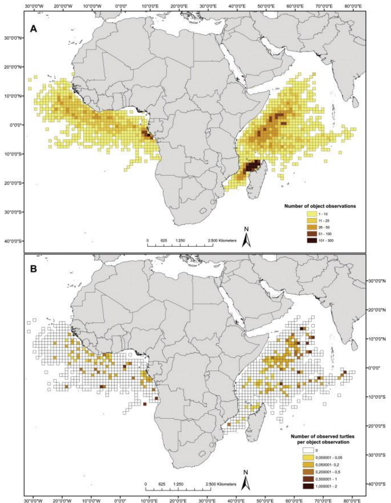
Figure 3: Total number of object observed (A) and number of observed marine turtles per object observation (B) per statistical square of 1° in the French and Spanish Purse seine fleet from 2003-2011 in the Atlantic and Indian Oceans
