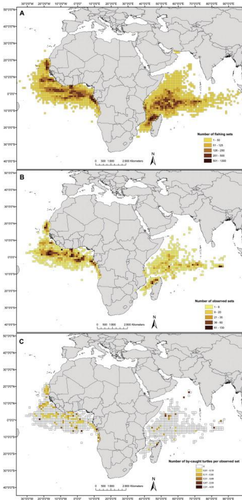
Figure 1: Total number of purse-seine sets on FSC (A), observed sets on FSC (B) and number of marine turtles bycatch per observed set on FSC (C) per statistical square of 1° in the French and Spanish Purse seine fleet from 1995-2011 in the Atlantic and Indian oceans
