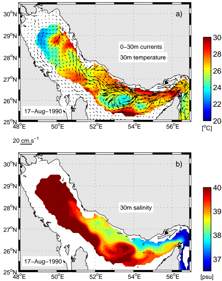
Fig. 4 Snapshot of temperature and velocity (only one arrow every 20 km is shown) in (a) and salinity (b) in August 1990. Currents are averaged over the upper 30m, while temperature and salinity are extracted at 30m depth.
