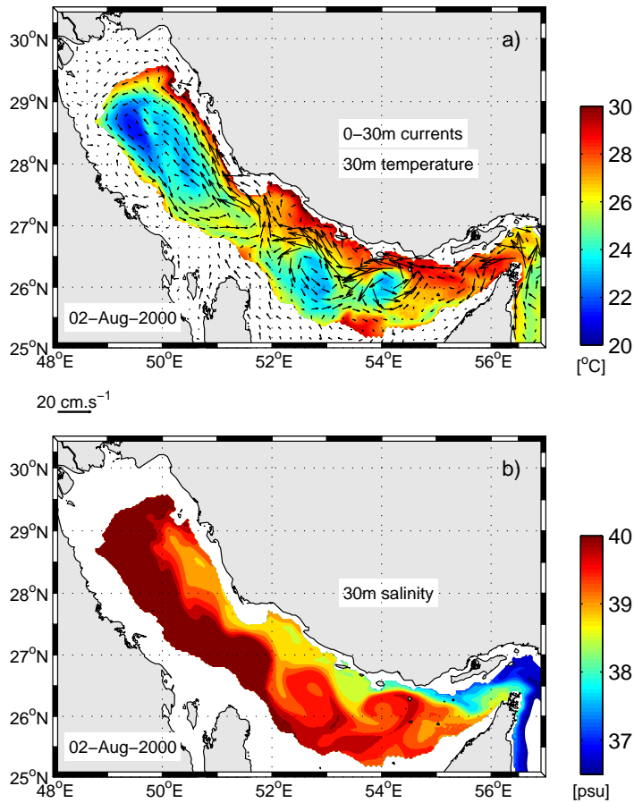
Fig. 11 Snapshot of temperature and velocity (only one arrow every 20 km is shown) in (a) and salinity (b) in August 2000 in INTER-HR. Currents are averaged over the upper 30m, while temperature and salinity are extracted at 30m depth.
