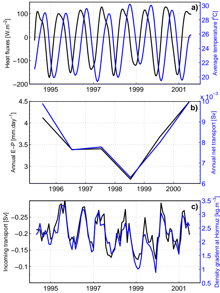
Fig. 6 (a) Surface heat fluxes ( Q_{\text{Total}} , positive from air to sea, black line) and averaged temperature over the Gulf (blue line). (b) Annual mean E-P above the Gulf (black line) and annual mean net transport across the Strait of Hormuz (blue line). (c) inflow transport at the Strait of Hormuz (black line) and difference in density at 75 m depth between PGW and IOSW (blue line).
