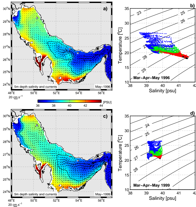
Fig. 7 Maps of (monthly averaged) surface salinity and currents in the Gulf in May 1996 (a) and in May 1999 (c); isohaline 39 psu is located by the black line. Temperature-Salinity diagram in spring in the central region of the Gulf in 1996 (b) and in 1999 (d).
