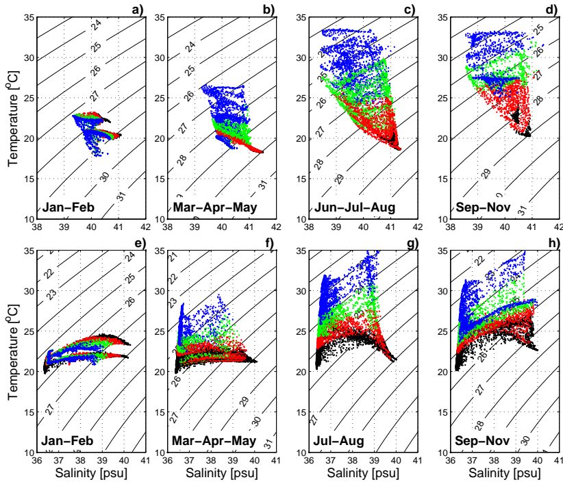
Fig. 5 Seasonal Temperature-Salinity diagram in the central region of the Gulf (top, see boxes in figure 1) and in the Strait of Hormuz (bottom), at selected depth intervals (5-20m in blue; 25-35m in green; 40-55m in red and 60-100m in black), based on monthly temperature and salinity.
