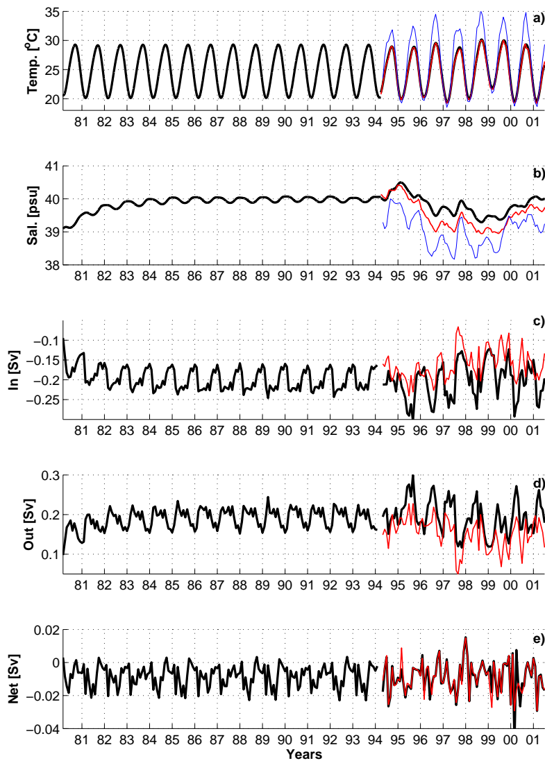
Fig. 2 Time evolution of (a) temperature averaged over the Gulf for years 1981-1994 (CLIM, black line) and 1994-2001 (INTER, black line and INTER-HR, red line); (b) salinity averaged over the Gulf (same color coding as for temperature); (c) inflow, (d) outflow and (e) net transports across the Strait of Hormuz (monthly data, in Sv, CLIM and INTER in black, INTER-HR in red). Upper panels also show the monthly SST (a, blue line) and SSS (b, blue line) from INTER for years 1994-2001.
