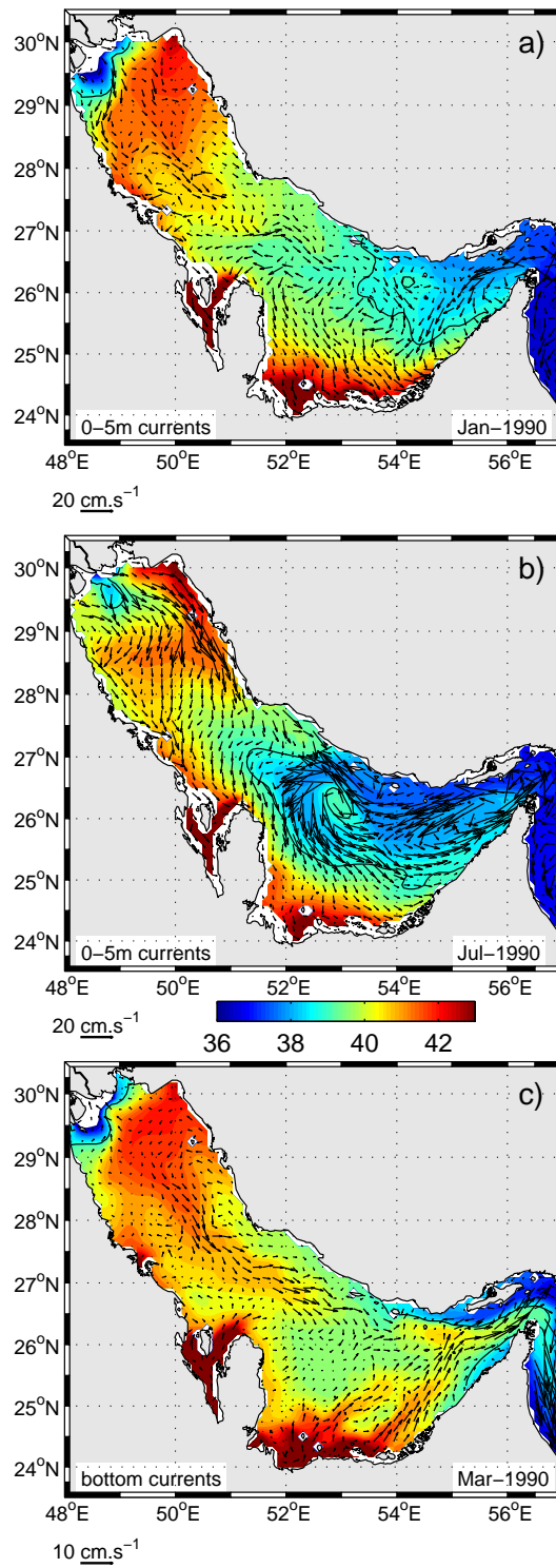
Fig. 3 Monthly averaged salinity and velocity (only one arrow every 20 km is shown) at the surface in January (a), July (b) and at the bottom in March (c). Isohaline 39.0 is located by the black line.
