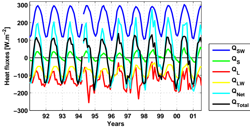
Fig. 13 Interannual time series of the (monthly averaged) heat fluxes in \text{W/m}^2 for the Persian Gulf (spatially averaged over the basin): Q_{SW} is the short-wave heat flux, Q_S the sensible heat flux, Q_L the latent heat flux, Q_{LW} the long-wave heat flux, Q_{Net} the net heat flux and Q_{Total} the total heat flux.
