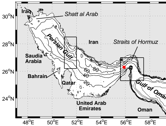
Fig. 1 Boundary of the 3D model domain; bathymetry over the Persian Gulf. The red square indicates the position of the modeled time series of temperature and salinity to compare to [17] mooring site. Black boxes show the location where temperature-salinity diagrams have been constructed for comparison with observations.
