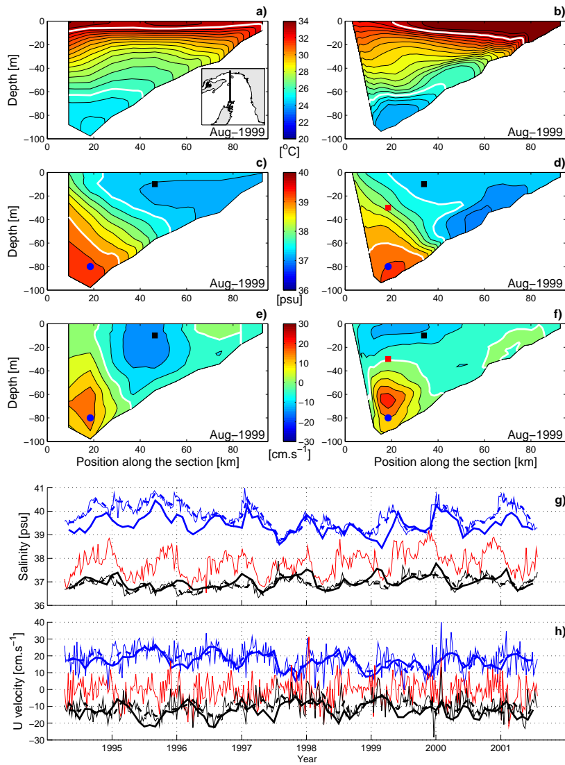
Fig. 8 Cross-sections of temperature (a, b), salinity (c, d) and normal velocity (e, f) at Hormuz for INTER (left panels, a, c, e) and INTER-HR (right panels, b, d and f) averaged over the month of August 1999; time series of salinity (g) and normal velocity (h) in the IOSW inflow (blue lines), in the deep PGW outflow (black lines) and at 35 m depth, above the deep outflow (red line, only for INTER-HR), monthly averaged for INTER (thick lines) and INTER-HR (dashed lines). The location of the section is shown on the subset of panel a, while the points where time series are extracted are shown by a black square (inflow), a blue circle (deep outflow) and a red square (35 m depth, above the deep outflow) in panels c-f. In the cross-sections, white lines locate 26 and 33°C isotherms, 37.5 and 39 isohalines and 0 cm/s isotach. For INTER-HR, the time series are also shown at higher frequency (7-day outputs filtered by Demerliac, thin lines).
