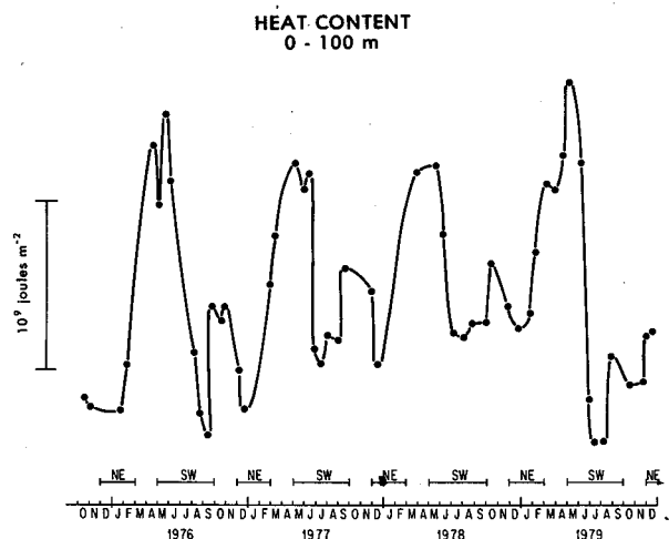
Figure 4 Heat storage from XBTs in the 0-100 m layer between 2°N-12°N in the Somali Basin from October 1975 to December 1979 along tanker sea-lane (Fig. 1) with duration of northeast (NE) and southwest (SW) monsoons given. Vertical scale length is 10 9 Jm -2 .
