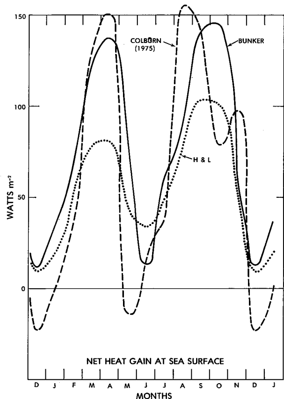
Figure 3 Net heat gain at the sea surface in Somali Basin. Bunker distribution calculated according to Bunker (1976) within basin region approximately 2°N-12°N; H & L is Hastenrath and Lamb (1979), their Figure 16; Colborn (1975), his Figure 25.
