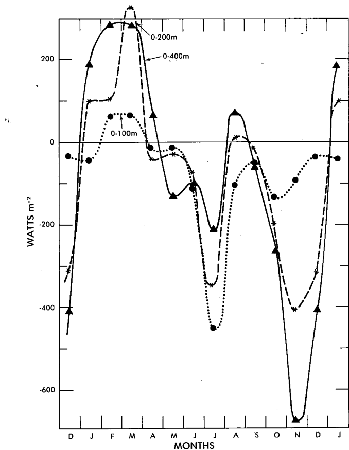
Figure 7 Rate of heat storage minus sea surface heat gain from Bunker's values (Fig. 3). Curves represent residual caused by horizontal advection and vertical displacement and diffusion of heat.
