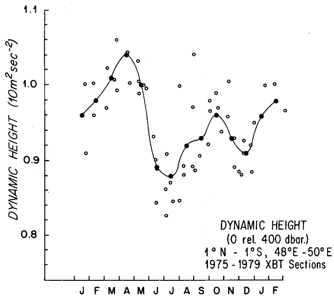
Figure 8 Geopotential anomaly of sea surface (0 rel. 400 dbar) at equator from 1975-1979 tanker XBT observations. Fixed T-S relation used in determinations (Bruce, 1979). Curves connects monthly means (solid dots). Standard deviation of "individual" observations (open dots) is \pm 0.04 (10 \text{ m}^2 \text{ s}^{-2}) . Each "individual" observation is generally an average of 5 stations between 1°S-1°N along sea-lane (Fig. 1).
