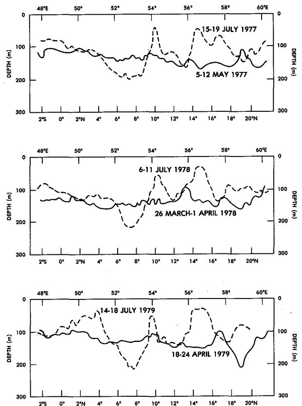
Figure 2 Examples of depth (m) of 20°C isotherm (mid-thermocline) of pre-monsoon (March, April, May) and southwest monsoon (July) conditions along tanker sea-lane (Fig. 1).
