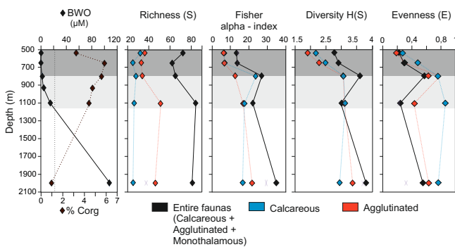
Figure 3. Stained foraminiferal diversity indices (in the > 150 μm fraction) along the sampling transect. The C org content (wt. %) is from Hunter et al. (2012) and Cowie et al. (2014). The dashed line corresponds to the 22 μM limit defining an OMZ according to Levin et al. (2003). The dark-grey shadow represent the core of the OMZ (< 2 μM; Paulmier and Ruiz-Pino, 2009) and the light-grey shadow the lower part of the OMZ (2–22 μM; Levin, 2003).
