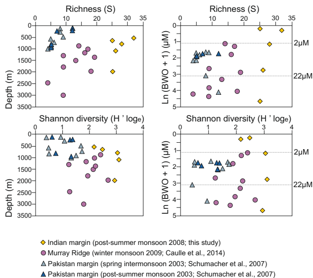
Figure 6. Species richness and Shannon index (calculated for the calcareous fauna only) vs. depth (m) and \text{Ln}(\text{BWO}+1) for the Indian margin, the Pakistan margin and the Murray Ridge. Because some values were < 1 , the BWO was expressed using the natural logarithm + 1 ( \text{Ln}(\text{BWO}+1) ). The dash lines correspond to the limits of the OMZ core ( 2 \mu\text{M} ) and to the lower boundary of the OMZ ( 22 \mu\text{M} ).
