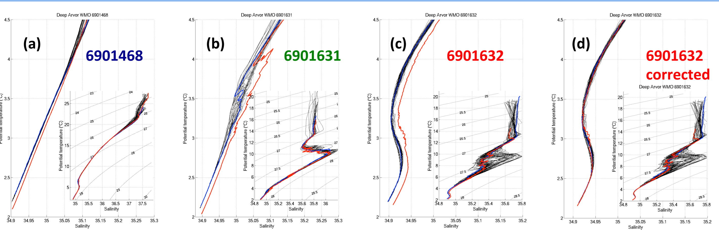
Figure 3: Theta/S diagram of the profiles collected by (a) float 6901468, (b) float 6901631, (c) float 6901632 and (d) 6901632 in using the corrected salinity following the OW method. The floats are identified by the blue, red and green stars on Figure 1, respectively. On each panel, the large figure is the theta/S diagram in the deep layers while the theta/S diagram in the inner plot represent the diagram for the full water-column. (Black curves) Deep-Arvor floats data. (Red curves) Calibrated reference profiles collected at float deployment. (Blue curves) Nearest float profile compared to the calibrated reference profile.
