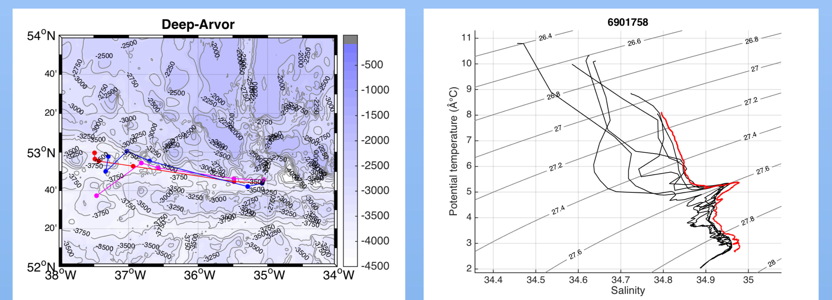
Figure 5: (Left panel) Trajectory of the 3 Deep Arvor deployed in the Charlie Gibbs Fracture Zone in 2015. (Right panel) (Black curves) Data of float 6901758 (Red curves) Pre-calibrated reference profiles collected at float deployment.
