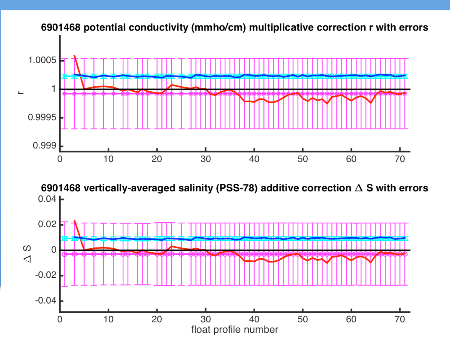
Figure 4: Correction proposed by the OW method for Deep-Arvor floats 6901468 (identified by blue stars on Figure 1). (Upper panel) The red (blue) curve represents the conductivity correction term for each profile while the magenta (cyan) line is the final correction term with one standard error when considering layers shallower than 2000 dbar (layer deeper than 3000 dbar). (Lower panel) Same as upper panel but for the vertically averaged salinity correction.
