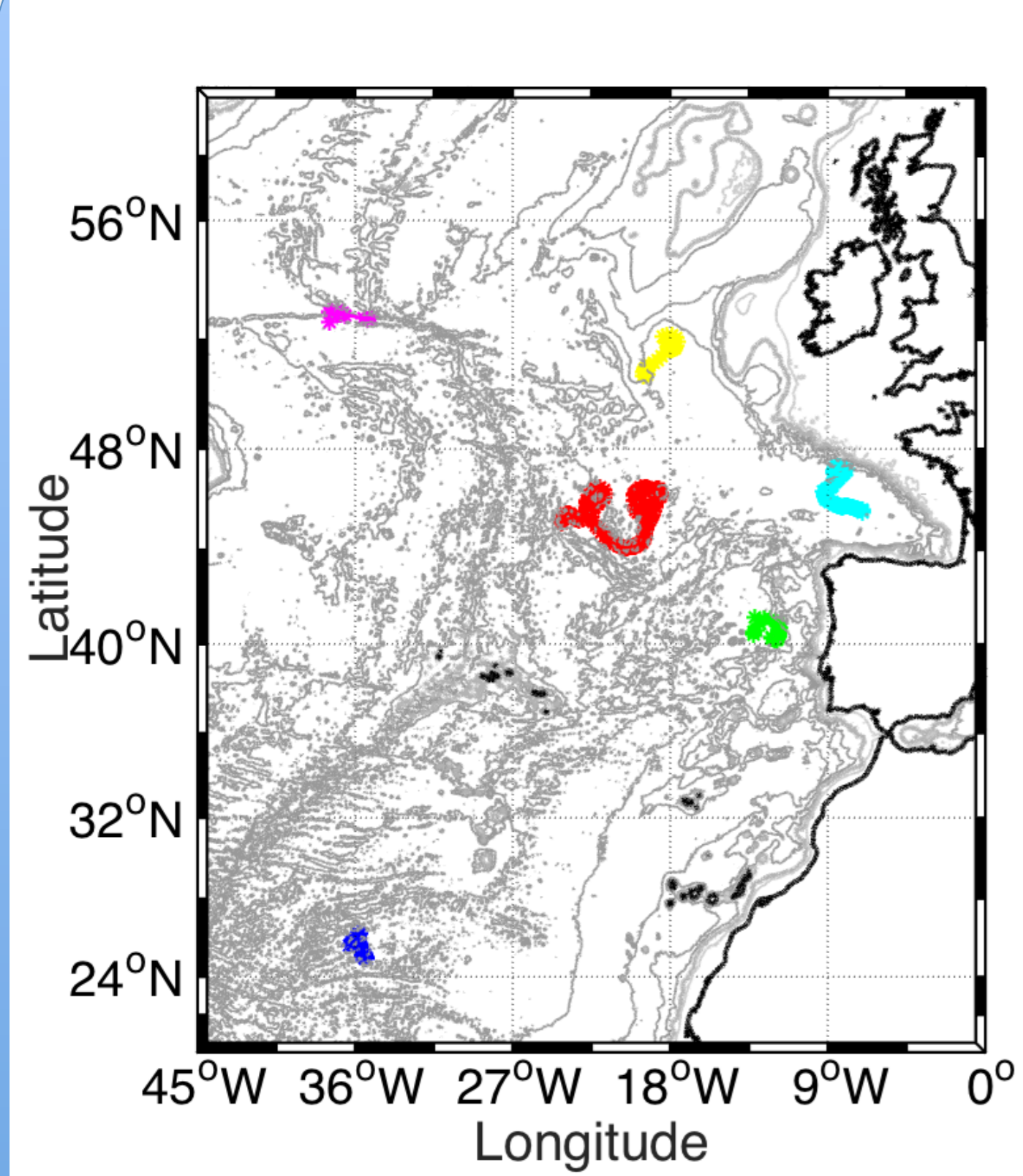
Figure 1: Positions of the 8 Deep-Arvor deployed in the North-Atlantic since 2012.
