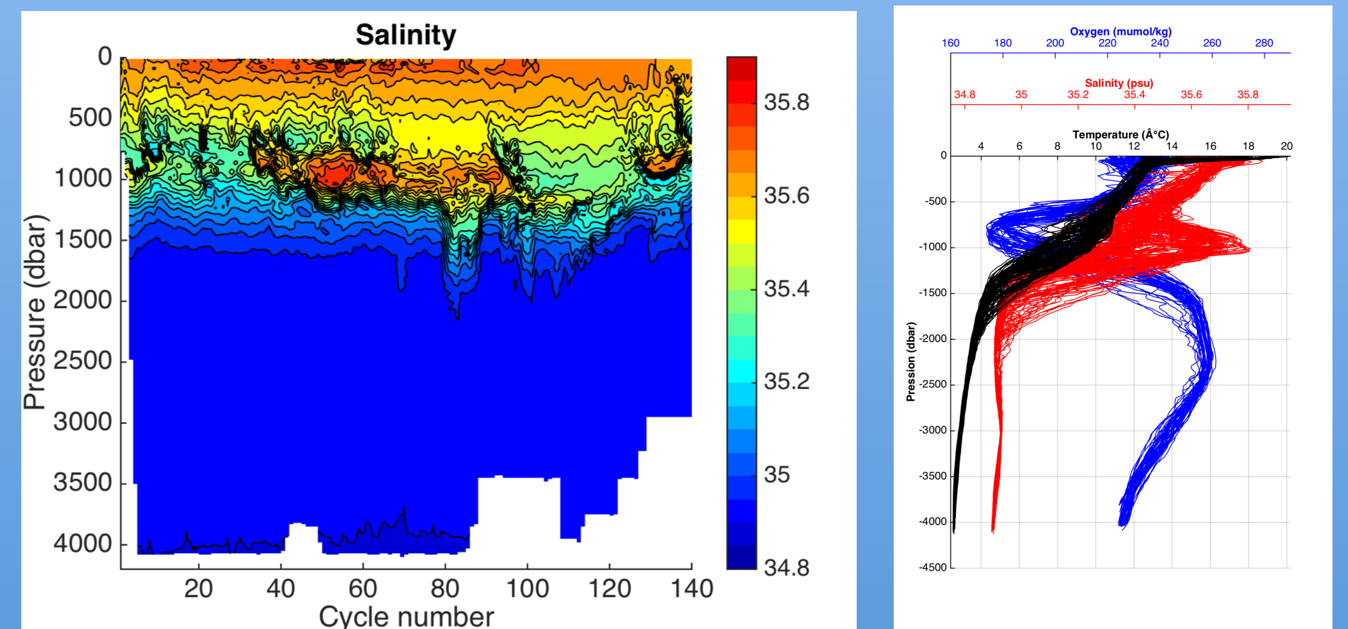
Figure 2: Data of float 6901632 (red stars on Figure 1) that acquired 142 cycles (1/3 of the profiles measured O2) down to 4000m depth or the bottom. (Left panel) Salinity section. (Right panel) Vertical profiles of temperature, salinity and oxygen.
