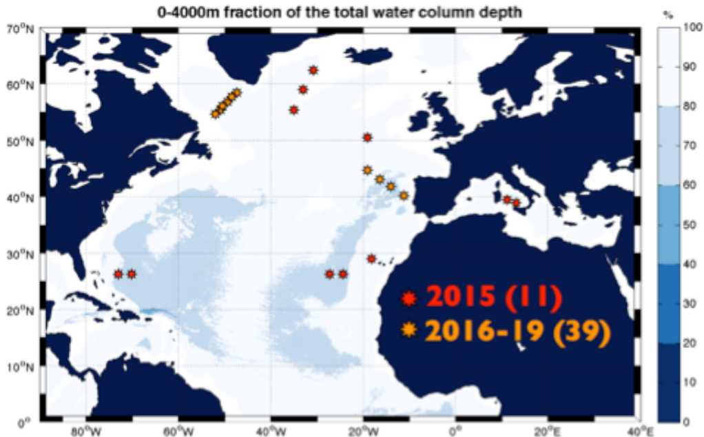
Figure 3: Location of planned Deep Arvor and Deep SOLO float deployments in the North Atlantic Ocean in 2015 (red stars) and 2016 to 2019 (orange stars).
