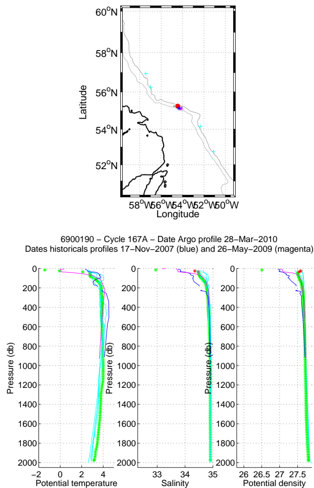
Figure 42: Flotteur 6900190, cycle 167. Upper panel: Position of the analysed CTD profile (red) and of the nearest CTD profiles (black). The nearest CTD profile in time is in magenta while the nearest CTD profile in space is in blue. Lower panels: Temperature, salinity and potential density as function of pressure for the analysed CTD profile (stars) and for the nearest CTD profile in time (magenta line) and for the nearest CTD profile in space (blue line). The color of the analysed CTD profile represents the QC flag (green for a QC=1; blue for a QC=2; orange for a QC=3 and red for a QC=4).
