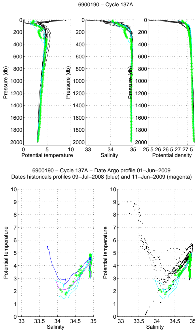
Figure 37: Float 6900190, cycle 137A. The analysed Argo profile (stars) is compared to the nearest Argo profiles (black line) and to two specific profiles: the nearest Argo profile in time (magenta) and the nearest Argo profile in space (blue). The color of the analysed Argo profile represents the QC flag (green for a QC=1; blue for a QC=2; orange for a QC=3 and red for a QC=4). (Upper panels) Temperature (left panel), salinity (middle panel) and potential density (right panel) as function of pressure. (Lower panels) \theta/S diagrams.
