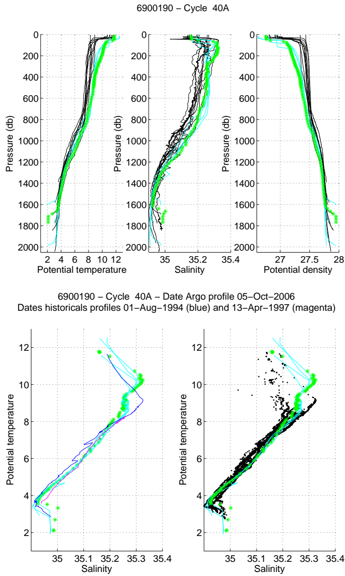
Figure 11: Float 6900190, cycle 40. The analysed CTD profile (stars) is compared to the nearest CTD profiles (black line) and to two specific profiles: the nearest CTD profile in time (magenta) and the nearest CTD profile in space (blue). The color of the analysed CTD profile represents the QC flag (green for a QC=1; blue for a QC=2; orange for a QC=3 and red for a QC=4). (Upper panels) Temperature (left panel), salinity (middle panel) and potential density (right panel) as function of pressure. (Lower panels) \theta/S diagrams.
