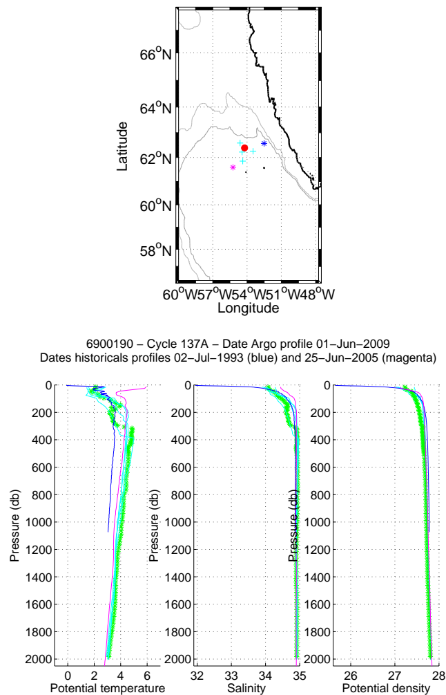
Figure 34: Flotteur 6900190, cycle 137. Upper panel: Position of the analysed CTD profile (red) and of the nearest CTD profiles (black). The nearest CTD profile in time is in magenta while the nearest CTD profile in space is in blue. Lower panels: Temperature, salinity and potential density as function of pressure for the analysed CTD profile (stars) and for the nearest CTD profile in time (magenta line) and for the nearest CTD profile in space (blue line). The color of the analysed CTD profile represents the QC flag (green for a QC=1; blue for a QC=2; orange for a QC=3 and red for a QC=4).
