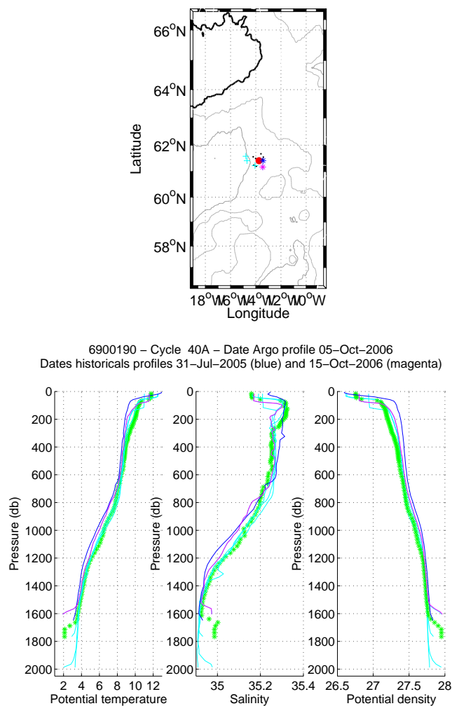
Figure 12: Flotteur 6900190, cycle 40. Upper panel: Position of the analysed Argo profile (red) and of the nearest Argo profiles (black). The nearest Argo profile in time is in magenta while the nearest CTD profile in space is in blue. Lower panels: Temperature, salinity and potential density as function of pressure for the analysed Argo profile (stars) and for the nearest Argo profile in time (magenta line) and for the nearest Argo profile in space (blue line). The color of the analysed Argo profile represents the QC flag (green for a QC=1; blue for a QC=2; orange for a QC=3 and red for a QC=4).
