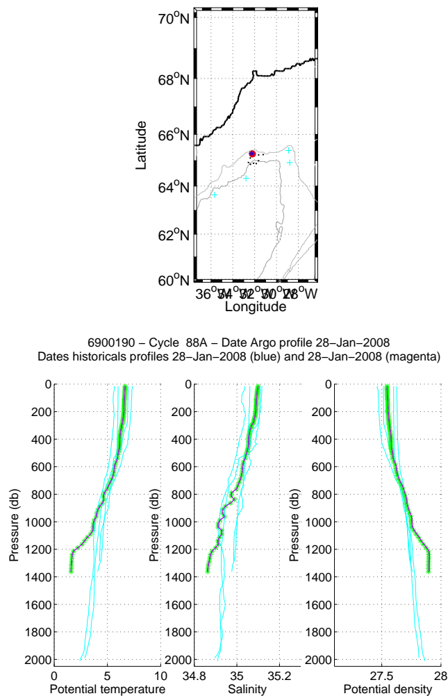
Figure 28: Flotteur 6900190, cycle 88. Upper panel: Position of the analysed Argo profile (red) and of the nearest Argo profiles (black). The nearest Argo profile in time is in magenta while the nearest CTD profile in space is in blue. Lower panels: Temperature, salinity and potential density as function of pressure for the analysed Argo profile (stars) and for the nearest Argo profile in time (magenta line) and for the nearest Argo profile in space (blue line). The color of the analysed Argo profile represents the QC flag (green for a QC=1; blue for a QC=2; orange for a QC=3 and red for a QC=4).
