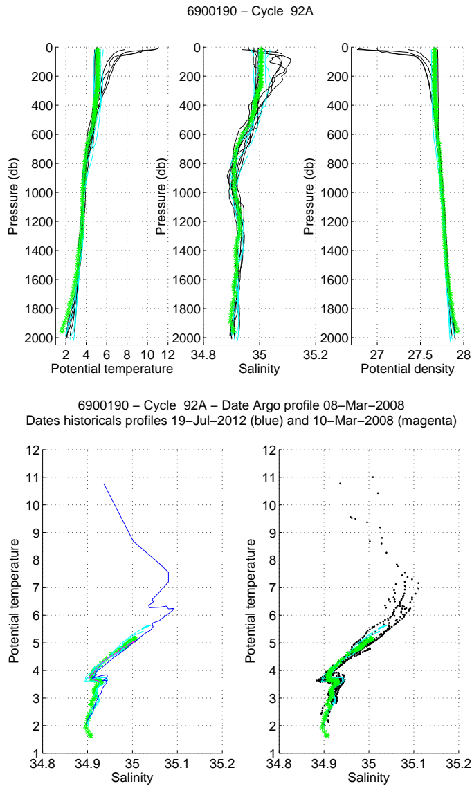
Figure 33: Float 6900190, cycle 92. The analysed Argo profile (stars) is compared to the nearest Argo profiles (black line) and to two specific profiles: the nearest Argo profile in time (magenta) and the nearest Argo profile in space (blue). The color of the analysed Argo profile represents the QC flag (green for a QC=1; blue for a QC=2; orange for a QC=3 and red for a QC=4). (Upper panels) Temperature (left panel), salinity (middle panel) and potential density (right panel) as function of pressure. (Lower panels) \theta/S diagrams.
