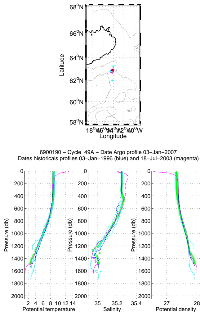
Figure 14: Flotteur 6900190, cycle 49. Upper panel: Position of the analysed CTD profile (red) and of the nearest CTD profiles (black). The nearest CTD profile in time is in magenta while the nearest CTD profile in space is in blue. Lower panels: Temperature, salinity and potential density as function of pressure for the analysed CTD profile (stars) and for the nearest CTD profile in time (magenta line) and for the nearest CTD profile in space (blue line). The color of the analysed CTD profile represents the QC flag (green for a QC=1; blue for a QC=2; orange for a QC=3 and red for a QC=4).
