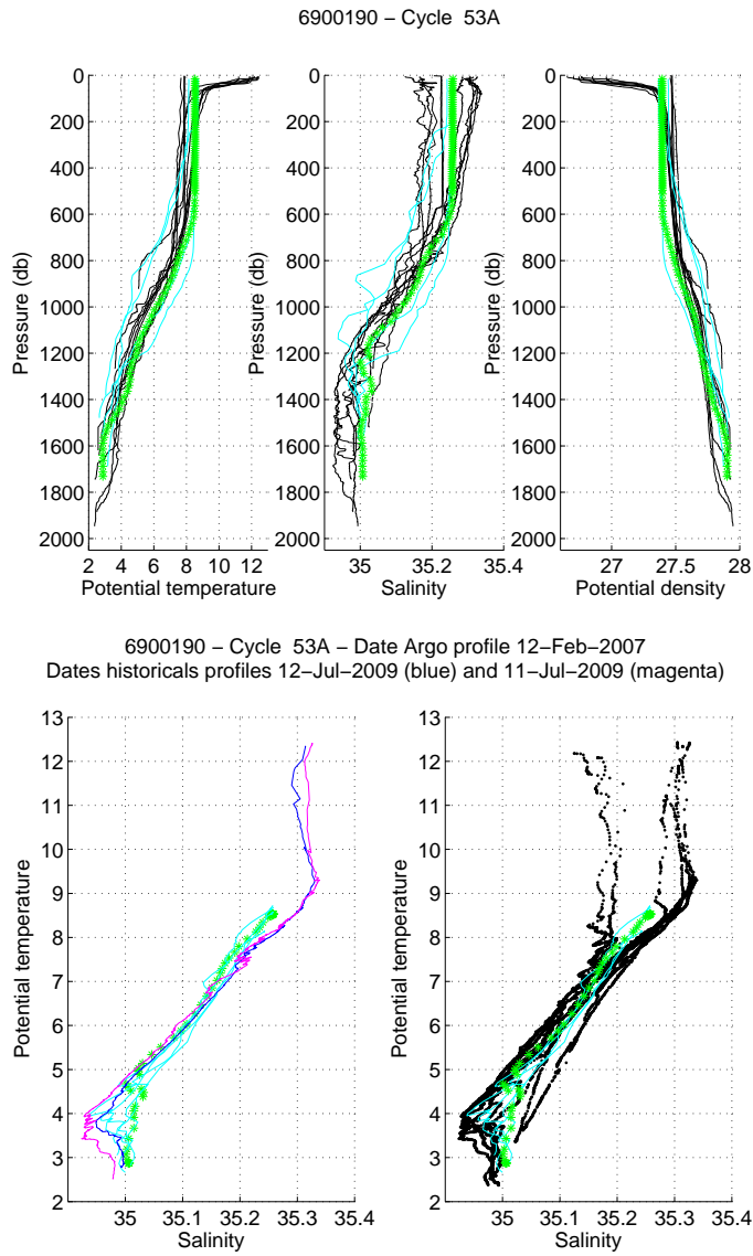
Figure 23: Float 6900190, cycle 53. The analysed CTD profile (stars) is compared to the nearest CTD profiles (black line) and to two specific profiles: the nearest CTD profile in time (magenta) and the nearest CTD profile in space (blue). The color of the analysed CTD profile represents the QC flag (green for a QC=1; blue for a QC=2; orange for a QC=3 and red for a QC=4). (Upper panels) Temperature (left panel), salinity (middle panel) and potential density (right panel) as function of pressure. (Lower panels) \theta/S diagrams.
