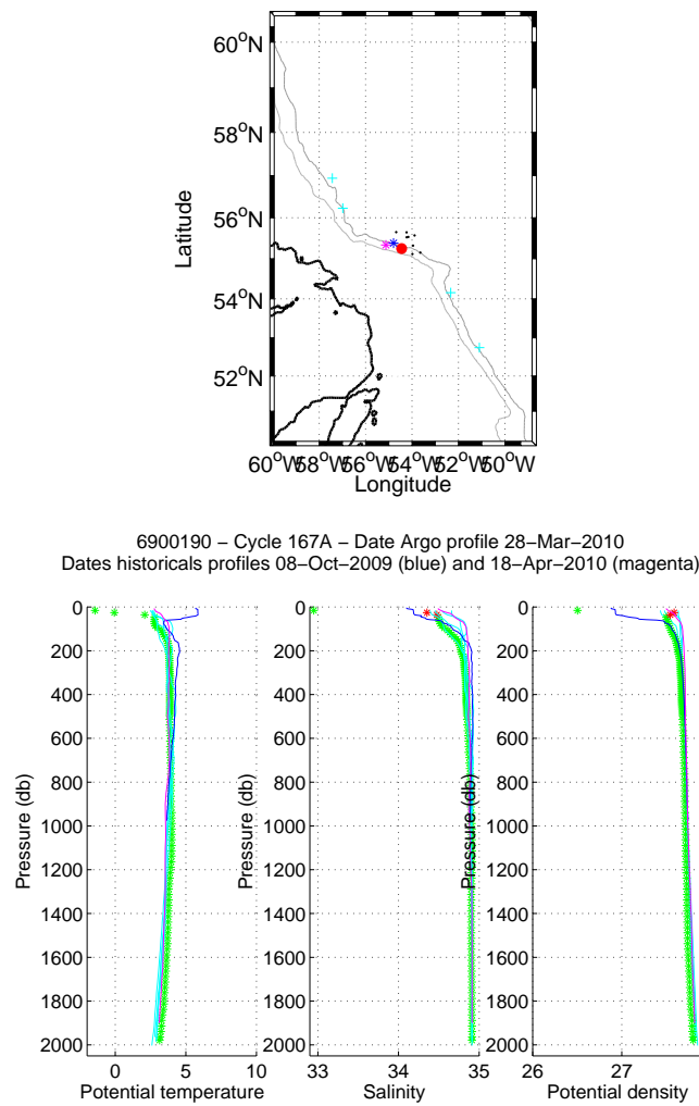
Figure 44: Flotteur 6900190, cycle 167. Upper panel: Position of the analysed Argo profile (red) and of the nearest Argo profiles (black). The nearest Argo profile in time is in magenta while the nearest CTD profile in space is in blue. Lower panels: Temperature, salinity and potential density as function of pressure for the analysed Argo profile (stars) and for the nearest Argo profile in time (magenta line) and for the nearest Argo profile in space (blue line). The color of the analysed Argo profile represents the QC flag (green for a QC=1; blue for a QC=2; orange for a QC=3 and red for a QC=4).
