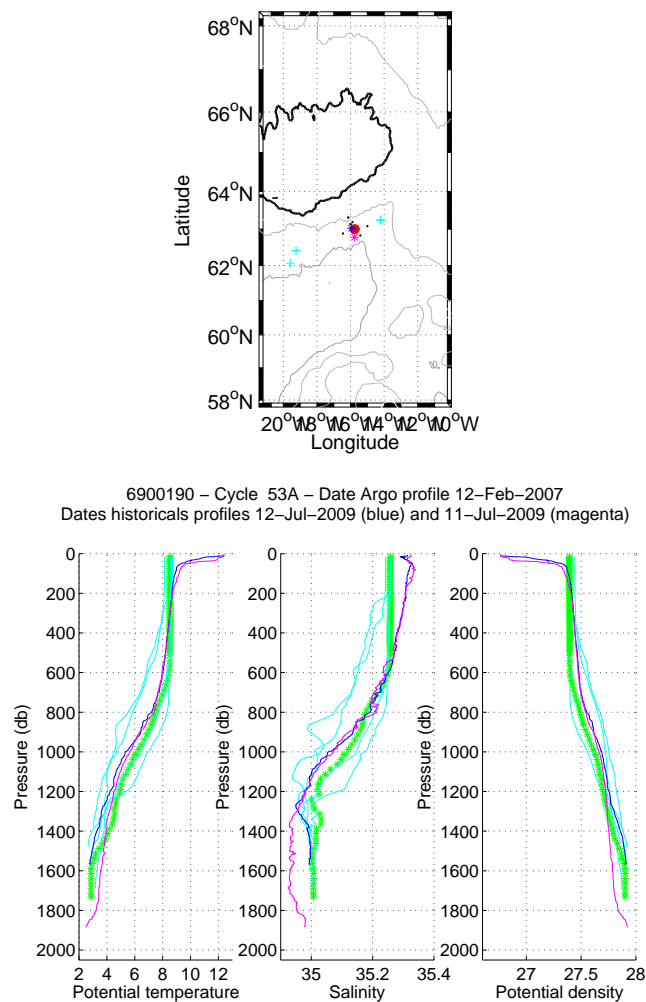
Figure 22: Flotteur 6900190, cycle 53. Upper panel: Position of the analysed CTD profile (red) and of the nearest CTD profiles (black). The nearest CTD profile in time is in magenta while the nearest CTD profile in space is in blue. Lower panels: Temperature, salinity and potential density as function of pressure for the analysed CTD profile (stars) and for the nearest CTD profile in time (magenta line) and for the nearest CTD profile in space (blue line). The color of the analysed CTD profile represents the QC flag (green for a QC=1; blue for a QC=2; orange for a QC=3 and red for a QC=4).
