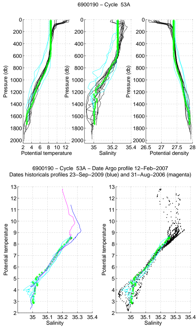
Figure 25: Float 6900190, cycle 53. The analysed Argo profile (stars) is compared to the nearest Argo profiles (black line) and to two specific profiles: the nearest Argo profile in time (magenta) and the nearest Argo profile in space (blue). The color of the analysed Argo profile represents the QC flag (green for a QC=1; blue for a QC=2; orange for a QC=3 and red for a QC=4). (Upper panels) Temperature (left panel), salinity (middle panel) and potential density (right panel) as function of pressure. (Lower panels) \theta/S diagrams.
