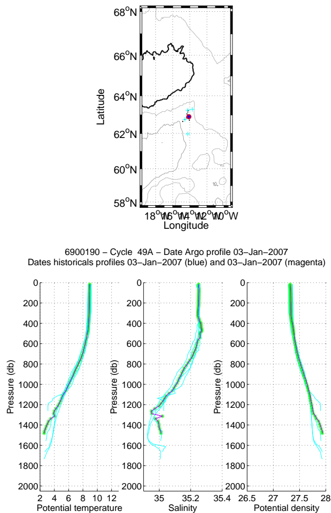
Figure 16: Flotteur 6900190, cycle 49. Upper panel: Position of the analysed Argo profile (red) and of the nearest Argo profiles (black). The nearest Argo profile in time is in magenta while the nearest CTD profile in space is in blue. Lower panels: Temperature, salinity and potential density as function of pressure for the analysed Argo profile (stars) and for the nearest Argo profile in time (magenta line) and for the nearest Argo profile in space (blue line). The color of the analysed Argo profile represents the QC flag (green for a QC=1; blue for a QC=2; orange for a QC=3 and red for a QC=4).
