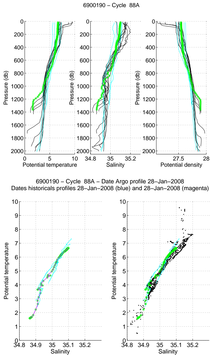
Figure 29: Float 6900190, cycle 88. The analysed Argo profile (stars) is compared to the nearest Argo profiles (black line) and to two specific profiles: the nearest Argo profile in time (magenta) and the nearest Argo profile in space (blue). The color of the analysed Argo profile represents the QC flag (green for a QC=1; blue for a QC=2; orange for a QC=3 and red for a QC=4). (Upper panels) Temperature (left panel), salinity (middle panel) and potential density (right panel) as function of pressure. (Lower panels) \theta/S diagrams.
