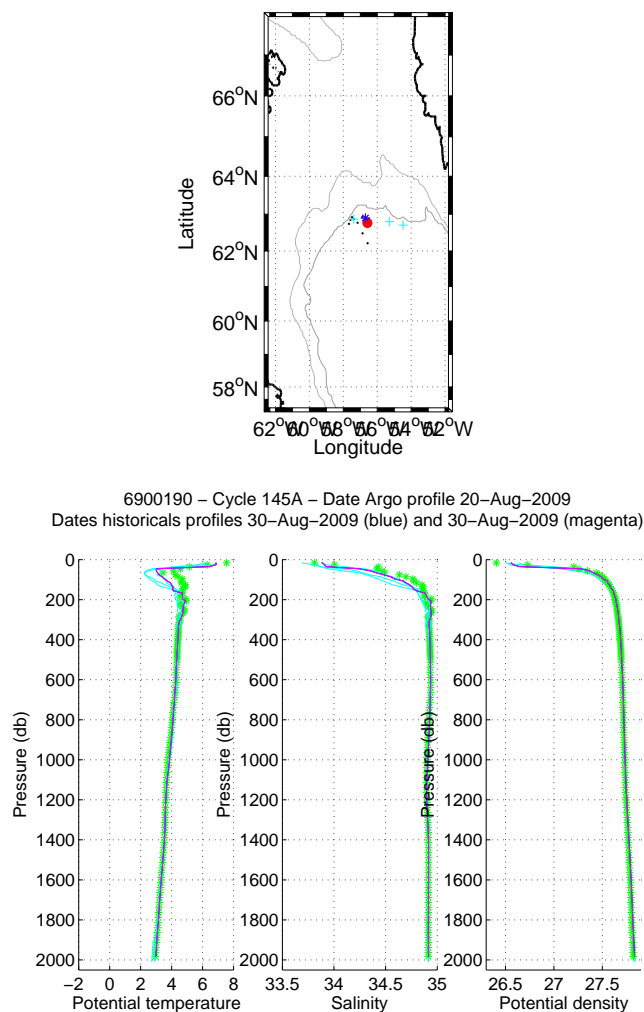
Figure 40: Flotteur 6900190, cycle 145. Upper panel: Position of the analysed Argo profile (red) and of the nearest Argo profiles (black). The nearest Argo profile in time is in magenta while the nearest CTD profile in space is in blue. Lower panels: Temperature, salinity and potential density as function of pressure for the analysed Argo profile (stars) and for the nearest Argo profile in time (magenta line) and for the nearest Argo profile in space (blue line). The color of the analysed Argo profile represents the QC flag (green for a QC=1; blue for a QC=2; orange for a QC=3 and red for a QC=4).
