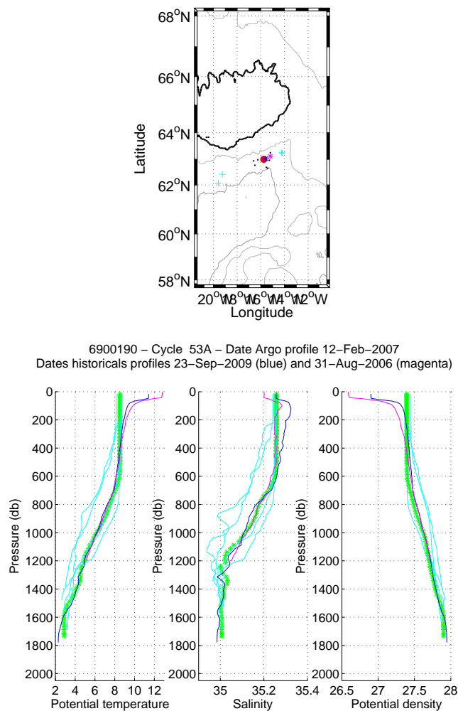
Figure 24: Flotteur 6900190, cycle 53. Upper panel: Position of the analysed Argo profile (red) and of the nearest Argo profiles (black). The nearest Argo profile in time is in magenta while the nearest CTD profile in space is in blue. Lower panels: Temperature, salinity and potential density as function of pressure for the analysed Argo profile (stars) and for the nearest Argo profile in time (magenta line) and for the nearest Argo profile in space (blue line). The color of the analysed Argo profile represents the QC flag (green for a QC=1; blue for a QC=2; orange for a QC=3 and red for a QC=4).
