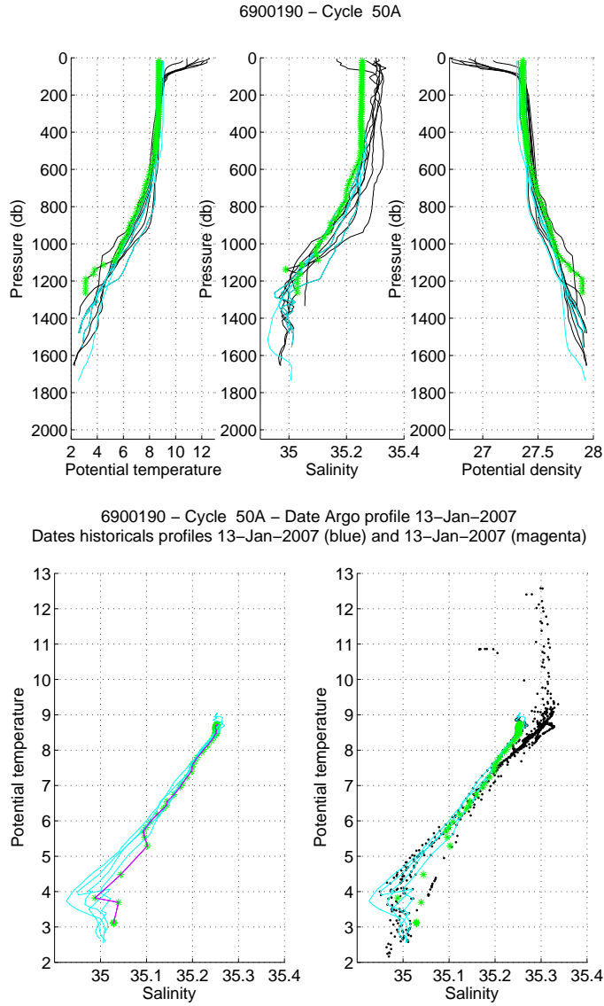
Figure 21: Float 6900190, cycle 50. The analysed Argo profile (stars) is compared to the nearest Argo profiles (black line) and to two specific profiles: the nearest Argo profile in time (magenta) and the nearest Argo profile in space (blue). The color of the analysed Argo profile represents the QC flag (green for a QC=1; blue for a QC=2; orange for a QC=3 and red for a QC=4). (Upper panels) Temperature (left panel), salinity (middle panel) and potential density (right panel) as function of pressure. (Lower panels) \theta/S diagrams.
