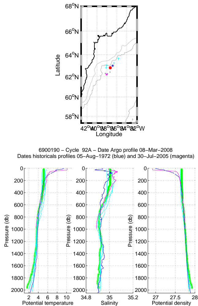
Figure 30: Flotteur 6900190, cycle 92. Upper panel: Position of the analysed CTD profile (red) and of the nearest CTD profiles (black). The nearest CTD profile in time is in magenta while the nearest CTD profile in space is in blue. Lower panels: Temperature, salinity and potential density as function of pressure for the analysed CTD profile (stars) and for the nearest CTD profile in time (magenta line) and for the nearest CTD profile in space (blue line). The color of the analysed CTD profile represents the QC flag (green for a QC=1; blue for a QC=2; orange for a QC=3 and red for a QC=4).
