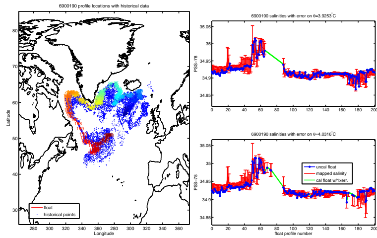
Figure 46: Figures from the OW method. (Left) Position of the historical and float data. (Right) Comparison, on various \theta levels, between the float data and the historical data interpolated at the float position.
