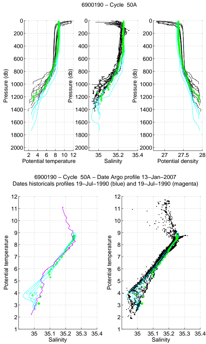
Figure 19: Float 6900190, cycle 50. The analysed CTD profile (stars) is compared to the nearest CTD profiles (black line) and to two specific profiles: the nearest CTD profile in time (magenta) and the nearest CTD profile in space (blue). The color of the analysed CTD profile represents the QC flag (green for a QC=1; blue for a QC=2; orange for a QC=3 and red for a QC=4). (Upper panels) Temperature (left panel), salinity (middle panel) and potential density (right panel) as function of pressure. (Lower panels) \theta/S diagrams.
