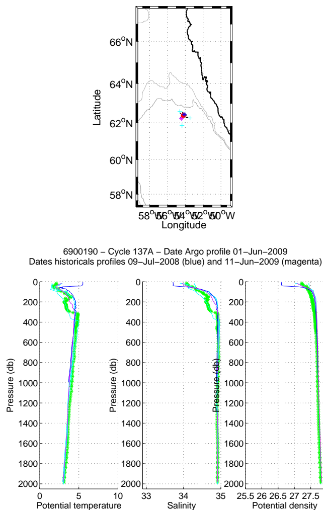
Figure 36: Flotteur 6900190, cycle 137A. Upper panel: Position of the analysed Argo profile (red) and of the nearest Argo profiles (black). The nearest Argo profile in time is in magenta while the nearest CTD profile in space is in blue. Lower panels: Temperature, salinity and potential density as function of pressure for the analysed Argo profile (stars) and for the nearest Argo profile in time (magenta line) and for the nearest Argo profile in space (blue line). The color of the analysed Argo profile represents the QC flag (green for a QC=1; blue for a QC=2; orange for a QC=3 and red for a QC=4).
