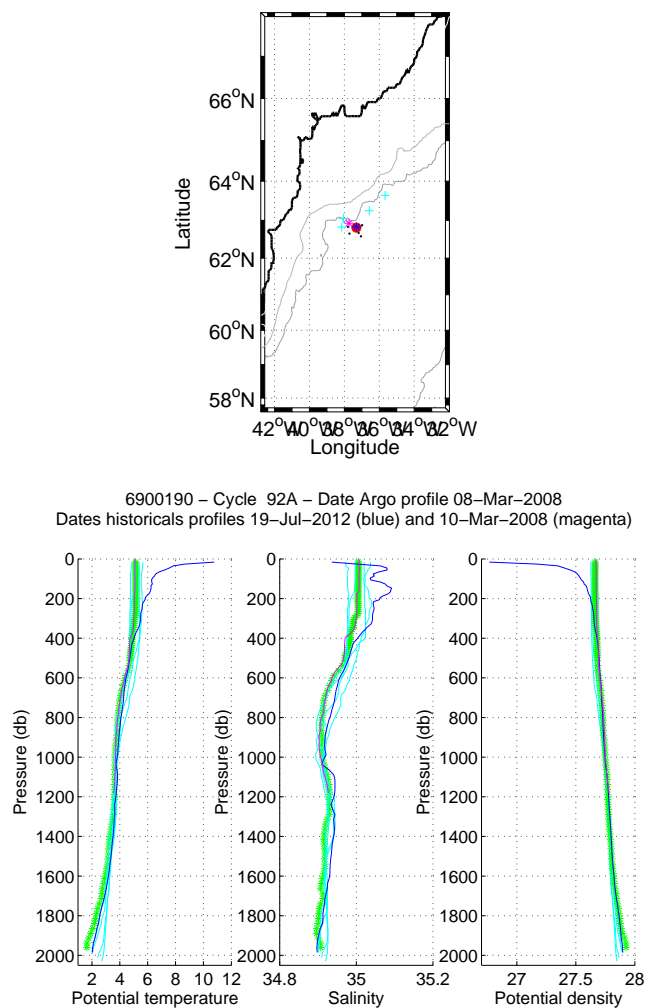
Figure 32: Flotteur 6900190, cycle 92. Upper panel: Position of the analysed Argo profile (red) and of the nearest Argo profiles (black). The nearest Argo profile in time is in magenta while the nearest CTD profile in space is in blue. Lower panels: Temperature, salinity and potential density as function of pressure for the analysed Argo profile (stars) and for the nearest Argo profile in time (magenta line) and for the nearest Argo profile in space (blue line). The color of the analysed Argo profile represents the QC flag (green for a QC=1; blue for a QC=2; orange for a QC=3 and red for a QC=4).
