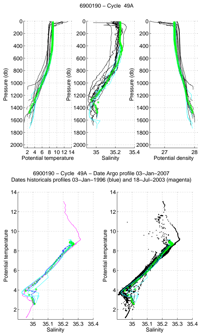
Figure 15: Float 6900190, cycle 49. The analysed CTD profile (stars) is compared to the nearest CTD profiles (black line) and to two specific profiles: the nearest CTD profile in time (magenta) and the nearest CTD profile in space (blue). The color of the analysed CTD profile represents the QC flag (green for a QC=1; blue for a QC=2; orange for a QC=3 and red for a QC=4). (Upper panels) Temperature (left panel), salinity (middle panel) and potential density (right panel) as function of pressure. (Lower panels) \theta/S diagrams.
