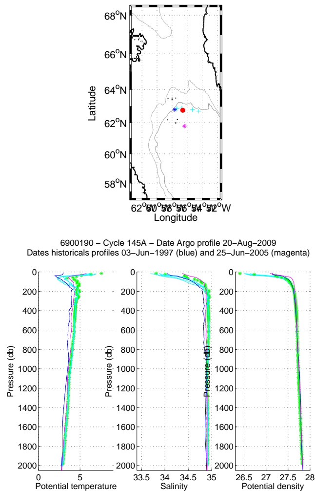
Figure 38: Flotteur 6900190, cycle 145. Upper panel: Position of the analysed CTD profile (red) and of the nearest CTD profiles (black). The nearest CTD profile in time is in magenta while the nearest CTD profile in space is in blue. Lower panels: Temperature, salinity and potential density as function of pressure for the analysed CTD profile (stars) and for the nearest CTD profile in time (magenta line) and for the nearest CTD profile in space (blue line). The color of the analysed CTD profile represents the QC flag (green for a QC=1; blue for a QC=2; orange for a QC=3 and red for a QC=4).
