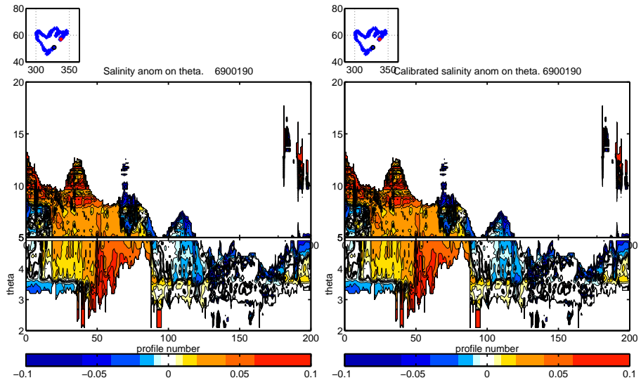
Figure 48: Figures from the OW method. Salinity anomaly:(left) raw data; (right) corrected data using the OW correction.
