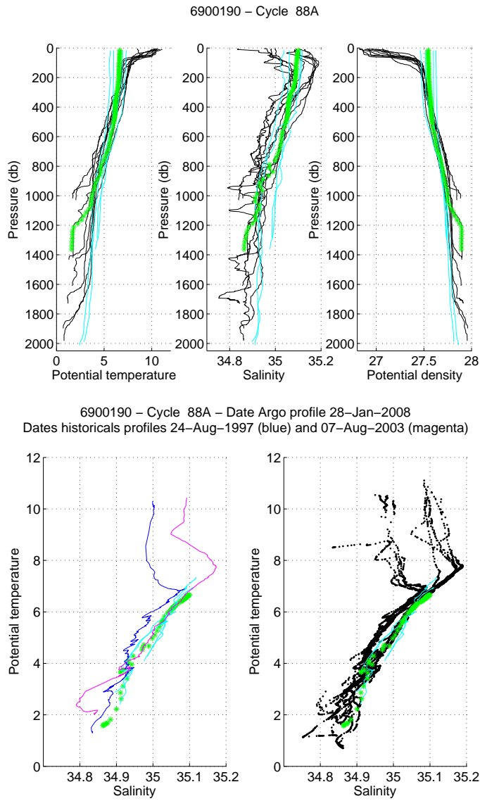
Figure 27: Float 6900190, cycle 88. The analysed CTD profile (stars) is compared to the nearest CTD profiles (black line) and to two specific profiles: the nearest CTD profile in time (magenta) and the nearest CTD profile in space (blue). The color of the analysed CTD profile represents the QC flag (green for a QC=1; blue for a QC=2; orange for a QC=3 and red for a QC=4). (Upper panels) Temperature (left panel), salinity (middle panel) and potential density (right panel) as function of pressure. (Lower panels) \theta/S diagrams.
