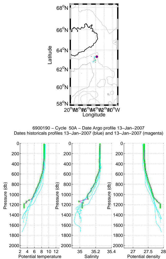
Figure 20: Flotteur 6900190, cycle 50. Upper panel: Position of the analysed Argo profile (red) and of the nearest Argo profiles (black). The nearest Argo profile in time is in magenta while the nearest CTD profile in space is in blue. Lower panels: Temperature, salinity and potential density as function of pressure for the analysed Argo profile (stars) and for the nearest Argo profile in time (magenta line) and for the nearest Argo profile in space (blue line). The color of the analysed Argo profile represents the QC flag (green for a QC=1; blue for a QC=2; orange for a QC=3 and red for a QC=4).
