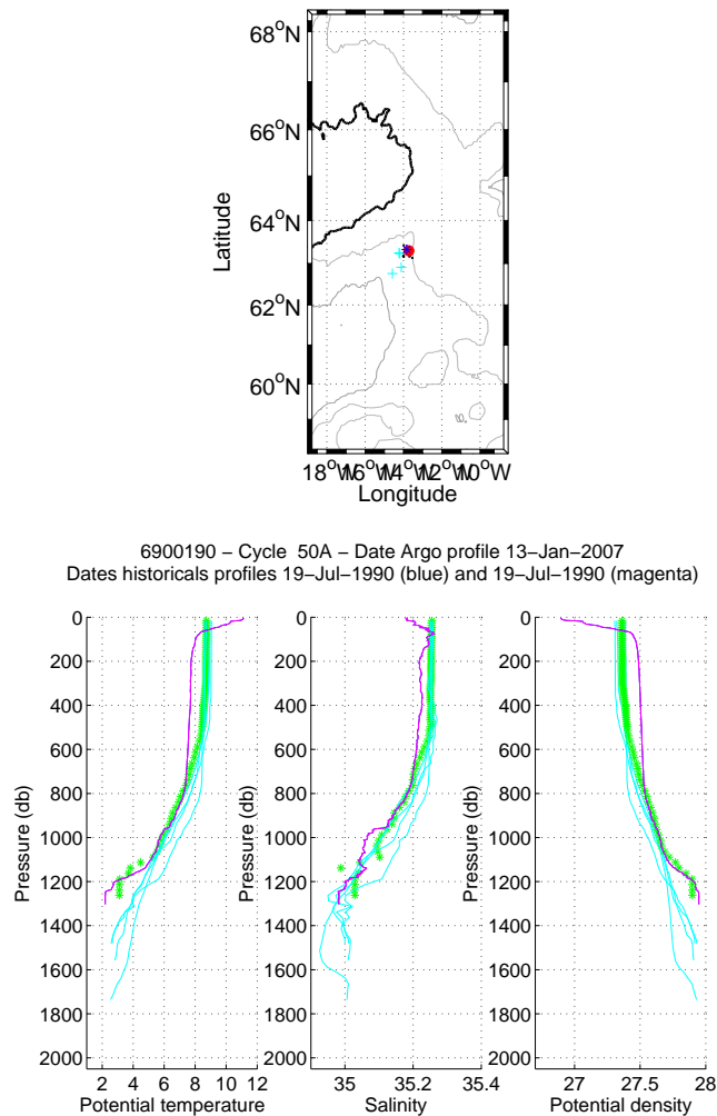
Figure 18: Flotteur 6900190, cycle 50. Upper panel: Position of the analysed CTD profile (red) and of the nearest CTD profiles (black). The nearest CTD profile in time is in magenta while the nearest CTD profile in space is in blue. Lower panels: Temperature, salinity and potential density as function of pressure for the analysed CTD profile (stars) and for the nearest CTD profile in time (magenta line) and for the nearest CTD profile in space (blue line). The color of the analysed CTD profile represents the QC flag (green for a QC=1; blue for a QC=2; orange for a QC=3 and red for a QC=4).
