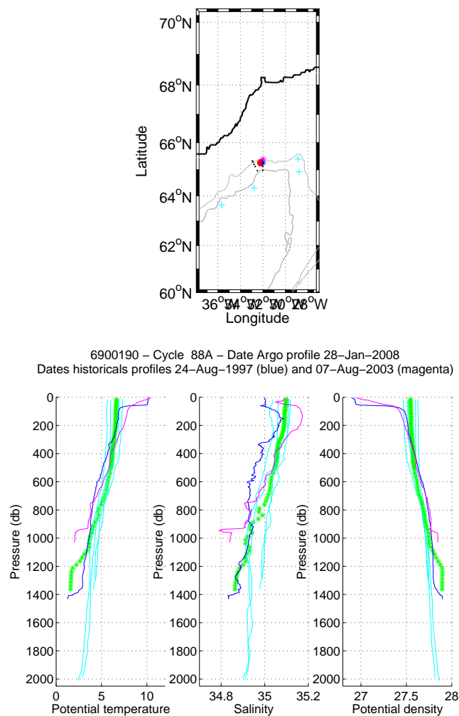
Figure 26: Flotteur 6900190, cycle 88. Upper panel: Position of the analysed CTD profile (red) and of the nearest CTD profiles (black). The nearest CTD profile in time is in magenta while the nearest CTD profile in space is in blue. Lower panels: Temperature, salinity and potential density as function of pressure for the analysed CTD profile (stars) and for the nearest CTD profile in time (magenta line) and for the nearest CTD profile in space (blue line). The color of the analysed CTD profile represents the QC flag (green for a QC=1; blue for a QC=2; orange for a QC=3 and red for a QC=4).
