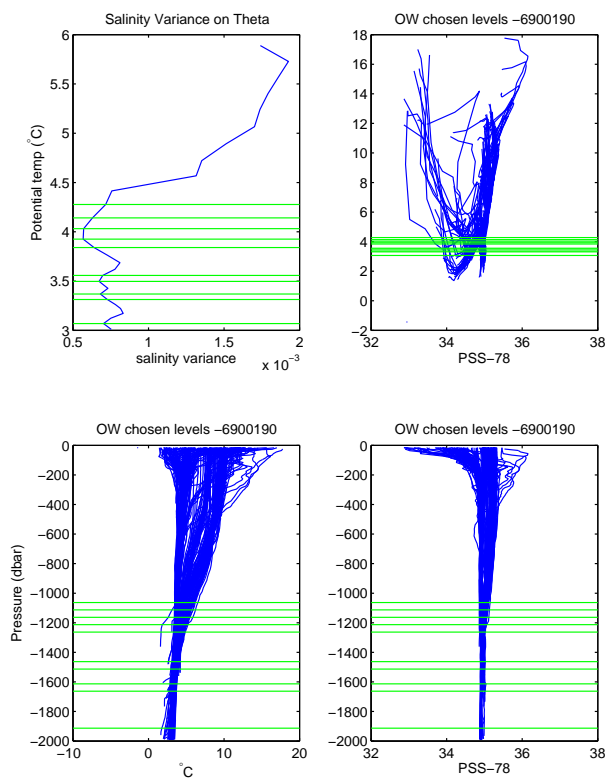
Figure 50: Chosed levels by the OW method.
