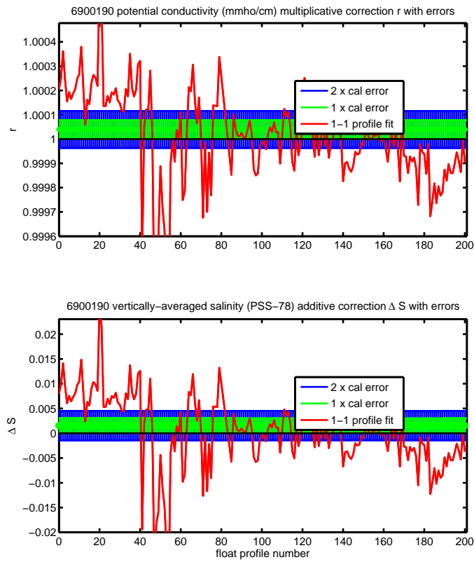
Figure 49: Correction proposed by the OW method.
