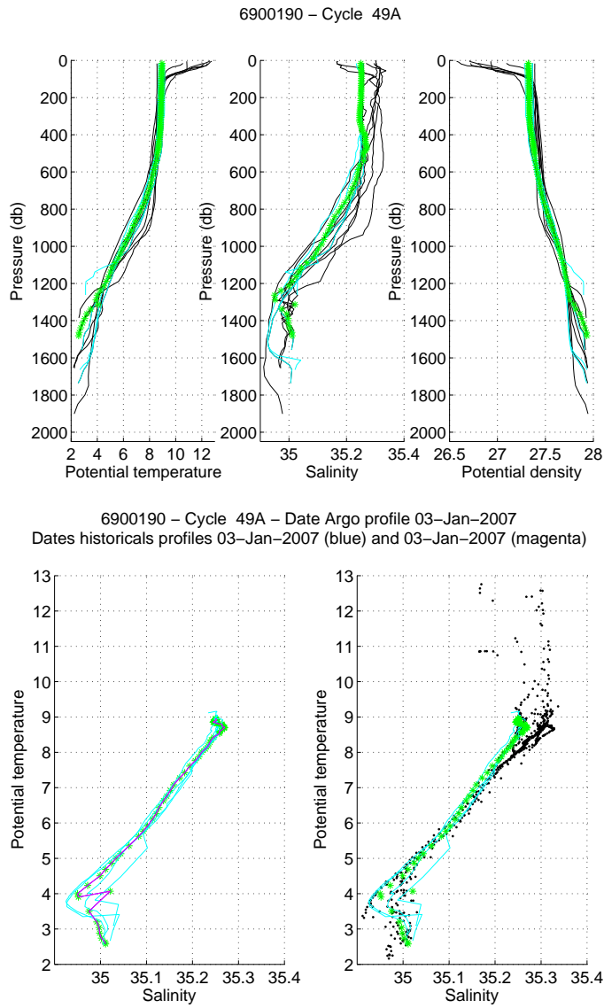
Figure 17: Float 6900190, cycle 49. The analysed Argo profile (stars) is compared to the nearest Argo profiles (black line) and to two specific profiles: the nearest Argo profile in time (magenta) and the nearest Argo profile in space (blue). The color of the analysed Argo profile represents the QC flag (green for a QC=1; blue for a QC=2; orange for a QC=3 and red for a QC=4). (Upper panels) Temperature (left panel), salinity (middle panel) and potential density (right panel) as function of pressure. (Lower panels) \theta/S diagrams.
