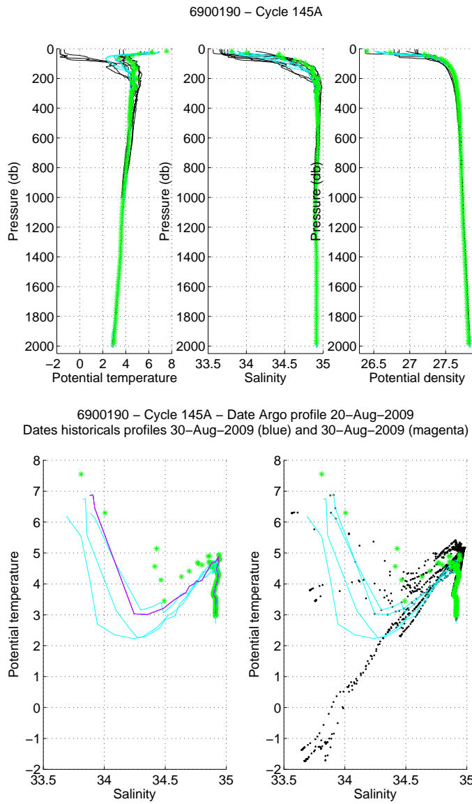
Figure 41: Float 6900190, cycle 145. The analysed Argo profile (stars) is compared to the nearest Argo profiles (black line) and to two specific profiles: the nearest Argo profile in time (magenta) and the nearest Argo profile in space (blue). The color of the analysed Argo profile represents the QC flag (green for a QC=1; blue for a QC=2; orange for a QC=3 and red for a QC=4). (Upper panels) Temperature (left panel), salinity (middle panel) and potential density (right panel) as function of pressure. (Lower panels) \theta/S diagrams.
