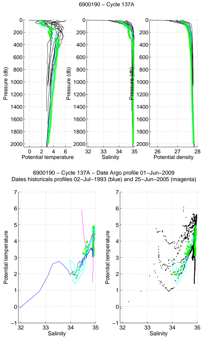
Figure 35: Float 6900190, cycle 137. The analysed CTD profile (stars) is compared to the nearest CTD profiles (black line) and to two specific profiles: the nearest CTD profile in time (magenta) and the nearest CTD profile in space (blue). The color of the analysed CTD profile represents the QC flag (green for a QC=1; blue for a QC=2; orange for a QC=3 and red for a QC=4). (Upper panels) Temperature (left panel), salinity (middle panel) and potential density (right panel) as function of pressure. (Lower panels) \theta/S diagrams.
