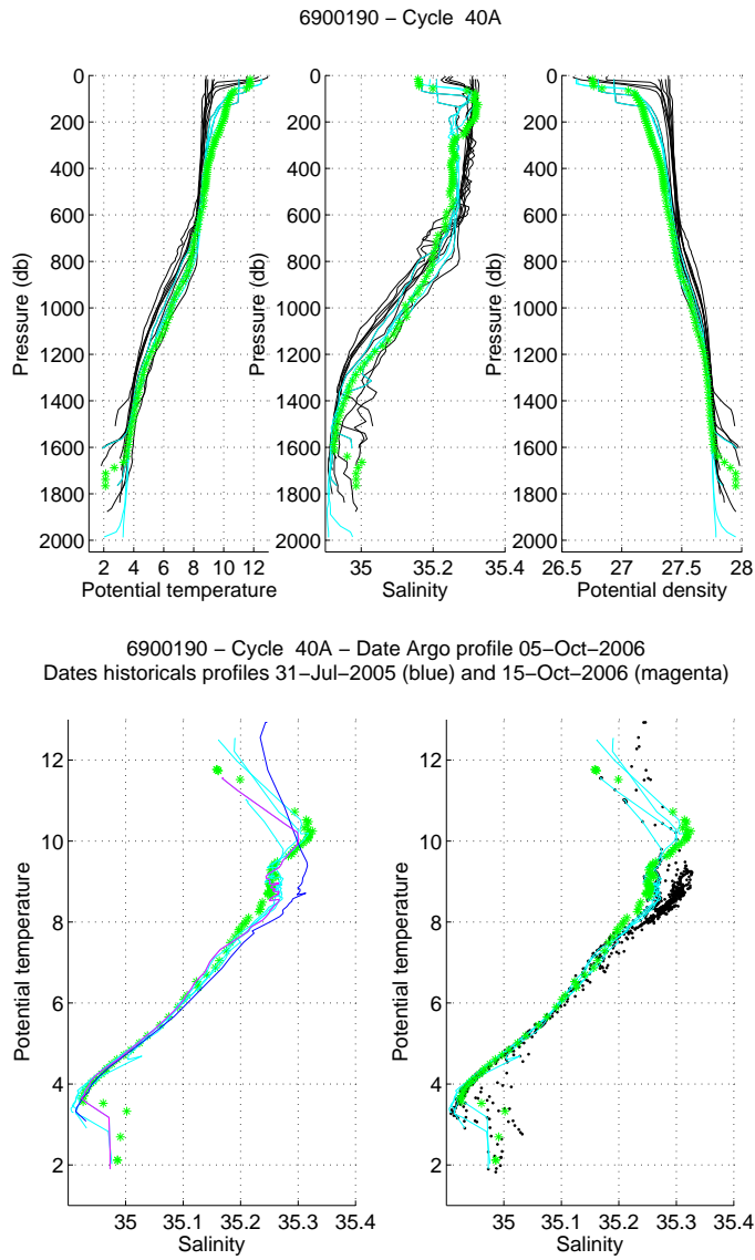
Figure 13: Float 6900190, cycle 40. The analysed Argo profile (stars) is compared to the nearest Argo profiles (black line) and to two specific profiles: the nearest Argo profile in time (magenta) and the nearest Argo profile in space (blue). The color of the analysed Argo profile represents the QC flag (green for a QC=1; blue for a QC=2; orange for a QC=3 and red for a QC=4). (Upper panels) Temperature (left panel), salinity (middle panel) and potential density (right panel) as function of pressure. (Lower panels) \theta/S diagrams.
