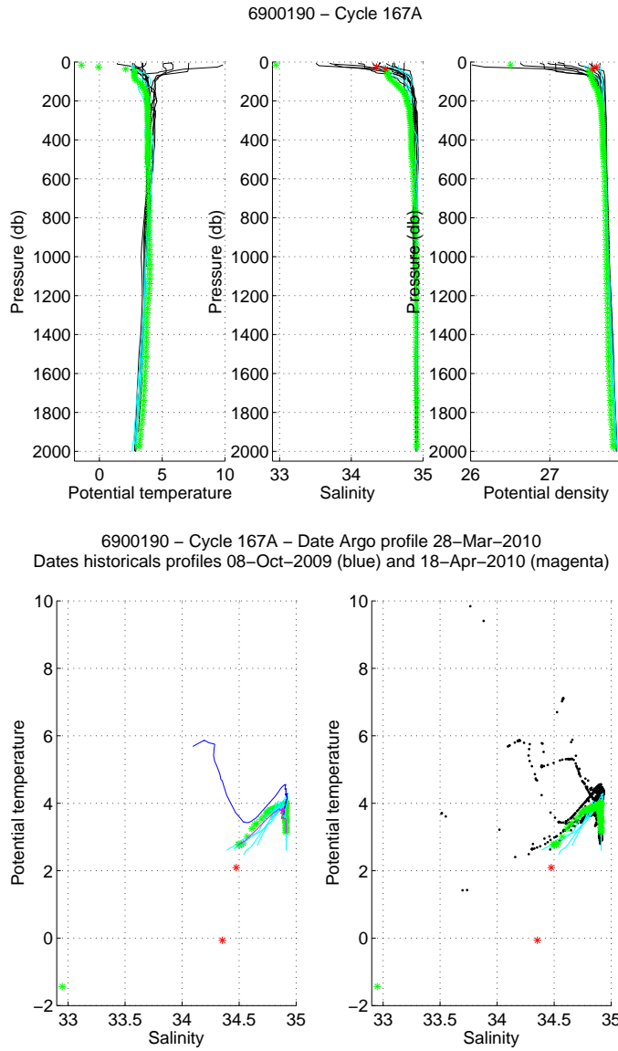
Figure 45: Float 6900190, cycle 167. The analysed Argo profile (stars) is compared to the nearest Argo profiles (black line) and to two specific profiles: the nearest Argo profile in time (magenta) and the nearest Argo profile in space (blue). The color of the analysed Argo profile represents the QC flag (green for a QC=1; blue for a QC=2; orange for a QC=3 and red for a QC=4). (Upper panels) Temperature (left panel), salinity (middle panel) and potential density (right panel) as function of pressure. (Lower panels) \theta/S diagrams.
