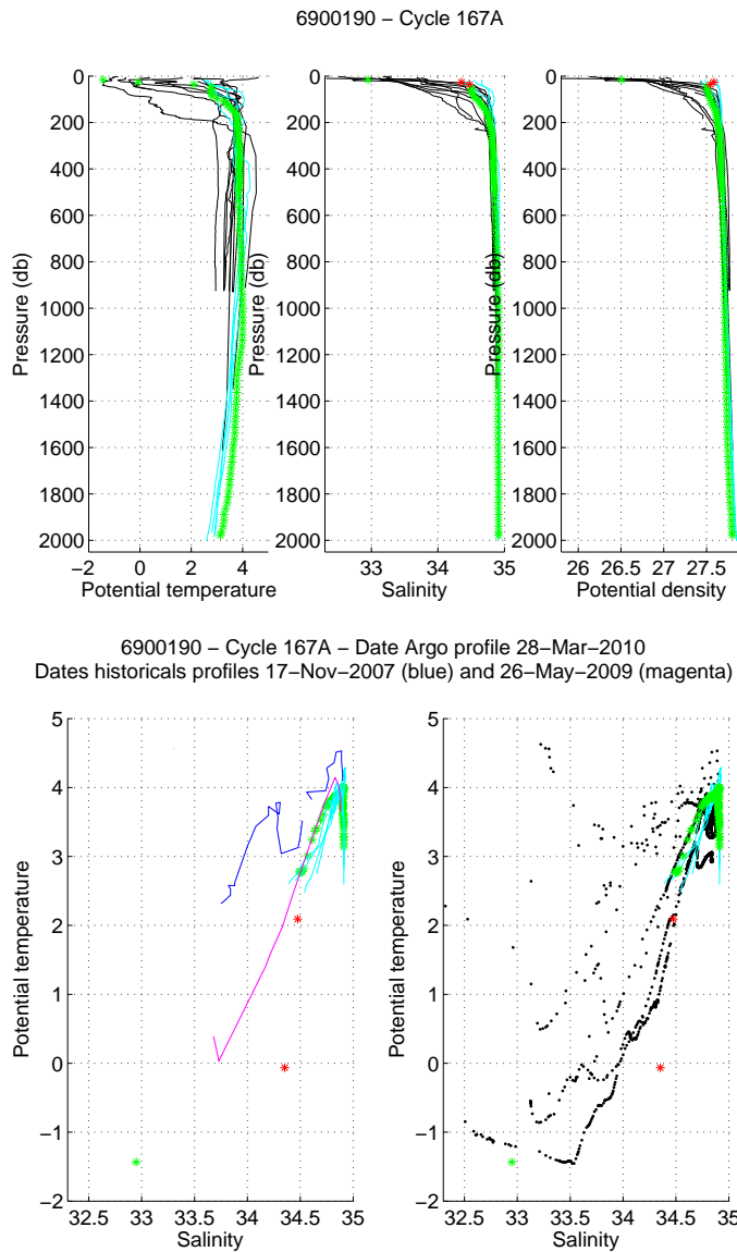
Figure 43: Float 6900190, cycle 167. The analysed CTD profile (stars) is compared to the nearest CTD profiles (black line) and to two specific profiles: the nearest CTD profile in time (magenta) and the nearest CTD profile in space (blue). The color of the analysed CTD profile represents the QC flag (green for a QC=1; blue for a QC=2; orange for a QC=3 and red for a QC=4). (Upper panels) Temperature (left panel), salinity (middle panel) and potential density (right panel) as function of pressure. (Lower panels) \theta/S diagrams.
