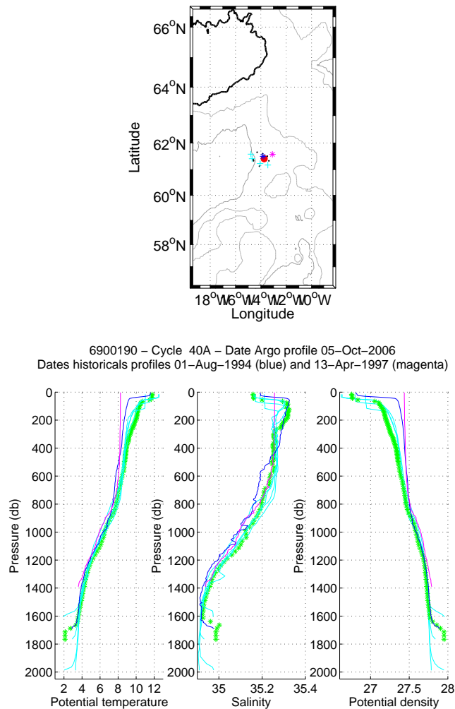
Figure 10: Flotteur 6900190, cycle 40. Upper panel: Position of the analysed CTD profile (red) and of the nearest CTD profiles (black). The nearest CTD profile in time is in magenta while the nearest CTD profile in space is in blue. Lower panels: Temperature, salinity and potential density as function of pressure for the analysed CTD profile (stars) and for the nearest CTD profile in time (magenta line) and for the nearest CTD profile in space (blue line). The color of the analysed CTD profile represents the QC flag (green for a QC=1; blue for a QC=2; orange for a QC=3 and red for a QC=4).
