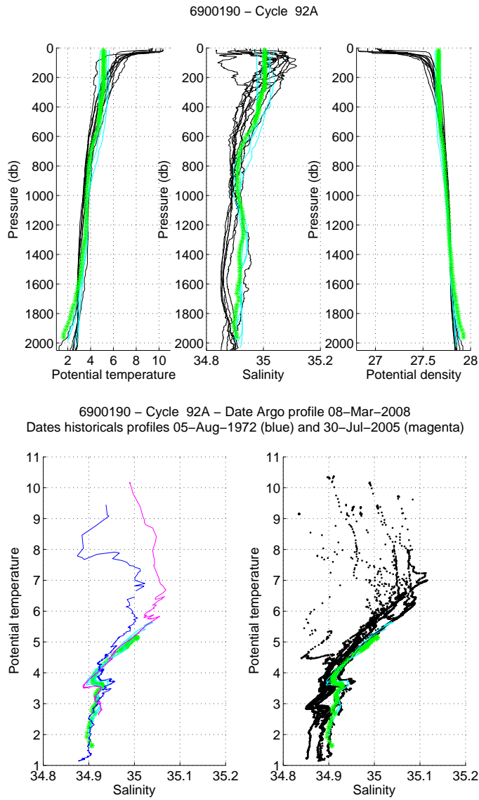
Figure 31: Float 6900190, cycle 92. The analysed CTD profile (stars) is compared to the nearest CTD profiles (black line) and to two specific profiles: the nearest CTD profile in time (magenta) and the nearest CTD profile in space (blue). The color of the analysed CTD profile represents the QC flag (green for a QC=1; blue for a QC=2; orange for a QC=3 and red for a QC=4). (Upper panels) Temperature (left panel), salinity (middle panel) and potential density (right panel) as function of pressure. (Lower panels) \theta/S diagrams.
