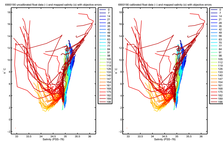
Figure 47: Figures from the OW method. Comparison of the \theta/S diagram of the float with the historical database. (left) raw data; (right) corrected data using the OW correction.
