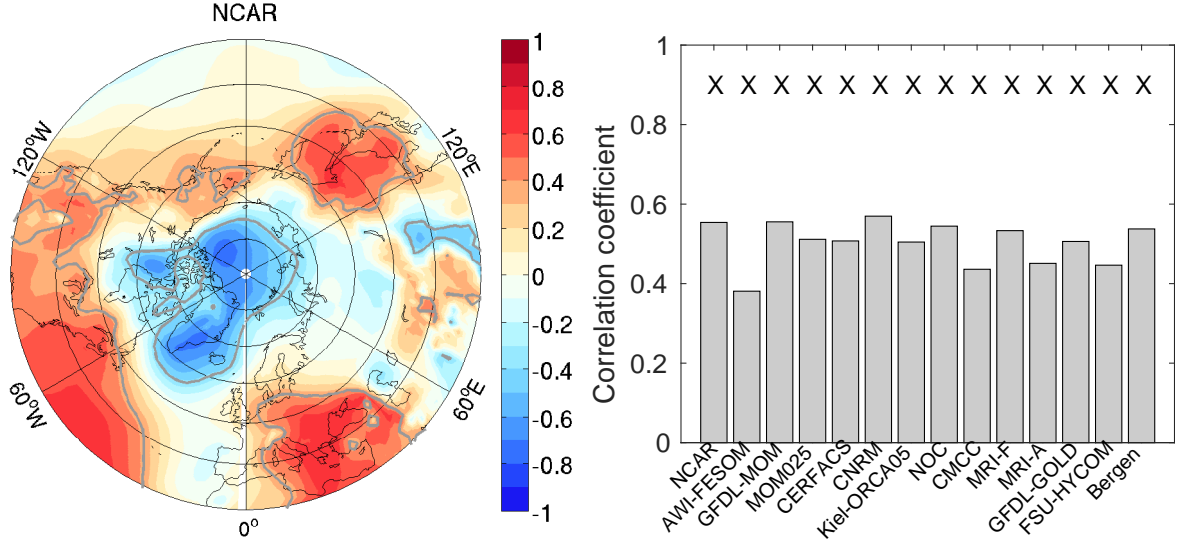
(a) Correlation of DS transport with SLP
