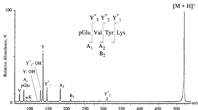
FIG. 3. Daughter ions observed by nanoES-MS-MS of the molecular ion ( m/z = 520 ) of the \text{NH}_2 -terminally blocked tryptic peptide of the penaeidin-3. The fragmentation data shown here, combined with other mass-spectral data (Table I), allowed deduction of the pGlu-Val-Tyr-Lys sequence.
