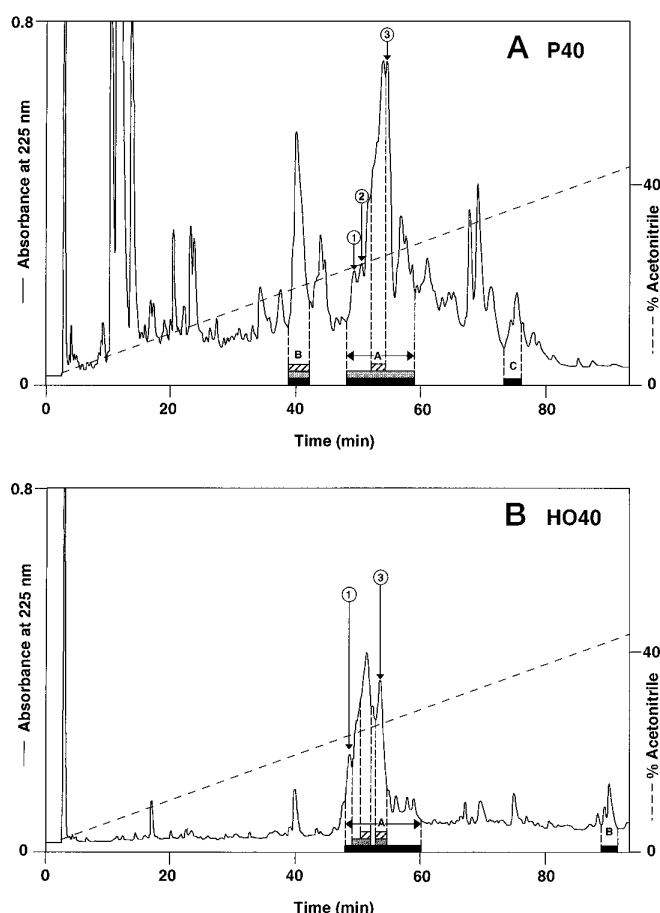
FIG. 1. Reversed-phase HPLC of two acidic extracts obtained from plasma (A) and hemocytes (B) of experimentally uninfected P. vannamei . The fractions eluted with 40% acetonitrile in acidified water from Sep-Pak C 18 cartridges (P40 and HO40) were analyzed on an Aquapore RP300 C 8 column using a 2–60% linear gradient (dashed line) of acidified acetonitrile over 80 min (0.72% acetonitrile/min) at a flow rate of 1 ml/min. Absorbance was monitored at 225 nm (solid line). Antimicrobial activity against E. coli D31 (hatched rectangles), M. luteus (black shaded rectangles), and N. crassa (gray shaded rectangles) was measured by liquid growth inhibition assays. The regions displaying antimicrobial activity are indicated by letters (A, B, and C). Fractions containing the peptides characterized in this study are indicated by arrows (1, 2, and 3).
