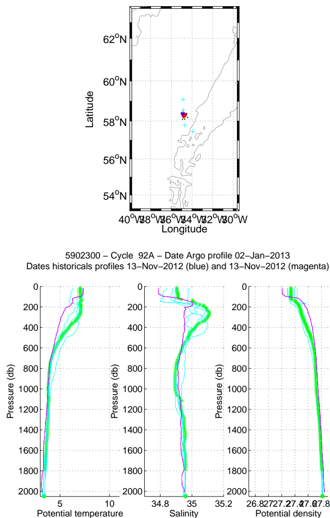
Figure 18: Flotteur 5902300, cycle 92A. Upper panel: Position of the analysed Argo profile (red) and of the nearest Argo profiles (black). The nearest Argo profile in time is in magenta while the nearest CTD profile in space is in blue. Lower panels: Temperature, salinity and potential density as function of pressure for the analysed Argo profile (stars) and for the nearest Argo profile in time (magenta line) and for the nearest Argo profile in space (blue line). The color of the analysed Argo profile represents the QC flag (green for a QC=1; blue for a QC=2; orange for a QC=3 and red for a QC=4).
