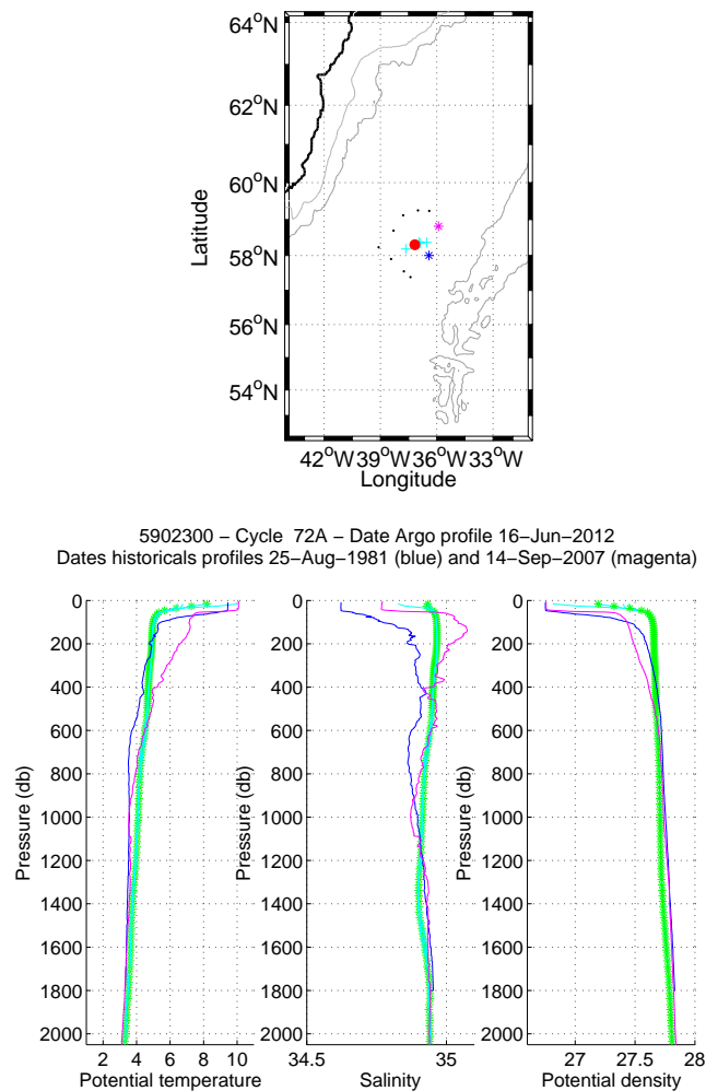
Figure 12: Flotteur 5902300, cycle 72. Upper panel: Position of the analysed CTD profile (red) and of the nearest CTD profiles (black). The nearest CTD profile in time is in magenta while the nearest CTD profile in space is in blue. Lower panels: Temperature, salinity and potential density as function of pressure for the analysed CTD profile (stars) and for the nearest CTD profile in time (magenta line) and for the nearest CTD profile in space (blue line). The color of the analysed CTD profile represents the QC flag (green for a QC=1; blue for a QC=2; orange for a QC=3 and red for a QC=4).
