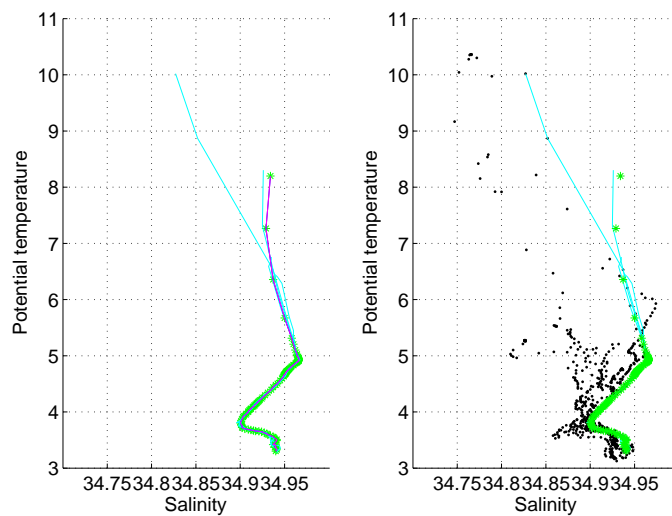
Figure 15: Float 5902300, cycle 72A. The analysed Argo profile (stars) is compared to the nearest Argo profiles (black line) and to two specific profiles: the nearest Argo profile in time (magenta) and the nearest Argo profile in space (blue). The color of the analysed Argo profile represents the QC flag (green for a QC=1; blue for a QC=2; orange for a QC=3 and red for a QC=4). (Upper panels) Temperature (left panel), salinity (middle panel) and potential density (right panel) as function of pressure. (Lower panels) \theta/S diagrams.
