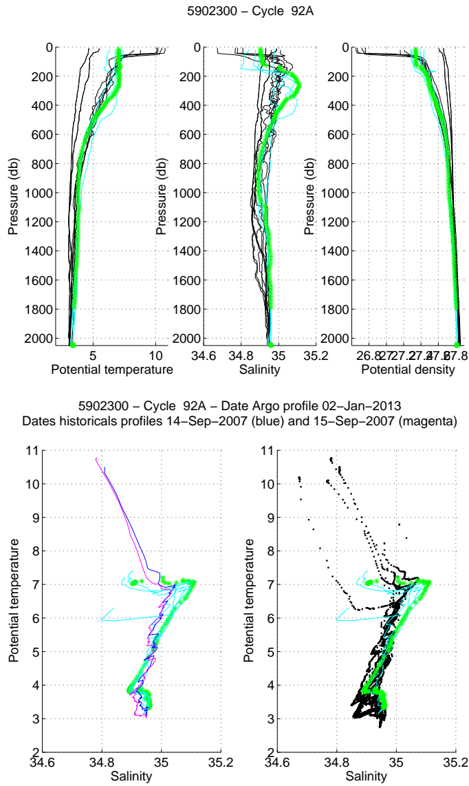
Figure 17: Float 5902300, cycle 92. The analysed CTD profile (stars) is compared to the nearest CTD profiles (black line) and to two specific profiles: the nearest CTD profile in time (magenta) and the nearest CTD profile in space (blue). The color of the analysed CTD profile represents the QC flag (green for a QC=1; blue for a QC=2; orange for a QC=3 and red for a QC=4). (Upper panels) Temperature (left panel), salinity (middle panel) and potential density (right panel) as function of pressure. (Lower panels) \theta/S diagrams.
