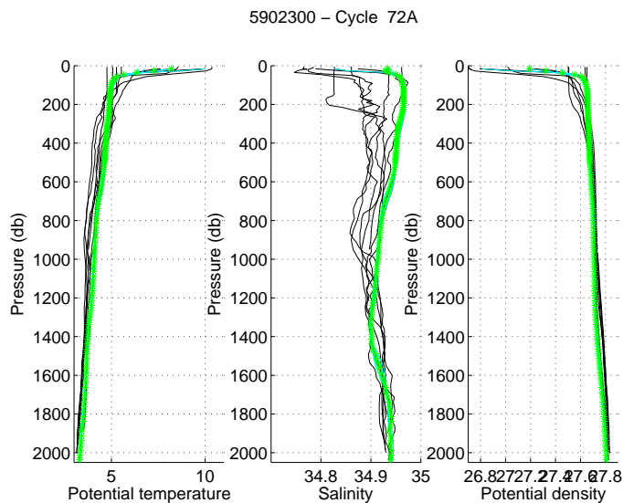
5902300 – Cycle 72A – Date Argo profile 16-Jun-2012 Dates historical profiles 16-Jun-2012 (blue) and 16-Jun-2012 (magenta)
