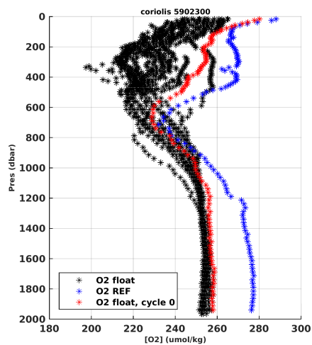
Figure 5: Profiles float 5902300 (black), O2 hydro reference (blue), O2 float cycle 0 (red)
