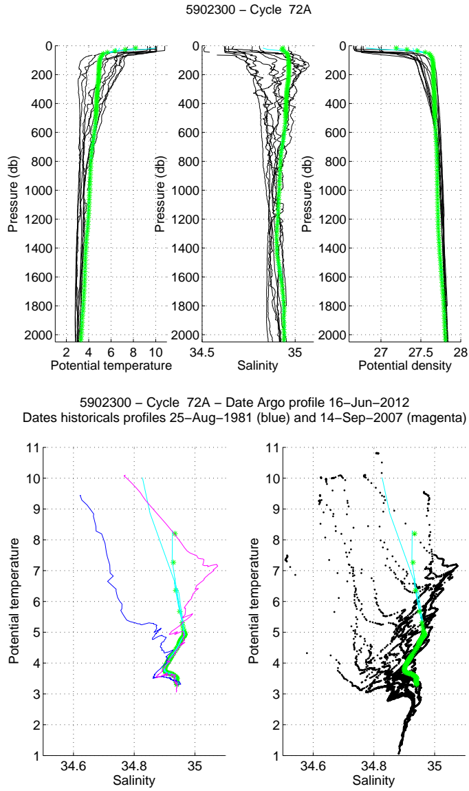
Figure 13: Float 5902300, cycle 72. The analysed CTD profile (stars) is compared to the nearest CTD profiles (black line) and to two specific profiles: the nearest CTD profile in time (magenta) and the nearest CTD profile in space (blue). The color of the analysed CTD profile represents the QC flag (green for a QC=1; blue for a QC=2; orange for a QC=3 and red for a QC=4). (Upper panels) Temperature (left panel), salinity (middle panel) and potential density (right panel) as function of pressure. (Lower panels) \theta/S diagrams.
