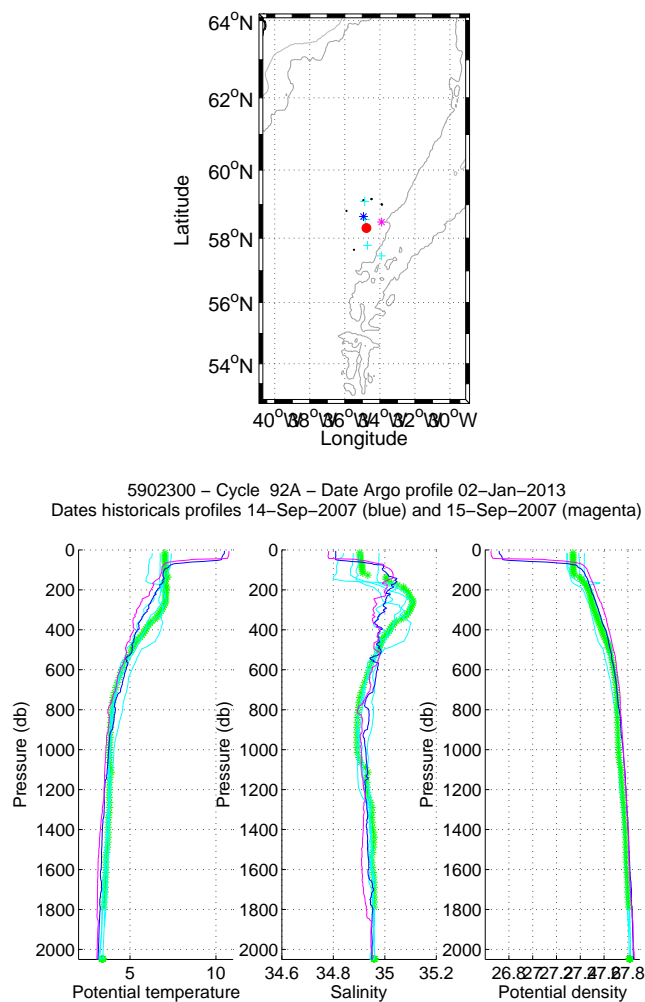
Figure 16: Flotteur 5902300, cycle 92. Upper panel: Position of the analysed CTD profile (red) and of the nearest CTD profiles (black). The nearest CTD profile in time is in magenta while the nearest CTD profile in space is in blue. Lower panels: Temperature, salinity and potential density as function of pressure for the analysed CTD profile (stars) and for the nearest CTD profile in time (magenta line) and for the nearest CTD profile in space (blue line). The color of the analysed CTD profile represents the QC flag (green for a QC=1; blue for a QC=2; orange for a QC=3 and red for a QC=4).
