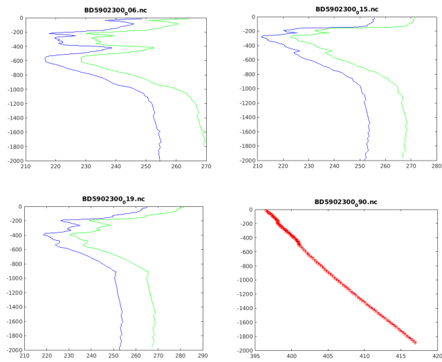
Figure 9: Float 5902300 : Corrected profiles in green
