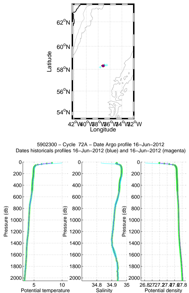
Figure 14: Flotteur 5902300, cycle 72A. Upper panel: Position of the analysed Argo profile (red) and of the nearest Argo profiles (black). The nearest Argo profile in time is in magenta while the nearest CTD profile in space is in blue. Lower panels: Temperature, salinity and potential density as function of pressure for the analysed Argo profile (stars) and for the nearest Argo profile in time (magenta line) and for the nearest Argo profile in space (blue line). The color of the analysed Argo profile represents the QC flag (green for a QC=1; blue for a QC=2; orange for a QC=3 and red for a QC=4).
