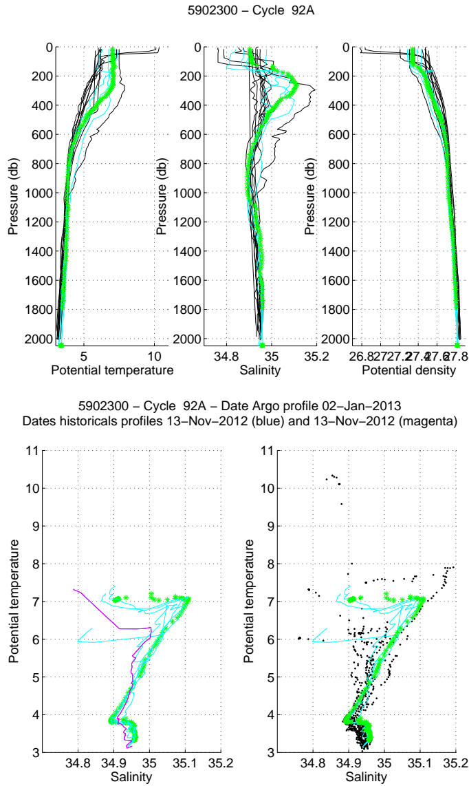
Figure 19: Float 5902300, cycle 92A. The analysed Argo profile (stars) is compared to the nearest Argo profiles (black line) and to two specific profiles: the nearest Argo profile in time (magenta) and the nearest Argo profile in space (blue). The color of the analysed Argo profile represents the QC flag (green for a QC=1; blue for a QC=2; orange for a QC=3 and red for a QC=4). (Upper panels) Temperature (left panel), salinity (middle panel) and potential density (right panel) as function of pressure. (Lower panels) \theta/S diagrams.
