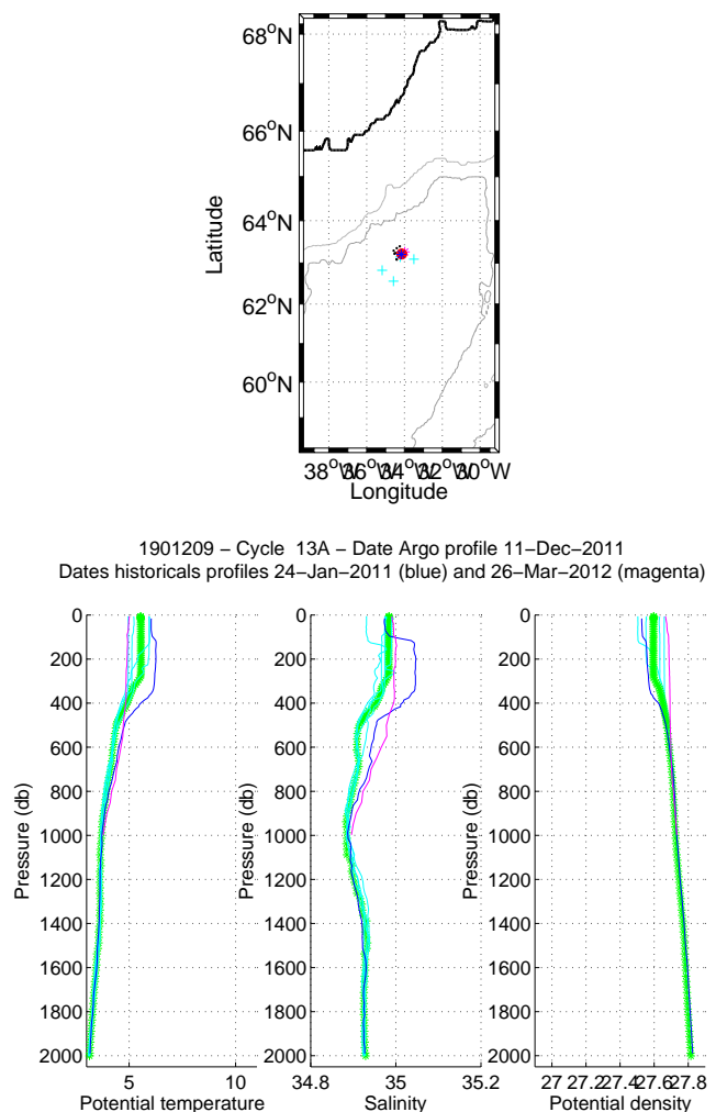
Figure 14: Flotteur 1901209, cycle 13A. Upper panel: Position of the analysed Argo profile (red) and of the nearest Argo profiles (black). The nearest Argo profile in time is in magenta while the nearest CTD profile in space is in blue. Lower panels: Temperature, salinity and potential density as function of pressure for the analysed Argo profile (stars) and for the nearest Argo profile in time (magenta line) and for the nearest Argo profile in space (blue line). The color of the analysed Argo profile represents the QC flag (green for a QC=1; blue for a QC=2; orange for a QC=3 and red for a QC=4).
