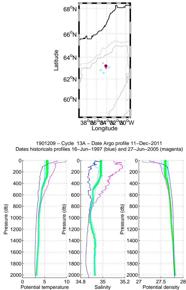
Figure 12: Flotteur 1901209, cycle 13. Upper panel: Position of the analysed CTD profile (red) and of the nearest CTD profiles (black). The nearest CTD profile in time is in magenta while the nearest CTD profile in space is in blue. Lower panels: Temperature, salinity and potential density as function of pressure for the analysed CTD profile (stars) and for the nearest CTD profile in time (magenta line) and for the nearest CTD profile in space (blue line). The color of the analysed CTD profile represents the QC flag (green for a QC=1; blue for a QC=2; orange for a QC=3 and red for a QC=4).
