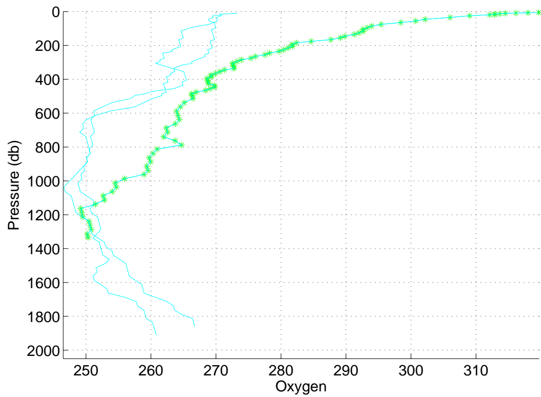
Figure 21: Float 1901209, cycle 24A. Oxygen data.
