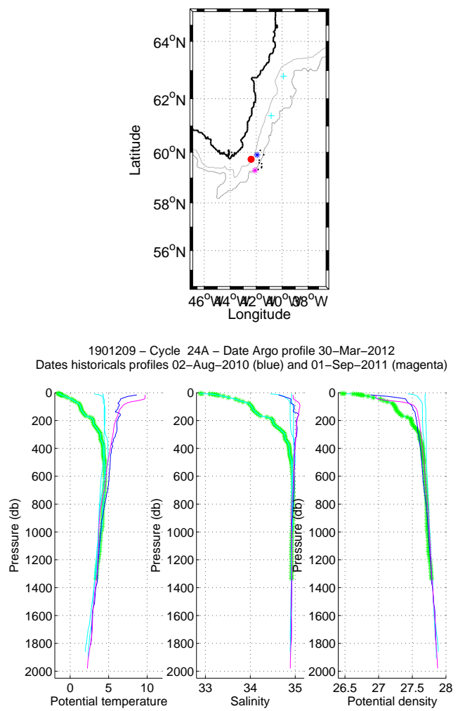
Figure 19: Flotteur 1901209, cycle 24A. Upper panel: Position of the analysed Argo profile (red) and of the nearest Argo profiles (black). The nearest Argo profile in time is in magenta while the nearest CTD profile in space is in blue. Lower panels: Temperature, salinity and potential density as function of pressure for the analysed Argo profile (stars) and for the nearest Argo profile in time (magenta line) and for the nearest Argo profile in space (blue line). The color of the analysed Argo profile represents the QC flag (green for a QC=1; blue for a QC=2; orange for a QC=3 and red for a QC=4).
