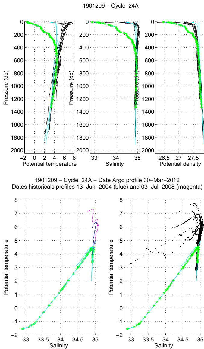
Figure 18: Float 1901209, cycle 24. The analysed CTD profile (stars) is compared to the nearest CTD profiles (black line) and to two specific profiles: the nearest CTD profile in time (magenta) and the nearest CTD profile in space (blue). The color of the analysed CTD profile represents the QC flag (green for a QC=1; blue for a QC=2; orange for a QC=3 and red for a QC=4). (Upper panels) Temperature (left panel), salinity (middle panel) and potential density (right panel) as function of pressure. (Lower panels) \theta/S diagrams.
