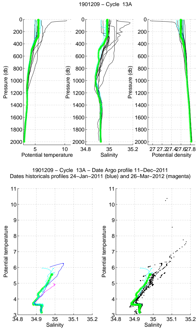
Figure 15: Float 1901209, cycle 13A. The analysed Argo profile (stars) is compared to the nearest Argo profiles (black line) and to two specific profiles: the nearest Argo profile in time (magenta) and the nearest Argo profile in space (blue). The color of the analysed Argo profile represents the QC flag (green for a QC=1; blue for a QC=2; orange for a QC=3 and red for a QC=4). (Upper panels) Temperature (left panel), salinity (middle panel) and potential density (right panel) as function of pressure. (Lower panels) \theta/S diagrams.
