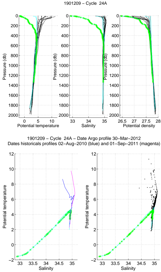
Figure 20: Float 1901209, cycle 24A. The analysed Argo profile (stars) is compared to the nearest Argo profiles (black line) and to two specific profiles: the nearest Argo profile in time (magenta) and the nearest Argo profile in space (blue). The color of the analysed Argo profile represents the QC flag (green for a QC=1; blue for a QC=2; orange for a QC=3 and red for a QC=4). (Upper panels) Temperature (left panel), salinity (middle panel) and potential density (right panel) as function of pressure. (Lower panels) \theta/S diagrams.
