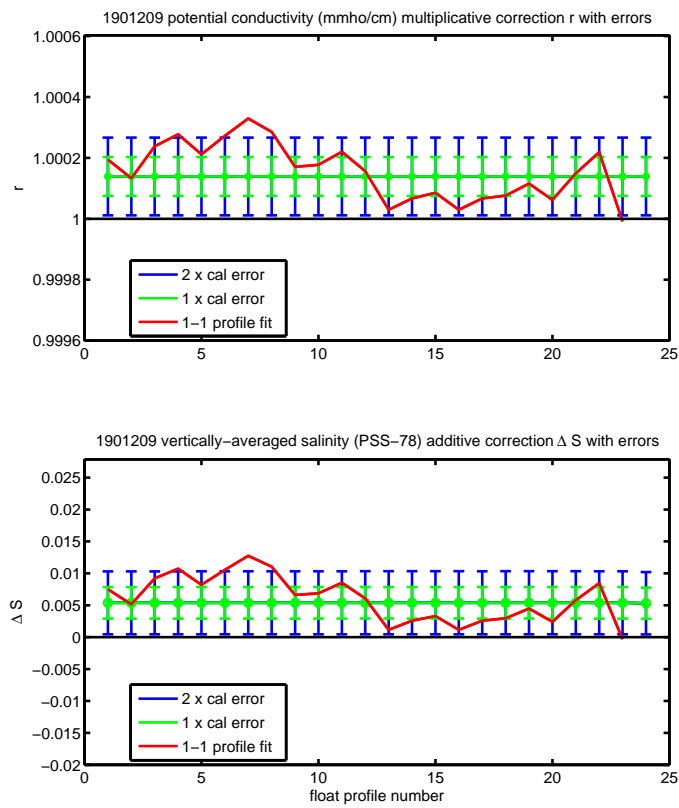
Figure 25: Correction proposed by the OW method.
