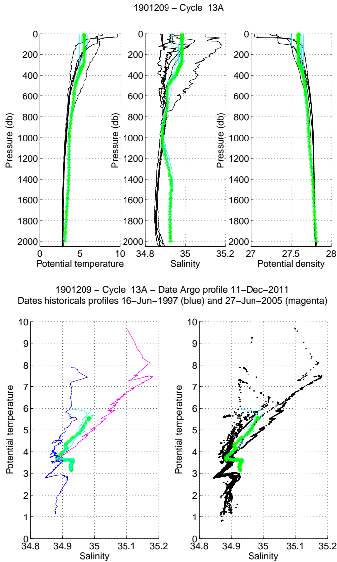
Figure 13: Float 1901209, cycle 13. The analysed CTD profile (stars) is compared to the nearest CTD profiles (black line) and to two specific profiles: the nearest CTD profile in time (magenta) and the nearest CTD profile in space (blue). The color of the analysed CTD profile represents the QC flag (green for a QC=1; blue for a QC=2; orange for a QC=3 and red for a QC=4). (Upper panels) Temperature (left panel), salinity (middle panel) and potential density (right panel) as function of pressure. (Lower panels) \theta/S diagrams.
