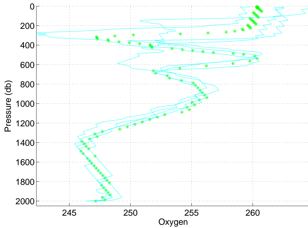
Figure 16: Float 1901209, cycle 13A. Oxygen data.
