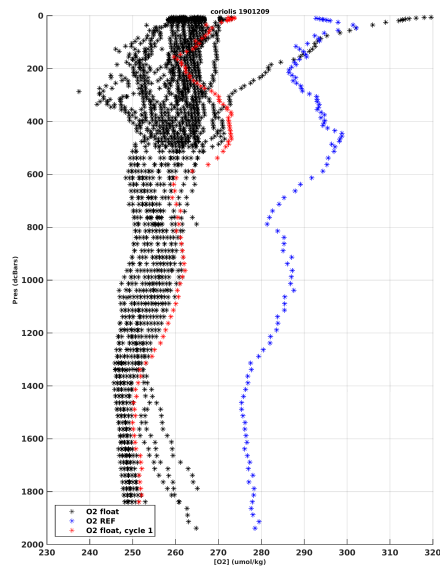
Figure 4: Profiles float 1901209 (black), O2 hydro reference (blue), O2 float cycle 1 (red)
