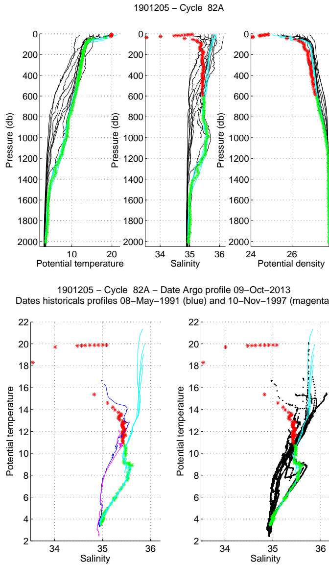
Figure 19: Float 1901205, cycle 82. The analysed CTD profile (stars) is compared to the nearest CTD profiles (black line) and to two specific profiles: the nearest CTD profile in time (magenta) and the nearest CTD profile in space (blue). The color of the analysed CTD profile represents the QC flag (green for a QC=1; blue for a QC=2; orange for a QC=3 and red for a QC=4). (Upper panels) Temperature (left panel), salinity (middle panel) and potential density (right panel) as function of pressure. (Lower panels) \theta/S diagrams.
