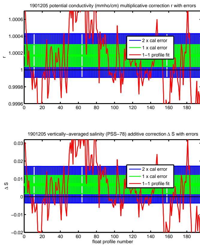
Figure 26: Correction proposed by the OW method.
