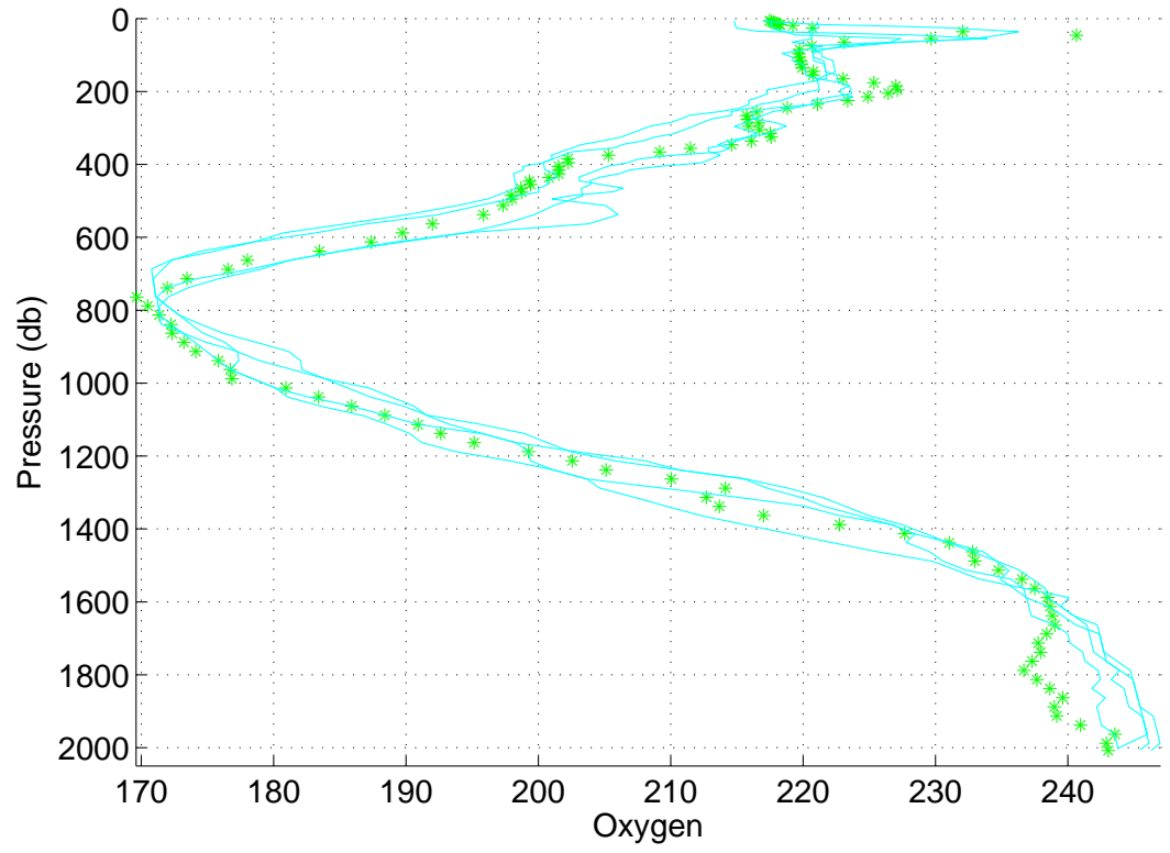
Figure 22: Float 1901205, cycle 82A. Oxygen data.
