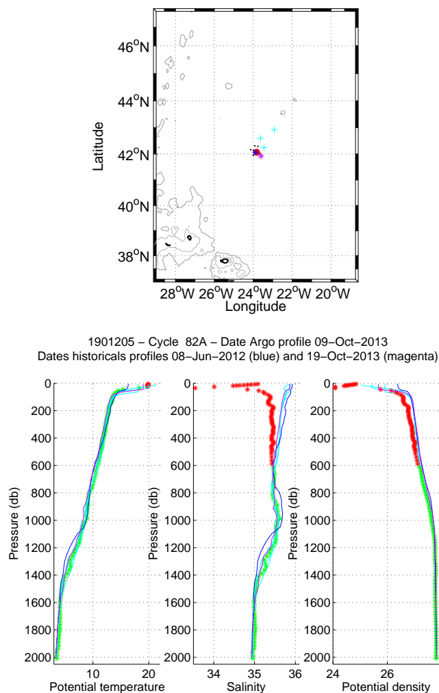
Figure 20: Flotteur 1901205, cycle 82A. Upper panel: Position of the analysed Argo profile (red) and of the nearest Argo profiles (black). The nearest Argo profile in time is in magenta while the nearest CTD profile in space is in blue. Lower panels: Temperature, salinity and potential density as function of pressure for the analysed Argo profile (stars) and for the nearest Argo profile in time (magenta line) and for the nearest Argo profile in space (blue line). The color of the analysed Argo profile represents the QC flag (green for a QC=1; blue for a QC=2; orange for a QC=3 and red for a QC=4).
