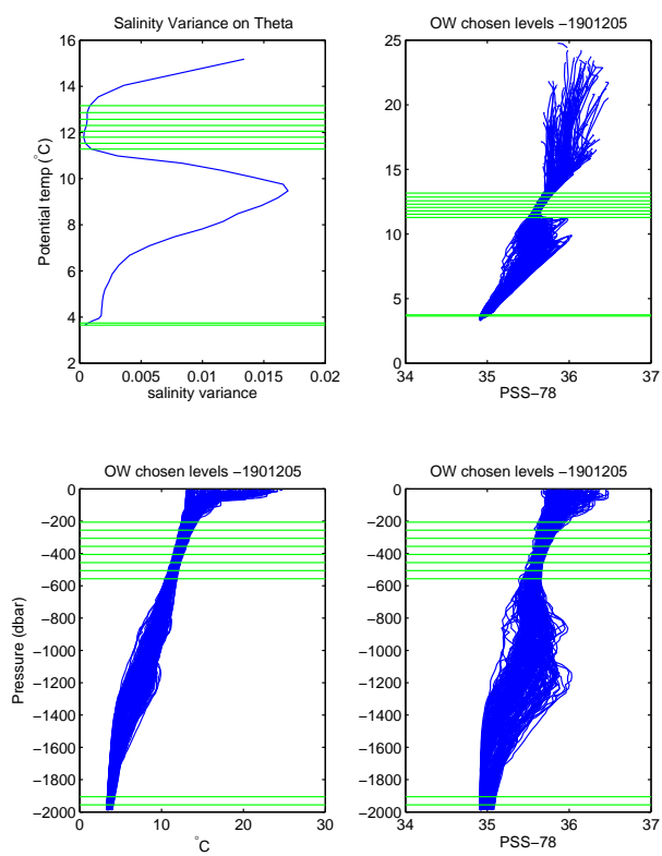
Figure 27: Chosed levels by the OW method.
