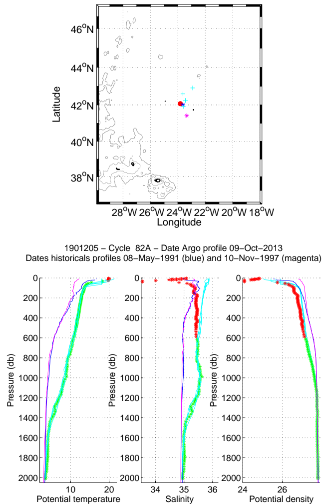
Figure 18: Flotteur 1901205, cycle 82. Upper panel: Position of the analysed CTD profile (red) and of the nearest CTD profiles (black). The nearest CTD profile in time is in magenta while the nearest CTD profile in space is in blue. Lower panels: Temperature, salinity and potential density as function of pressure for the analysed CTD profile (stars) and for the nearest CTD profile in time (magenta line) and for the nearest CTD profile in space (blue line). The color of the analysed CTD profile represents the QC flag (green for a QC=1; blue for a QC=2; orange for a QC=3 and red for a QC=4).
