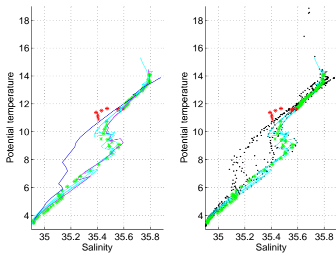
Figure 16: Float 1901205, cycle 31A. The analysed Argo profile (stars) is compared to the nearest Argo profiles (black line) and to two specific profiles: the nearest Argo profile in time (magenta) and the nearest Argo profile in space (blue). The color of the analysed Argo profile represents the QC flag (green for a QC=1; blue for a QC=2; orange for a QC=3 and red for a QC=4). (Upper panels) Temperature (left panel), salinity (middle panel) and potential density (right panel) as function of pressure. (Lower panels) \theta/S diagrams.
