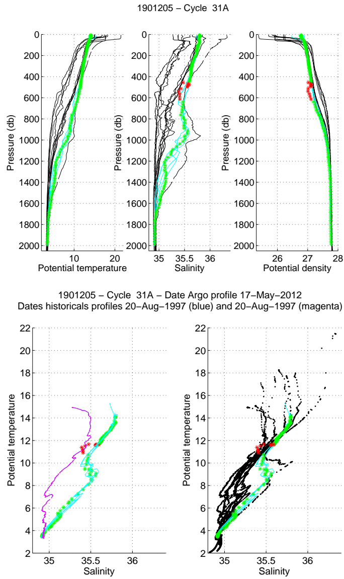
Figure 14: Float 1901205, cycle 31. The analysed CTD profile (stars) is compared to the nearest CTD profiles (black line) and to two specific profiles: the nearest CTD profile in time (magenta) and the nearest CTD profile in space (blue). The color of the analysed CTD profile represents the QC flag (green for a QC=1; blue for a QC=2; orange for a QC=3 and red for a QC=4). (Upper panels) Temperature (left panel), salinity (middle panel) and potential density (right panel) as function of pressure. (Lower panels) \theta/S diagrams.
