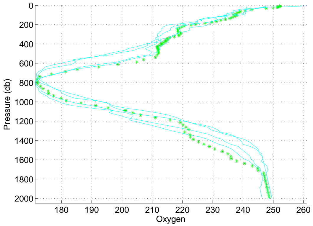
Figure 17: Float 1901205, cycle 31A. Oxygen data.
