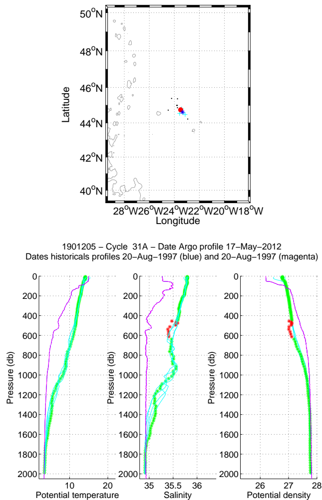
Figure 13: Flotteur 1901205, cycle 31. Upper panel: Position of the analysed CTD profile (red) and of the nearest CTD profiles (black). The nearest CTD profile in time is in magenta while the nearest CTD profile in space is in blue. Lower panels: Temperature, salinity and potential density as function of pressure for the analysed CTD profile (stars) and for the nearest CTD profile in time (magenta line) and for the nearest CTD profile in space (blue line). The color of the analysed CTD profile represents the QC flag (green for a QC=1; blue for a QC=2; orange for a QC=3 and red for a QC=4).
