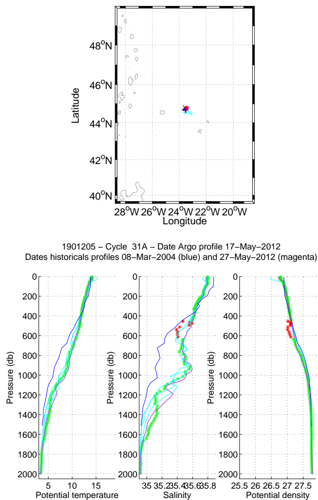
Figure 15: Flotteur 1901205, cycle 31A. Upper panel: Position of the analysed Argo profile (red) and of the nearest Argo profiles (black). The nearest Argo profile in time is in magenta while the nearest CTD profile in space is in blue. Lower panels: Temperature, salinity and potential density as function of pressure for the analysed Argo profile (stars) and for the nearest Argo profile in time (magenta line) and for the nearest Argo profile in space (blue line). The color of the analysed Argo profile represents the QC flag (green for a QC=1; blue for a QC=2; orange for a QC=3 and red for a QC=4).
