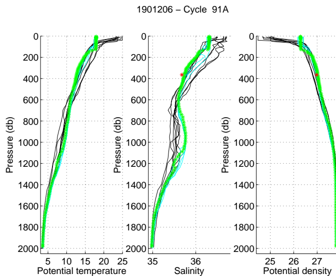
1901206 – Cycle 91A – Date Argo profile 09–Jan–2014 Dates historicals profiles 09–Jan–2014 (blue) and 09–Jan–2014 (magenta)
