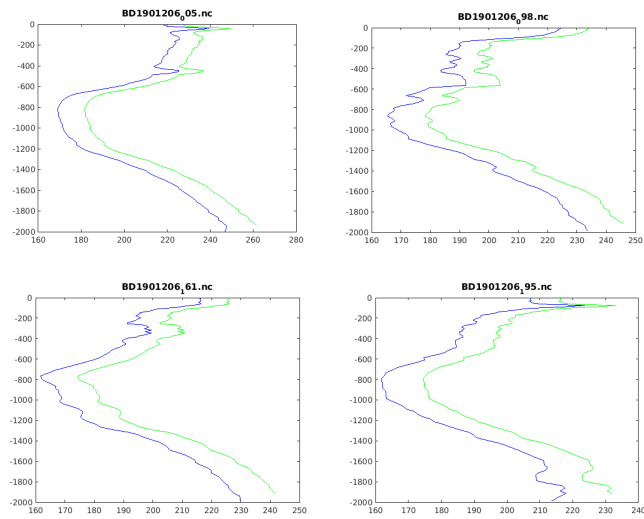
Figure 9: Float 1901206 : Corrected profiles in green.
