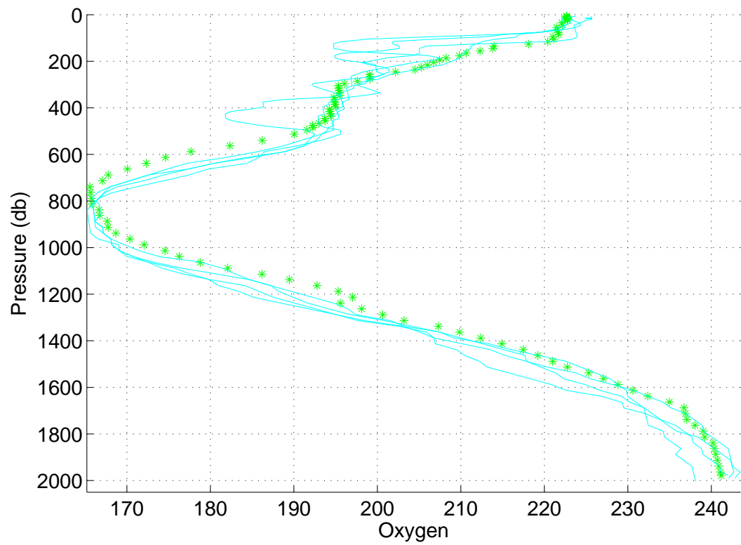
Figure 17: Float 1901206, cycle 91A. Oxygen data.
