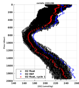
Figure 5: Profiles float 1901206 (black), O2 hydro reference (blue), O2 float cycle 1 (red)
