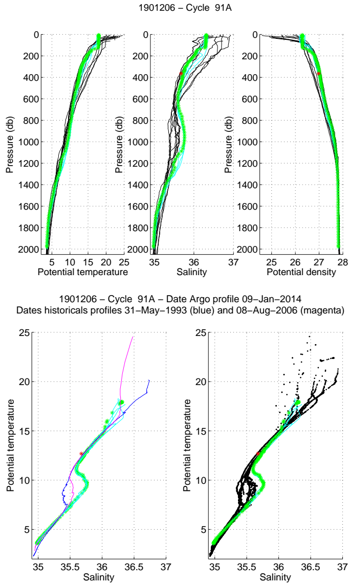
Figure 14: Float 1901206, cycle 91. The analysed CTD profile (stars) is compared to the nearest CTD profiles (black line) and to two specific profiles: the nearest CTD profile in time (magenta) and the nearest CTD profile in space (blue). The color of the analysed CTD profile represents the QC flag (green for a QC=1; blue for a QC=2; orange for a QC=3 and red for a QC=4). (Upper panels) Temperature (left panel), salinity (middle panel) and potential density (right panel) as function of pressure. (Lower panels) \theta/S diagrams.
