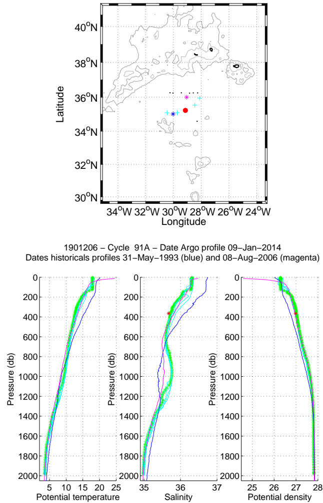
Figure 13: Flotteur 1901206, cycle 91. Upper panel: Position of the analysed CTD profile (red) and of the nearest CTD profiles (black). The nearest CTD profile in time is in magenta while the nearest CTD profile in space is in blue. Lower panels: Temperature, salinity and potential density as function of pressure for the analysed CTD profile (stars) and for the nearest CTD profile in time (magenta line) and for the nearest CTD profile in space (blue line). The color of the analysed CTD profile represents the QC flag (green for a QC=1; blue for a QC=2; orange for a QC=3 and red for a QC=4).
