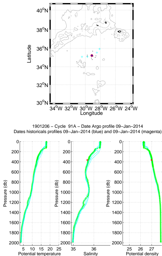
Figure 15: Flotteur 1901206, cycle 91A. Upper panel: Position of the analysed Argo profile (red) and of the nearest Argo profiles (black). The nearest Argo profile in time is in magenta while the nearest CTD profile in space is in blue. Lower panels: Temperature, salinity and potential density as function of pressure for the analysed Argo profile (stars) and for the nearest Argo profile in time (magenta line) and for the nearest Argo profile in space (blue line). The color of the analysed Argo profile represents the QC flag (green for a QC=1; blue for a QC=2; orange for a QC=3 and red for a QC=4).
