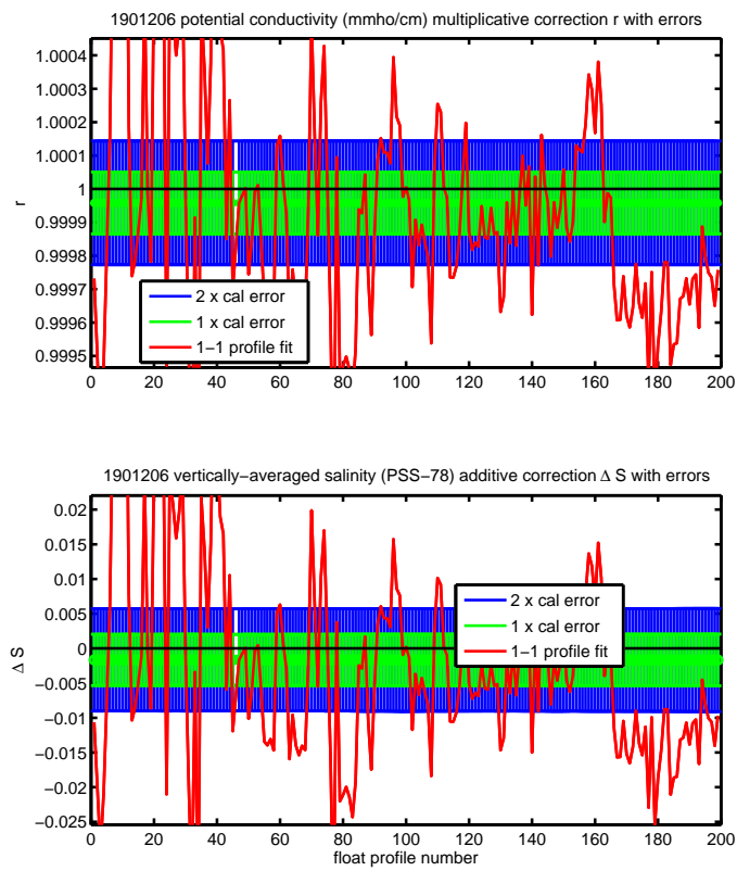
Figure 21: Correction proposed by the OW method.
