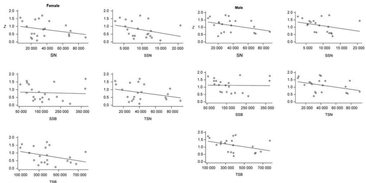
Figure 28. Total mortality ( Z ) based on revised IBTS Q1 cpue at age 1 vs. NP age 1 stock number (SN; r2f=0.08 , p=0.222 ; r2m=0.14 , p=0.106 ), spawning-stock number (SSN; r2f=0.11 , p=0.145 ; r2m=0.10 , p=0.178 ), SSB (t; r2f=0.00 , p=0.807 ; r2m=0.00 , p=0.942 ), total stock number (TSN; r2f=0.09 , p=0.177 ; r2m=0.15 , p=0.096 ), and total-stock biomass (TSB; t) ( r2f=0.12 , p=0.117 ; r2m=0.15 , p=0.089 ). Female figures at left, and male figures at right; regression lines are shown; numbers in millions and biomass in tonnes (t). Z is calculated according to Equation (1). (From Nielsen et al. 2012)
