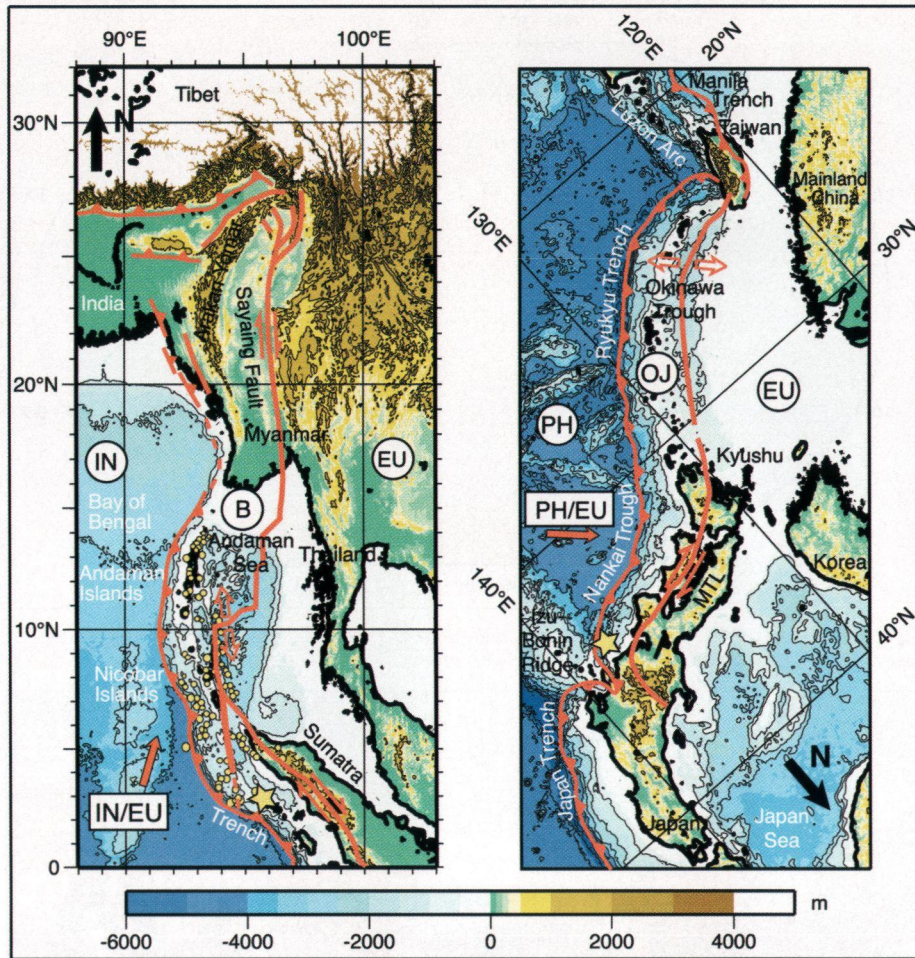
Fig. 1. Geodynamic context of the 2004 Sumatra great earthquake and similar geodynamic context between Japan and Taiwan. Yellow stars indicate the 2004 Sumatra earthquake and the expected-to-come Tokai earthquake [Le Pichon et al., 1996]. Yellow circles indicate the 2004 Sumatra aftershocks; the data are from the U.S. Geological Survey. Indonesian geodynamic context is from Institut de Physique du Globe de Paris (IPGP) and Ecole Normale Supérieure (ENS) de Paris. IN, India; B, Burma; EU, Eurasia; PH, Philippine; OJ, Okinawa-Japan; MTL, Median Tectonic Line.
