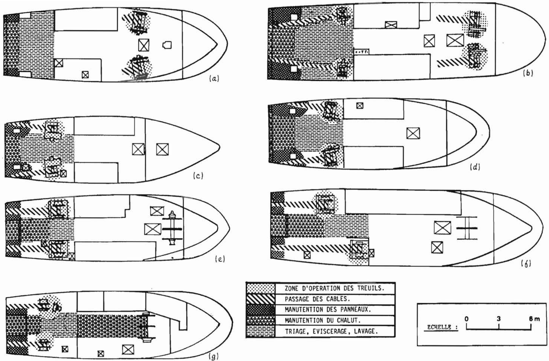
FIGURE 22 - TREUILS SCINDES
