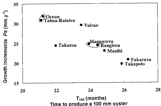
Figure 5. Annual growth increment P_S versus T_{100} . Sites for which differences were not significant are circled.
