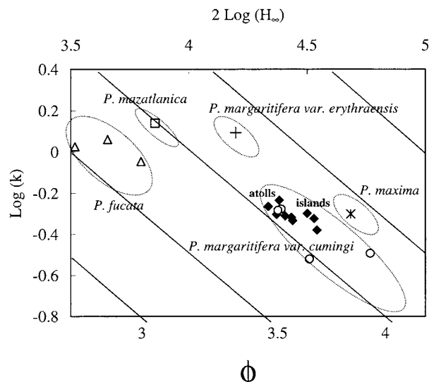
Figure 6. 3-D plot linking the growth parameters ( k , H_\infty and \Phi ) for several species of pearl oysters.
