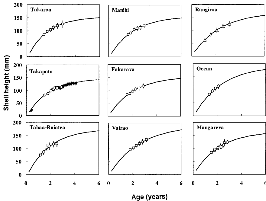
Figure 3. Von Bertalanffy models for the growth of P. margaritifera at nine sites in French Polynesia. Means \pm SE.
