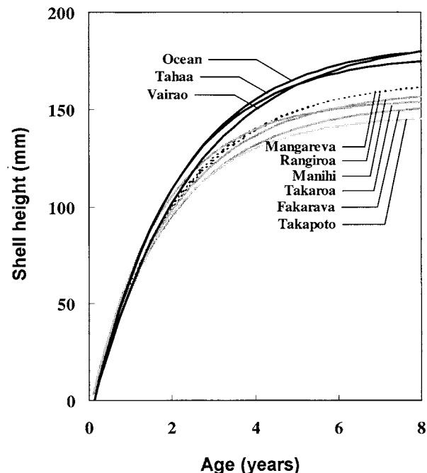
Figure 4. Comparison between the nine growth models obtained for P. margaritifera . Models obtained in ocean or island sites were significantly higher than models obtained in atolls sites.
