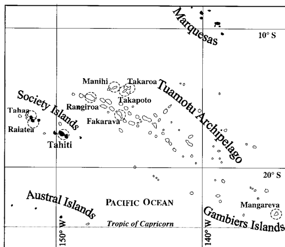
Figure 1. Location of experimental sites in French Polynesia. Polynesian islands are in black and atolls in white.
