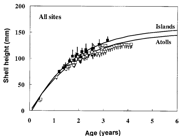
Figure 2. Comparisons between growth of P. margaritifera in culture in atolls (□), islands and in open ocean (■). Means \pm SE.
