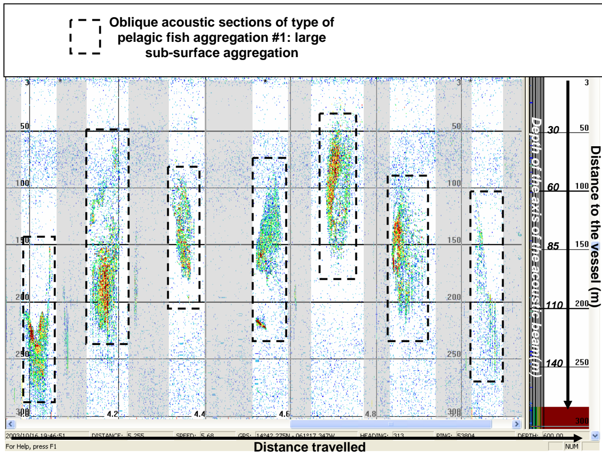
Figure 4-b : oblique beaming 120 kHz echogram of a rectangular survey with successive oblique sections of a sub-surface pelagic fish aggregation in green/yellow/red. Discarded sequences in grey.
