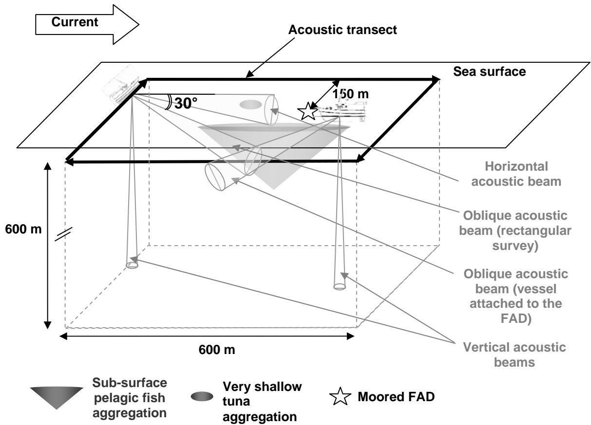
Figure 2: Oblique beaming acoustic survey patterns used around moored FADs in Martinique.
