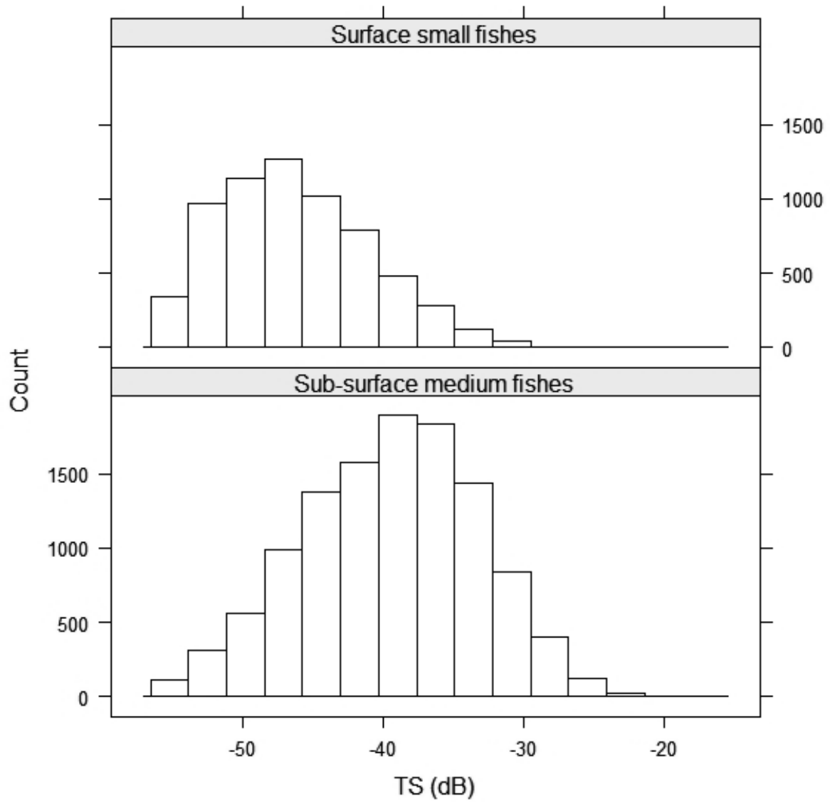
Figure 5: TS distribution of near-surface small fish and sub-surface medium-sized fish around a moored FAD in Martinique.
