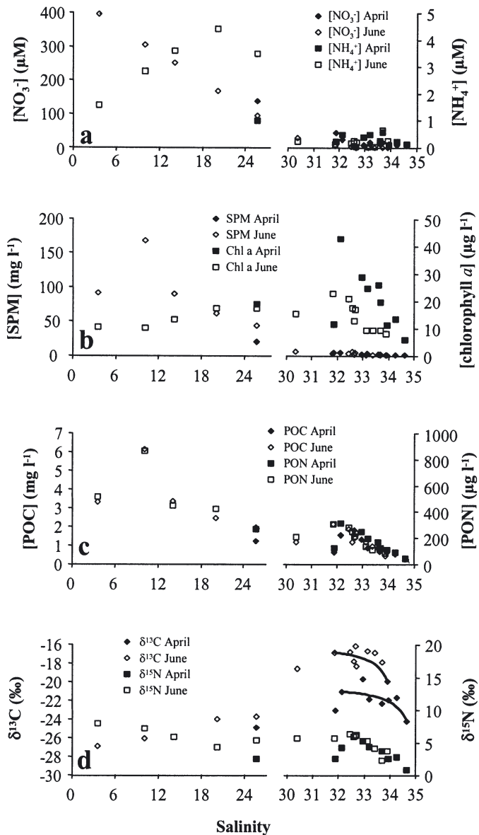
Fig. 2. (a) Nitrate and ammonium concentrations, (b) suspended particulate matter (SPM) and chlorophyll a ( chl a ) concentrations, (c) particulate organic carbon (POC) and nitrogen (PON) concentrations, and (d) \delta^{13}\text{C}_{\text{POC}} and \delta^{15}\text{N}_{\text{PON}} versus salinity during April and June 1997 in the Seine estuary (salinity < 30) and the Bay of Seine (salinity > 30). Curves in (d) correspond to mixing model (Eq. 1)
