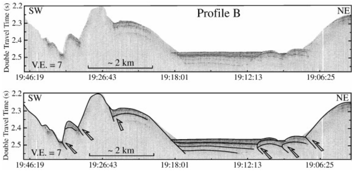
Figure 5: 3.5 kHz Profile B located in Fig. 3 across the same piggy-back basin than in Fig. 4, with numerous seaward vergence thrust faults showing signs of recent tectonic activity.
