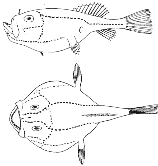
FIG. 10. - Chaunax pictus
