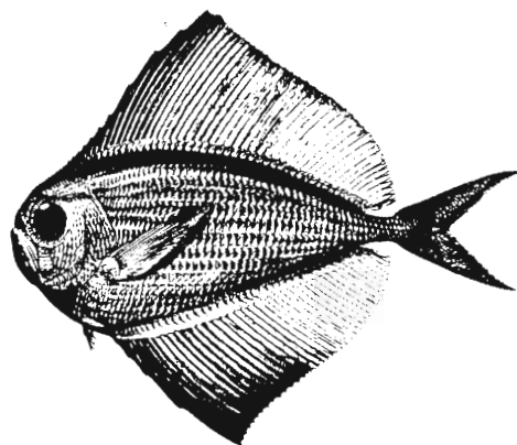
FIG. 7. - Pterycombus brama
