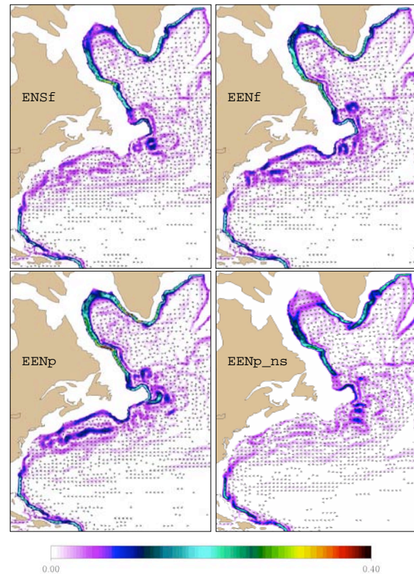
Fig. 2. Current vectors and velocities (colors, \text{m s}^{-1} ) at 1500 m along the northwestern boundary of the Atlantic, averaged over years 8–10 in the four simulations. Only one vector out of 16 is represented.
