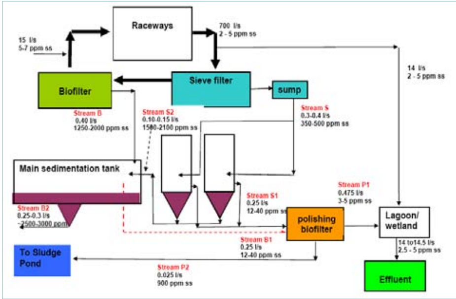
Figure 10: Overall configuration of sludge handling and waste water treatment at Højhoy. Note the labeling of the fluid streams. The details of these flows are shown in table 2. The diagram also shows the key flows and compositions of the flows within the farm.
