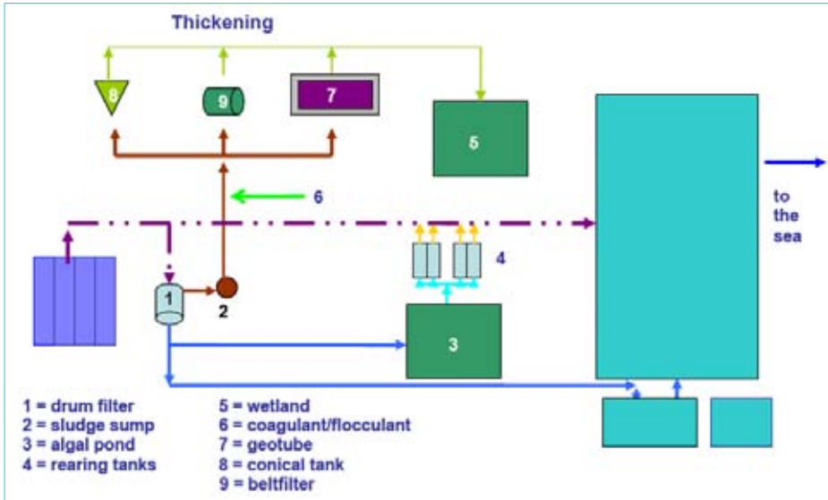
Figure 4: A schematic view of the treatment system
