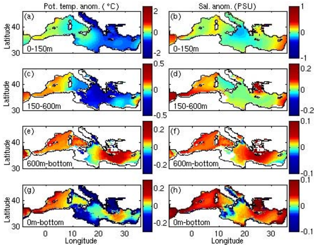
Figure 3 Differences between periods 1990-2000 and 1960-1970 of volume mean temperature ( ^{\circ}\text{C} , left) and salinity (right). From top to bottom respectively: layers 0-150m, 150-600m, 600m-bottom and 0m-bottom. The periods have been chosen to include and illustrate the major events occurring in both the Western and Eastern Mediterranean.
