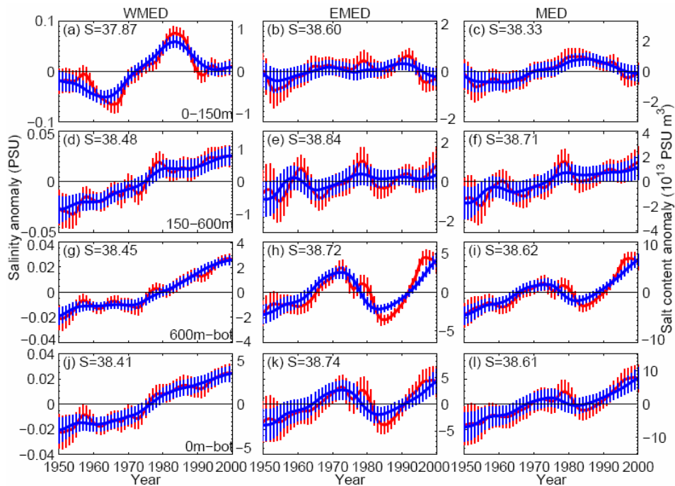
Figure 2 Same as 1 but for volume mean salinity (left scale) and salt content ( 10^{13} \text{ m}^3 , right scale) anomalies. Mean reference salinities are shown for each plot.
