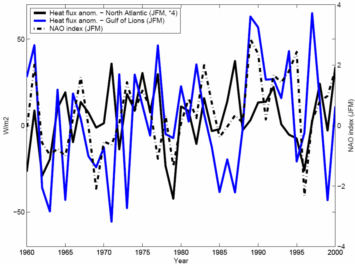
Figure 4 Time series of heat flux and temperature anomalies over period 1960-2000. A Winter time series (January to March) of NCEP-NCAR heat fluxes anomalies ( \text{W/m}^2 , left axis) over the North Atlantic (black, multiplied by 4), the Gulf of Lions (blue) and the corresponding NAO index (right axis, black). B Times series of temperature anomalies ( ^{\circ}\text{C} ) of the MEDAR Western Mediterranean Deep Water (3-year running window, blue), the pentadal North Atlantic (black) and the Global Ocean (green), and time integrated NCEP-NCAR heat fluxes over the Gulf of Lions (JFM, dashed blue) and the North Atlantic (all-year, dashed black).
