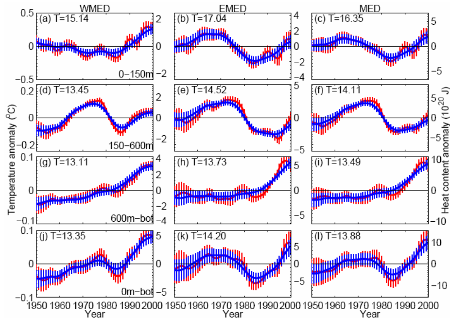
Figure 1 Pentadal and decadal variability of temperature for the period 1950-2000 for different areas and water volumes. From left to right: Western Mediterranean, Eastern Mediterranean and entire Mediterranean. Time series of volume mean temperature ( ^{\circ}\text{C} , left scale) and heat content ( 10^{20}\text{J} , right scale) anomalies. From top to bottom: layers 0-150m, 150-600m, 600m-bottom and 0m-bottom. Running temporal Gaussian windows are 10 years (blue) and 5 years (red). Vertical bars for each yearly estimate represent \pm 1 error standard deviation. Mean reference temperatures ( ^{\circ}\text{C} ) are shown for each plot.
