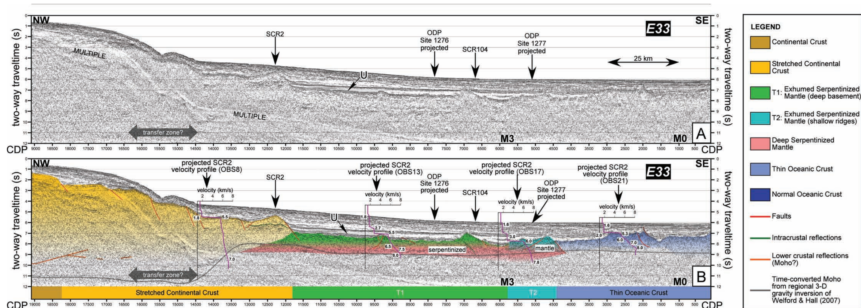
Figure 3. (a) Time migration of the Erable 33 (E33) seismic reflection profile with the corresponding interpretation of crustal domains (b). The legend to the right-hand side of the figure explains the shading and line colours used in the interpretation. The locations of magnetic anomalies M0 and M3 identified by Srivastava et al. (2000) are shown at the bottom of the sections. Crossovers with other seismic lines and projected ODP sites are identified with black arrows. The zone of overlap with the transfer zone discussed by Sibuet et al. (2007b) is highlighted with the double-pointed gray arrow. In (b), the overlain vertical velocity profiles were projected from the OBS locations in Fig. 7(b). The dark grey line corresponds to time-converted Moho constraints obtained from the 3-D regional gravity inversion from Welford & Hall (2007). The interpretations of crustal boundaries, labelled along the bottom of plot (b), are discussed in the text. Abbreviations: U-U reflection.
