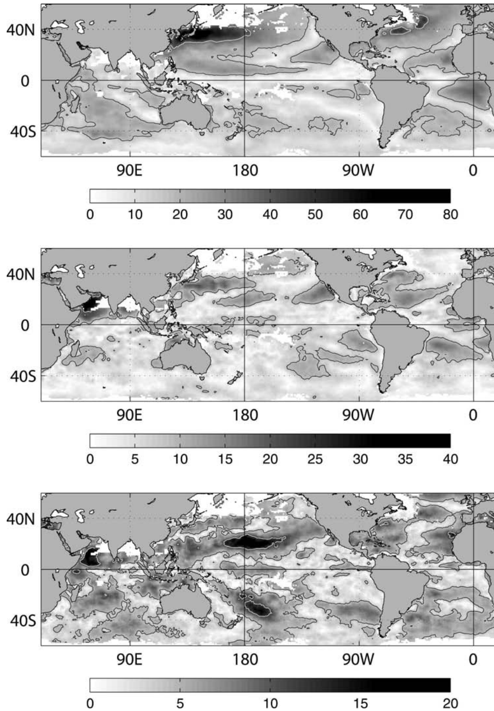
FIG. 2. Amplitudes of the (top) annual, (middle) semiannual, and (bottom) 4-month harmonics of the weekly latent heat flux time series (in \text{W m}^{-2} ). The solid white (black) contours in the top, middle, and bottom panels correspond, respectively, to 50 (20), 30 (10), and 15 (5) \text{W m}^{-2} . The white areas are regions of missing data.
