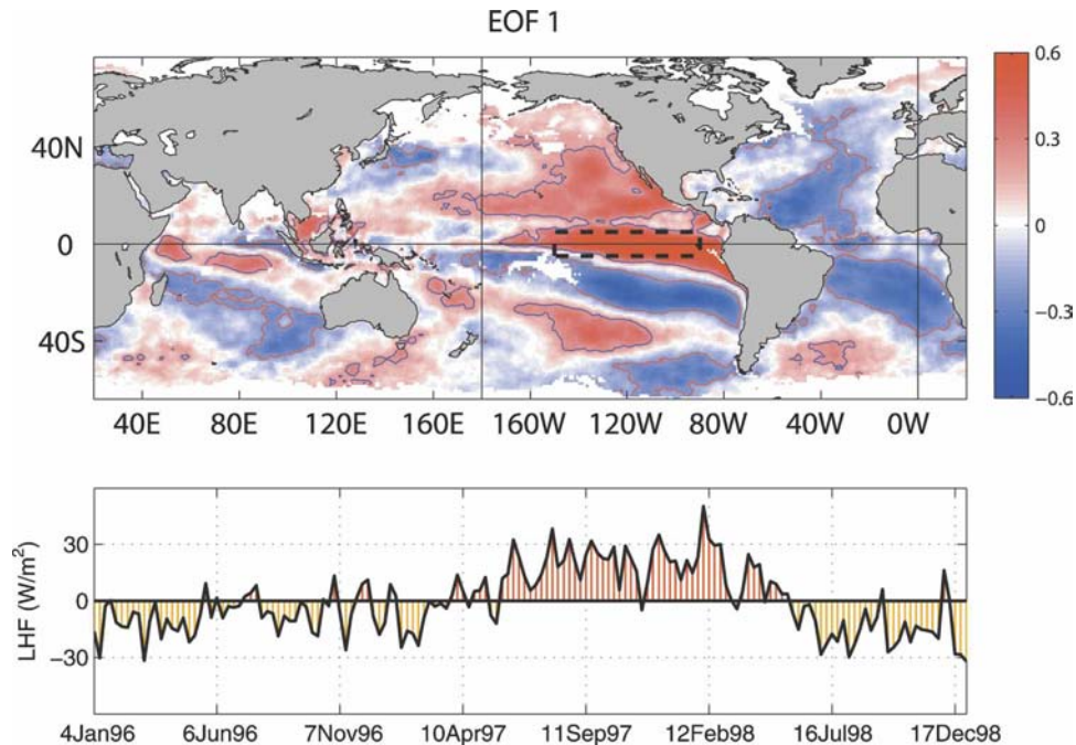
FIG. 4. Leading EOF of the weekly latent heat flux anomalies describing El Niño variability and accounting for 5% of the global anomalous variance. The latent heat flux anomalies were calculated by removing from every time series the mean (Fig. 1, top panel) as well as the seasonal cycle estimated by adding the three harmonics shown in Figs. 2 and 3. (top) Spatial distribution of the temporal correlation coefficient between the latent heat flux anomalies and the modal reconstruction over the Niño-3 index region indicated with the dashed box. The solid blue and red lines indicate the +0.21 and -0.21 contours, respectively. (bottom) Temporal reconstruction of the mode-related variability averaged over the Niño-3 index region.
