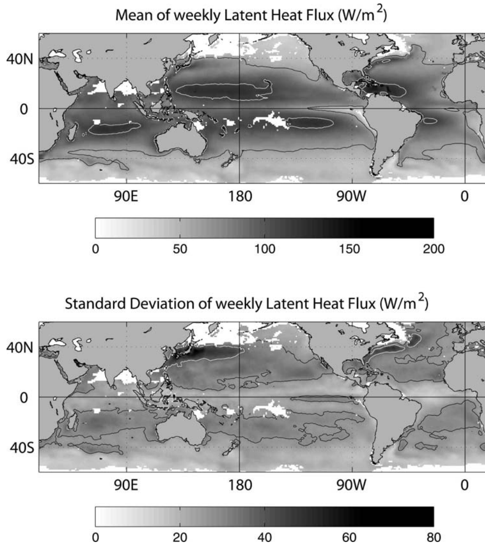
FIG. 1. Maps of the (top) mean and (bottom) standard deviation of the 3-yr (1996–98) weekly latent heat flux time series (in \text{W m}^{-2} ). The solid white (black) contours in the top and bottom panels, respectively, correspond to 150 (75) and 50 (35) \text{W m}^{-2} . The white areas are regions of missing data.
