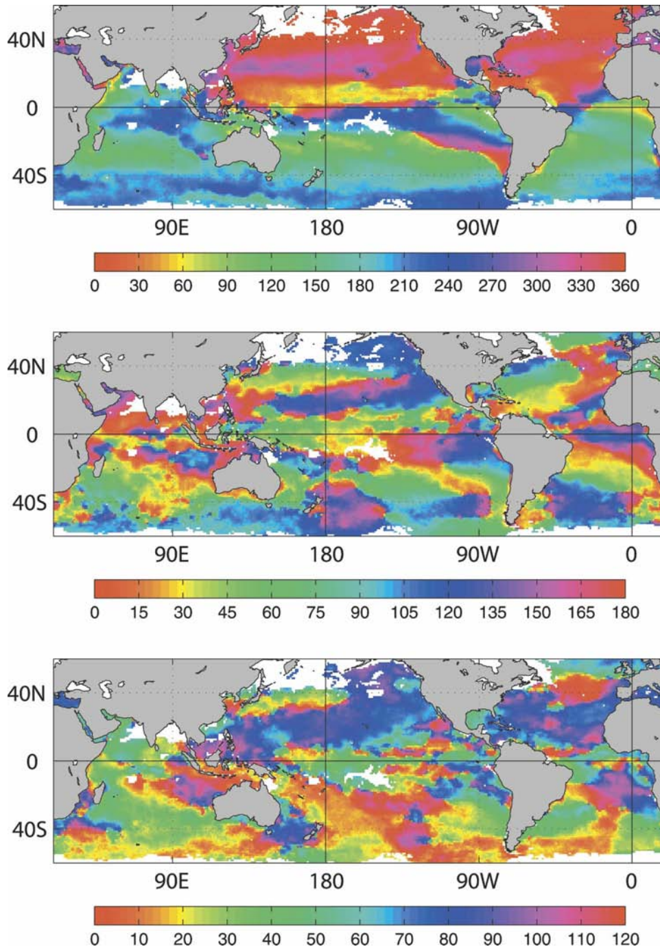
FIG. 3. Phases of the (top) annual, (middle) semiannual, and (bottom) 4-month harmonics of the weekly latent heat flux time series. The phase values correspond closely with the day of the year when the latent heat flux reaches a maximum. For the semiannual and 4-month harmonics one more maximum and two more maxima, respectively, occur 180 and 120/240 days after the day indicated. The white areas are regions of missing data.
