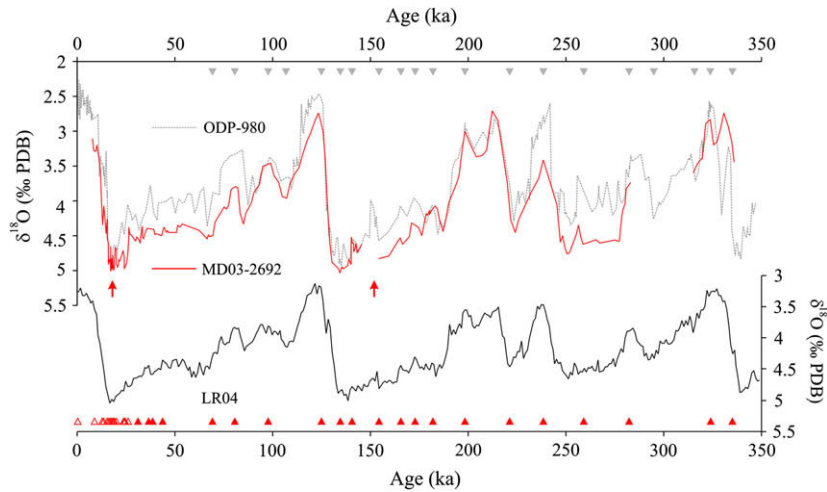
Fig. 4. Basis of the age models for cores MD03-2692 and ODP-980. Age control was established by alignment of the benthic foraminifera oxygen isotope records ( \delta^{18}\text{O} (‰), continuous red line: MD03-2692 and dotted grey line: ODP-980 (McManus et al., 1999)) with the LR04 benthic oxygen isotope stack of Lisiecki and Raymo (2005). Filled red and grey triangles indicate positions of the tie points for cores MD03-2692 and ODP-980, respectively. Open red triangles indicate the position of the AMS ^{14}\text{C} datings for core MD03-2692. Red arrows indicate the position of the laminated facies in core MD03-2692 (For interpretation of the references to colour in this figure legend, the reader is referred to the web version of this article).
