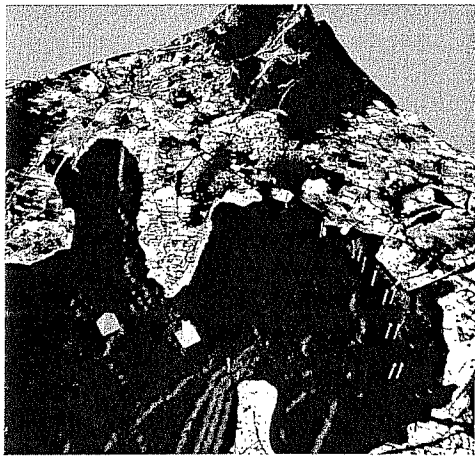
Figure 6 : detail of the north part of Thau lagoon depicting current field (red), various lighthouses and beacons, water treatment plant (dice), Oyster beds (grey rectangles), REMI monitoring network point (yellow).
