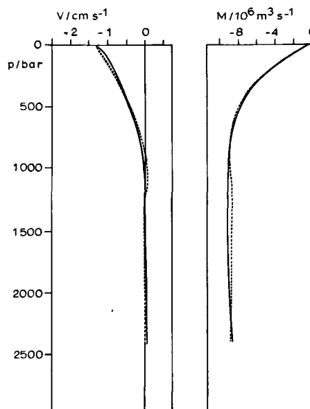
Figure 7 Geostrophic meridional velocity V relative to 1,300 dbar (left side) and the corresponding cumulative volume transport M (right side). Solid line is obtained from temperature-salinity-depth data, dashed line from temperature-depth data and mean T/S curve.
