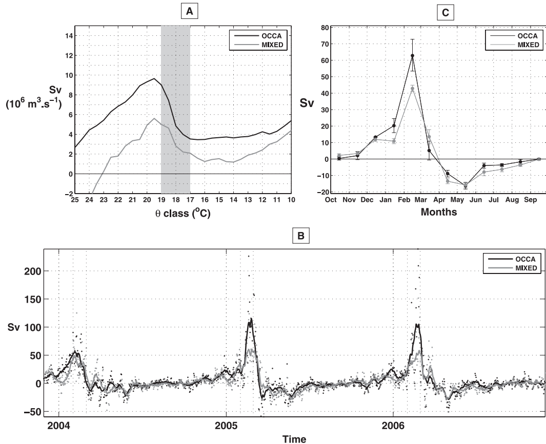
FIG. 3. (a) Three years (2004–06) of mean transformation rates \overline{F(\theta)} in OCCA (black) and MIXED (gray) datasets. The shaded area indicates the EDW range between 19^{\circ} and 17^{\circ}C . (b) Time series of EDW formation rate \Delta F = F(19) - F(17) from 2004 to 2006. Plain lines are daily time series that have been low-pass filtered with a 7-day cut-off frequency. Light black and gray dots are daily values for OCCA and MIXED datasets. First day of January, February, and March are denoted by the vertical dashed lines at the beginning of each year. (c) Composite net formation rate \Delta F(18^{\circ}C) obtained by averaging monthly mean fields over the 3-yr time series shown in (b). Vertical bars mark the 3-yr standard deviation amplitude. Circles are the values obtained by integrating in space monthly mean formation maps, such as those shown in Fig. 8.
