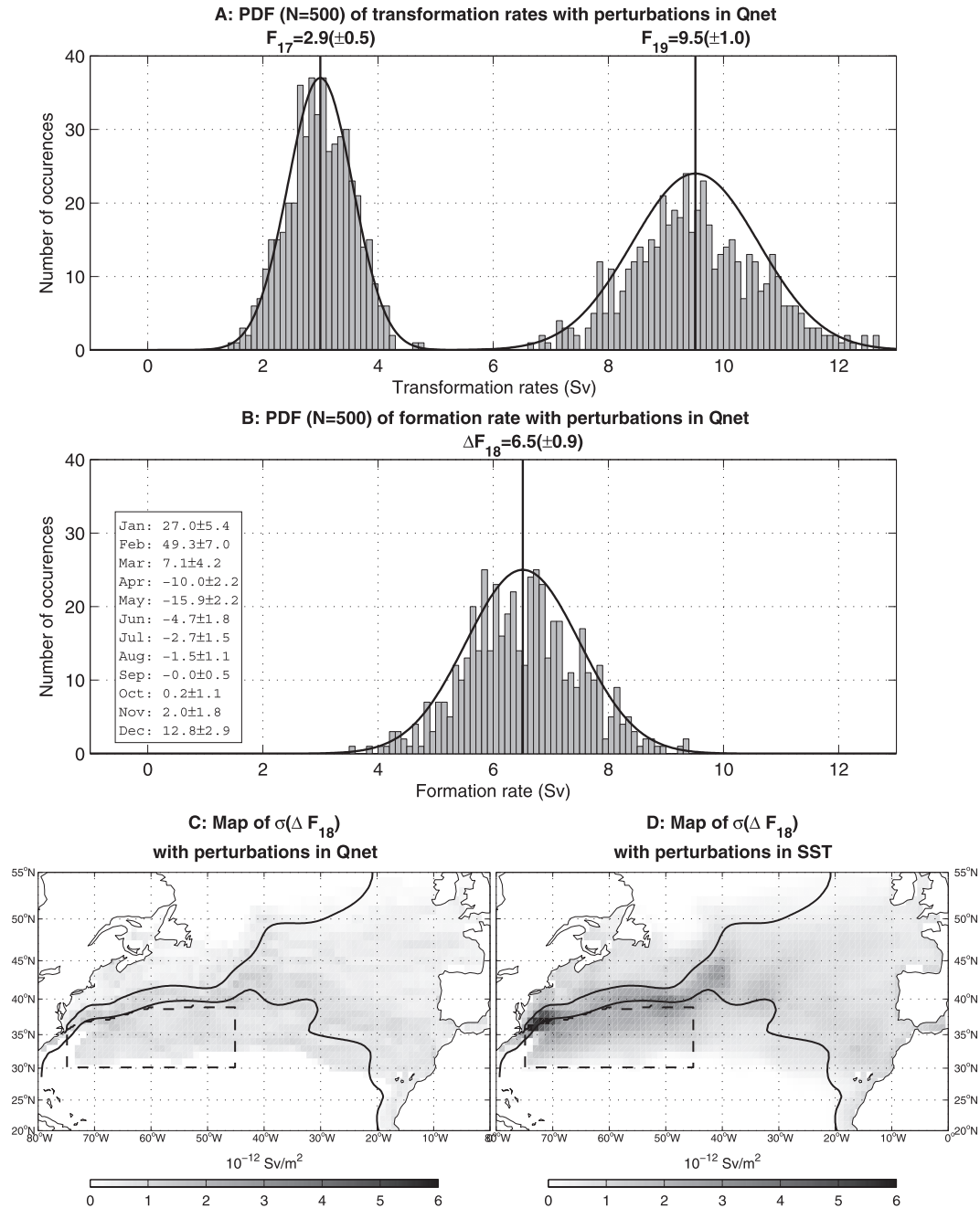
FIG. 9. From the OCCA dataset: PDFs of (a) transformation F(17^{\circ}\text{C}) , F(19^{\circ}\text{C}) and (b) formation \Delta F(18^{\circ}\text{C}) rates for the first ensemble experiment where only the air-sea heat flux is perturbed (see text). In (b), monthly mean and standard deviation of \Delta F(18^{\circ}\text{C}) are tabulated. (bottom) Maps of local standard deviation of \Delta F(18^{\circ}\text{C}) for the (c) first and (d) second ensemble with perturbations on Q_{net} and SST only, respectively. Dashed black line is the formation box area and two thick black contours are mean -0.2 - and -0.6 -m SSH from OCCA .
