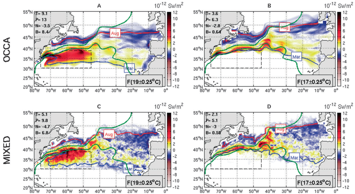
FIG. 4. The mean transformation maps of (left) \overline{\mathcal{F}}(19^{\circ}\text{C}) and (right) \overline{\mathcal{F}}(17^{\circ}\text{C}) ( \text{Sv m}^{-2} ) for the 3-yr period 2004–06: (top) OCCA dataset and (bottom) MIXED dataset. Red (blue) contours are the August (March) mean position of the 19^{\circ} and 17^{\circ}\text{C} isotherms; green contours are the mean -0.2\text{-} and -0.6\text{-m} SSH from OCCA. Integral quantities of the fields are shown in the upper-left corner of each map (Sv) over the total domain (T), for positive areas only (P), for negative areas only (N), and over the dashed black box (B). A nonlinear color scale has been used to reveal patterns.
