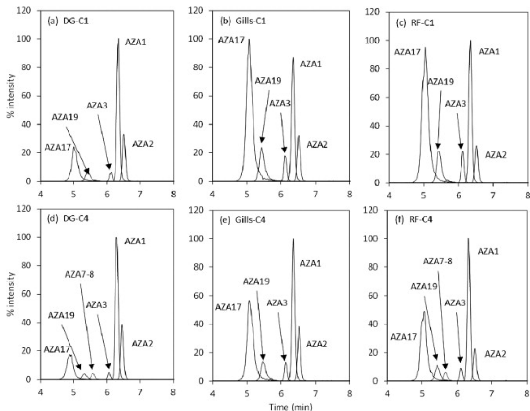
Figure 3. Comparison of metabolites profiles in mussel tissues after exposure to the different conditions by LC–MS/MS analysis (method A): (a) Digestive glands (DG), (b) Gills, and (c) Remaining flesh (RF) after mussel exposure to dissolved AZAs ( 7.5 \mu\text{g mL}^{-1} ) (Condition 1); and (d) DG, (e) Gills, and (f) RF after mussel exposure to live A. spinosum cells ( 1 \times 10^5 \text{ cell mL}^{-1} ) (Condition 4).
