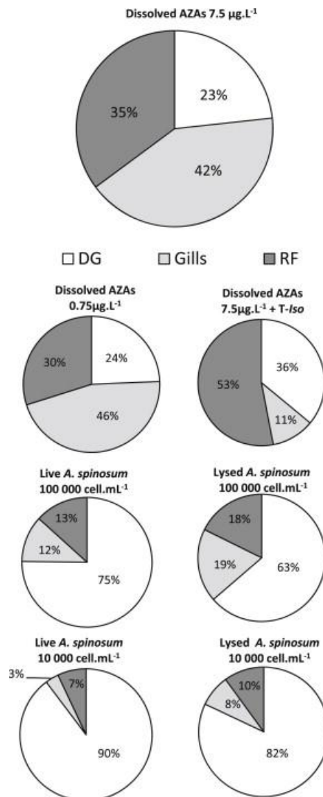
Figure 2. Total AZA tissue distribution in mussels (digestive gland (DG, □), remaining flesh (RF, ■) and gills (▣)) after 24 h of exposure to dissolved AZAs, live A. spinosum or lysed A. spinosum at different concentrations.
