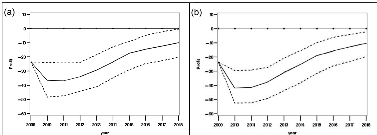
Figure 5. Annual profits (million €) of the large French trawlers, resulting from 200 simulations run with either the data-rich (median: thick & plain line, 5 th and 95 th percentiles: thick & dotted lines) or the data-limited (median: thin & plain line, 5 th and 95 th percentiles: thin & dotted lines) blue ling harvest control rules. The initial blue ling stock-at-age numbers correspond to either (a) the actual 2009 spawning biomass or (b) 10% of the unfished spawning biomass. The plain dotted line represents the zero-profit level.
