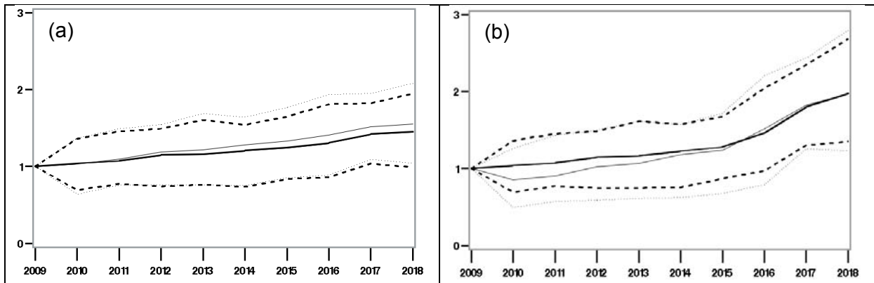
Figure 6. Blue ling. Annual catch per unit of effort (median: thin & plain line, 5 th and 95 th percentiles: thin & dotted lines) for large French trawlers, and spawning stock biomass (median: thick and plain line, 5 th and 95 th percentiles) relative to their respective 2009 value, resulting from 200 simulations run with the data-rich blue ling harvest control rule. The initial blue ling stock-at-age numbers correspond to either (a) the actual 2009 spawning biomass or (b) 10% of the unfished spawning biomass.
