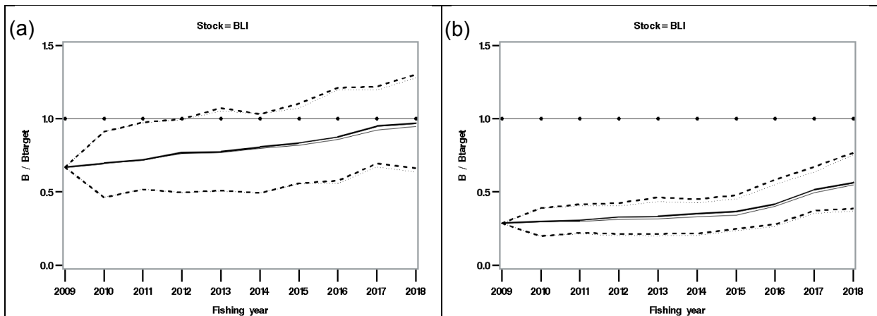
Figure 1. Blue ling. Annual spawning stock biomass relative to B_{target} resulting from 200 simulations run with either the data-rich (median: thick & plain line, 5 th and 95 th percentiles: thick & dotted lines) or the data-limited (median: thin & plain line, 5 th and 95 th percentiles: thin & dotted lines) blue ling harvest control rules. The initial blue ling stock-at-age numbers correspond to either (a) the actual 2009 spawning biomass or (b) 10% of the unfished spawning biomass. The plain dotted line represents the targeted level.
