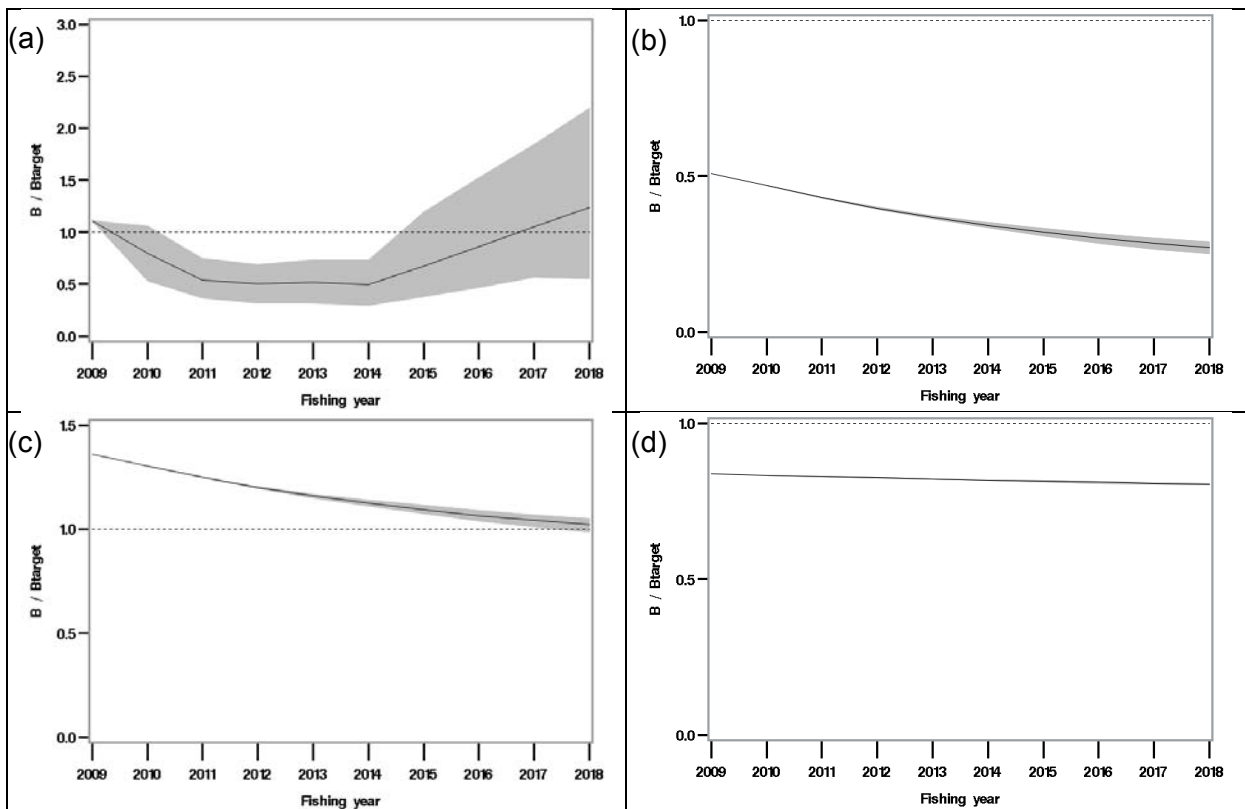
Figure 3. Annual spawning stock biomass (or total biomass) relative to B_{target} resulting from 200 simulations run with the data-rich blue ling harvest control rule; (a) saithe, (b) roundnose grenadier, (c) black scabbardfish, (d) deepwater sharks. The initial blue ling stock-at-age numbers correspond to the actual 2009 spawning biomass. The median (plain line) and the area between the 5 th and the 95 th percentiles (shaded in grey) are represented.
