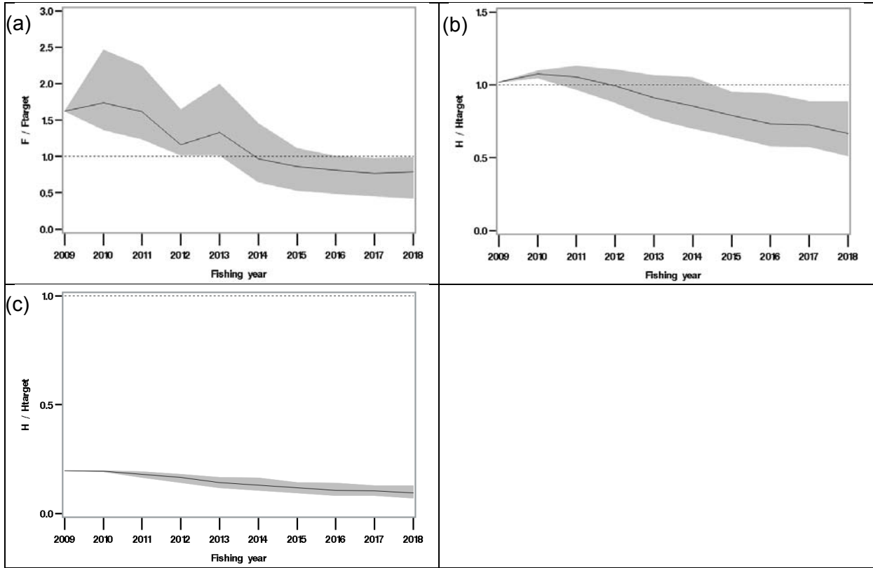
Figure 4. Annual fishing mortality (or harvest rate) relative to F_{target} (or H_{target} ) resulting from 200 simulations run with the data-rich blue ling harvest control rule; (a) saithe, (b) roundnose grenadier, (c) black scabbardfish. The initial blue ling stock-at-age numbers correspond to the actual 2009 spawning biomass. The median (plain line) and the area between the 5 th and the 95 th percentiles (shaded in grey) are represented.
