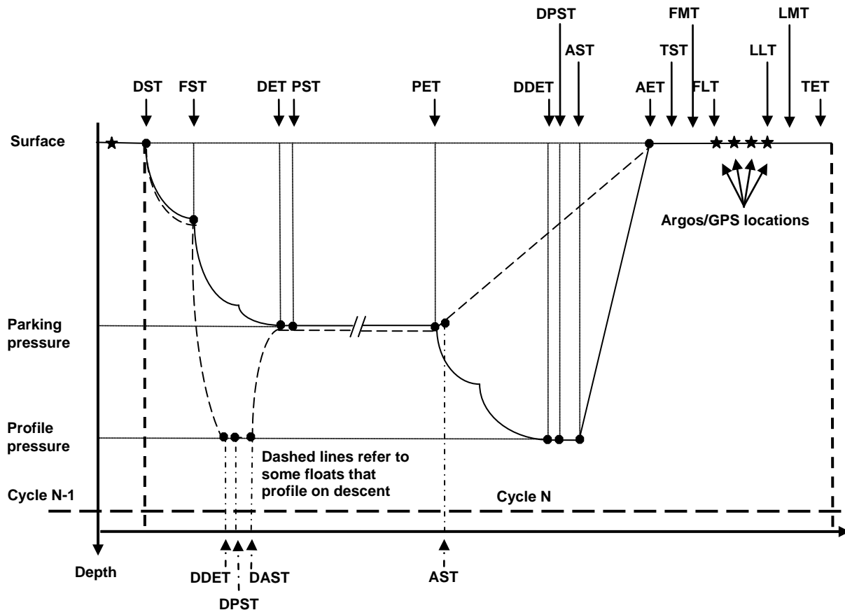
Figure 1: Figure showing float cycle and the cycle timing variables. Floats can profile either on descent or ascent. Most floats profile on ascent. Their float path is shown with a solid black line. Some floats profile on descent. One such float, the new SOLO-II Deep float, has a cycle as shown by the dashed line.
