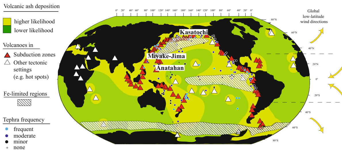
Fig. 5.24 World-map illustrating the distribution of subaerial (Holocene-) active volcanoes indicated as triangles (highlighted are the volcanoes cited in the text). Oceanic regions with higher likelihood of volcanic ash deposition are shown as yellow regions (Olgun et al. 2011), based on marine sediment core data, the frequency of tephra layers found in the ocean
