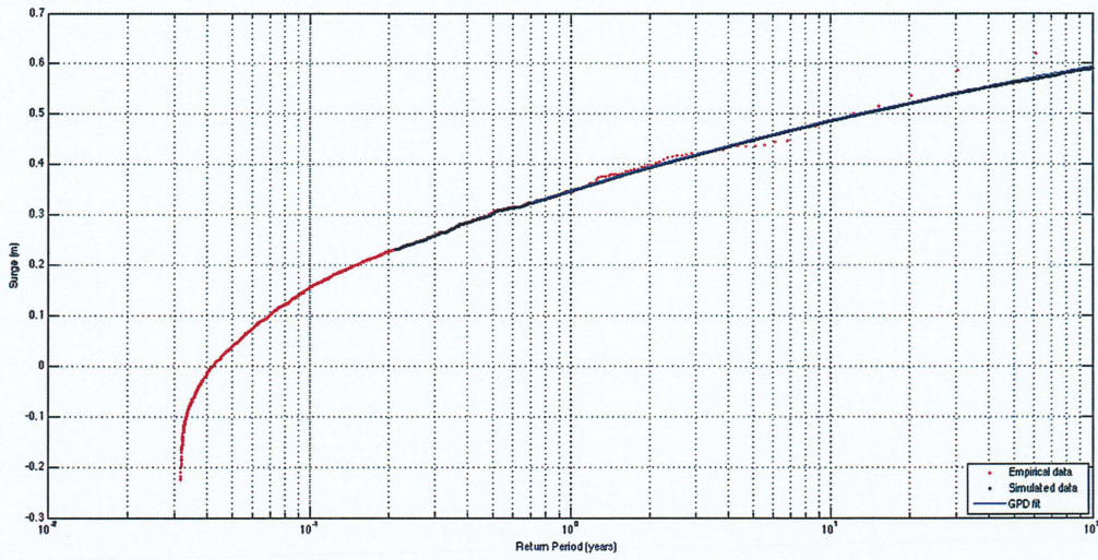
Figure 7 Comparison of the marginal distribution of S: empirical, simulated and GPD fit
