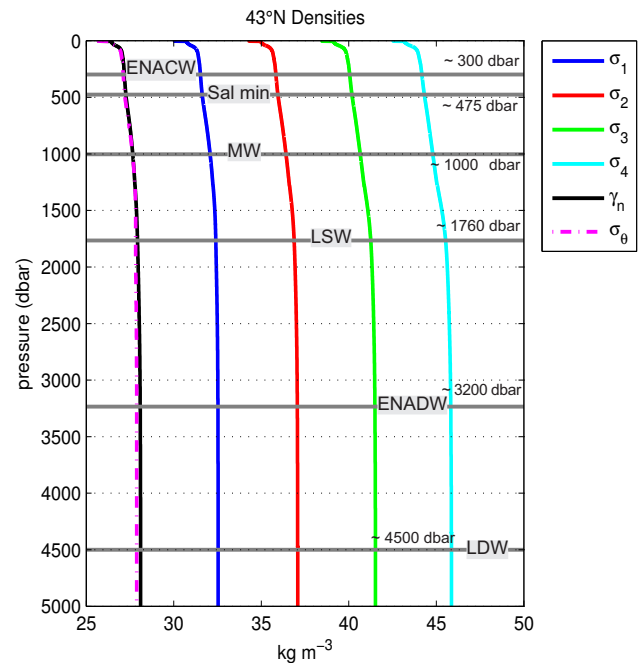
Fig. 2. Time and zonally averaged potential density relative to the sea surface ( \sigma_\theta ), 1000 dbar, 2000 dbar, 3000 dbar, 4000 dbar ( \sigma_1, 2, 3, 4 ) and neutral density ( \gamma^n ) as a function of pressure.
