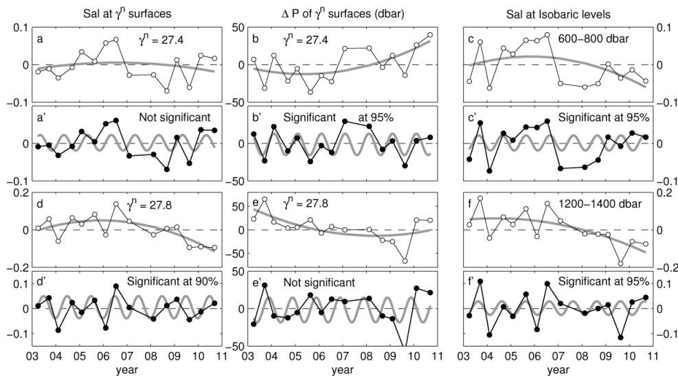
Fig. 6. Time series of (a), (d) salinity anomaly at isopycnal levels \gamma^n = 27.4 and 27.8 , (b), (e) pressure (anomaly) at which these isopycnal levels lie, (c), (f) salinity anomaly at isobaric levels 600–800 and 1200–1400 dbar, roughly corresponding to these isopycnals. A two-degree polynomial trend is computed for each series (thick gray). Prime versions of figures correspond to the simple harmonic analysis applied to the residual (time series minus trend, black dots) following Eq. (3).
