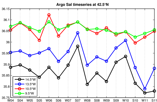
Fig. 12. Time series of the salinity field along the 42.5° N section from the interpolated field at 1000–1250 dbar level from Argo floats for the period 2004–2011, at different locations in the slope (9.5° W and 10.5° W) and the outer ocean region west of the Galicia Bank (13.5° W and 14.5° W)
