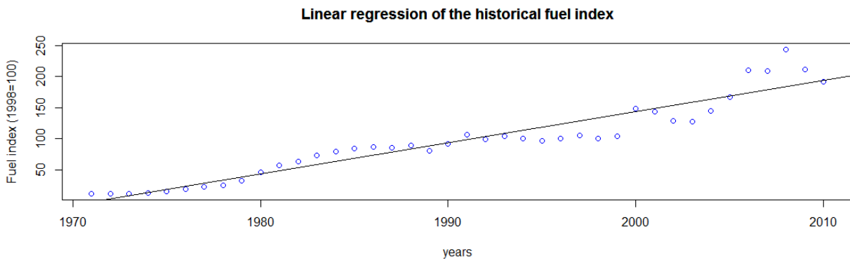
Figure 4.8: Linear regression of fuel price index relying on historical data from 1971 to 2010. R^2 = 0.9033 and Pvalue = 2.2 * 10^{-16} ( <0.05 , significant). The slope of the regression line is 4.9831 (meaning an increase of 5% per year). Data source: ABARES (2010) .
