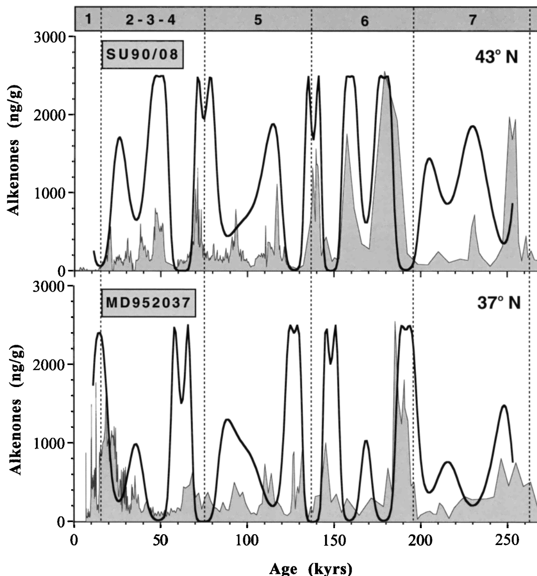
Figure 7. Modeled productivity at sites SU90/08 and MD952037. Comparison of the reconstructed paleoproductivity (solid thick line) to the alkenone-derived productivity records (shaded area) for each location. Numbers above the plot refer to the oxygen isotopic stages, and vertical dashed lines refer to the transition between them.
