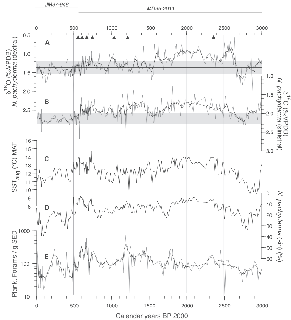
Figure 4. Temporal changes in surface ocean variability at the Vøring Plateau over the past 3000 years. The distribution of data from the two spliced cores is shown at the top. Comparisons between (a and b) changes in the oxygen isotope composition of N. pachyderma (dex) and N. pachyderma (sin), (c) August SST, (d) relative abundance of N. pachyderma (sin) (note the inverted scale), and absolute abundance of planktic foraminifers (>150 \mu\text{m} ) per gram dry bulk sediment (smoothed by a 3-point moving average). The absolute foraminiferal abundance data is plotted on a logarithmic scale to emphasize the variability at low abundances. Figures 4a, 4b, and 4e show raw data (gray line) and a 5-point moving average (black line) of the raw data. Shaded bars denote typical core top oxygen isotope values of N. pachyderma (dex) and N. pachyderma (sin) taken from Johannessen [1992]. Thin, solid lines across the shaded bars represent average \delta^{18}\text{O} values for the past 50 years in JM97-948/2A. Filled triangles denote radiocarbon age control points.
