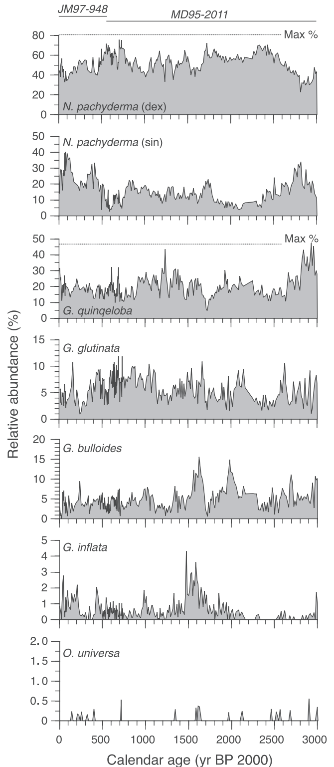
Figure 3. Temporal changes in the relative abundance of selected (major) planktic foraminifer species in cores JM97-948/2A and MD95-2011 over the past 3000 years. The distribution of data from the two spliced cores is shown at the top. Stippled lines show the maximum abundance of N. pachyderma (dex) and G. quinqueloba in the modern core top database.
