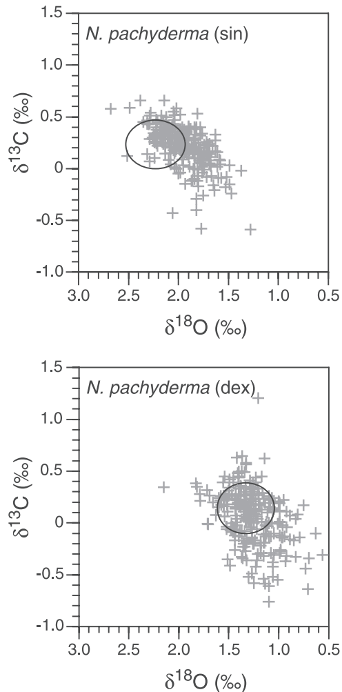
Figure 5. Characteristics of surface waters in the eastern Norwegian Sea over the past 3000 years based on planktic foraminiferal \delta^{18}\text{O} and \delta^{13}\text{C} measurements. Circles denote modern \delta^{18}\text{O} and \delta^{13}\text{C} values of Atlantic Waters in the Nordic Seas [Johannessen, 1992].
