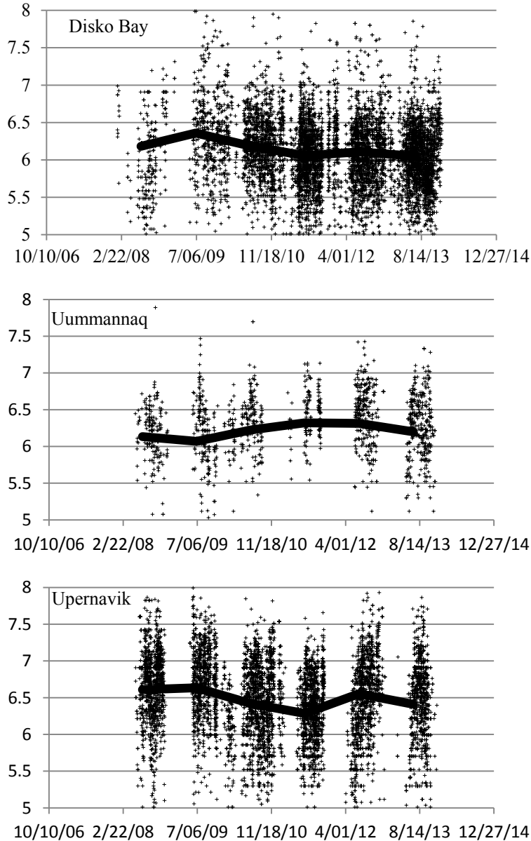
Fig 2.5. Greenland halibut in Division 1A inshore: Standardized longline logbook catch rates. (Points are LogCPUE, line is GLM: \text{logcpue} = \text{overall mean} + \text{yr} + \text{month} + \text{vessel} )
