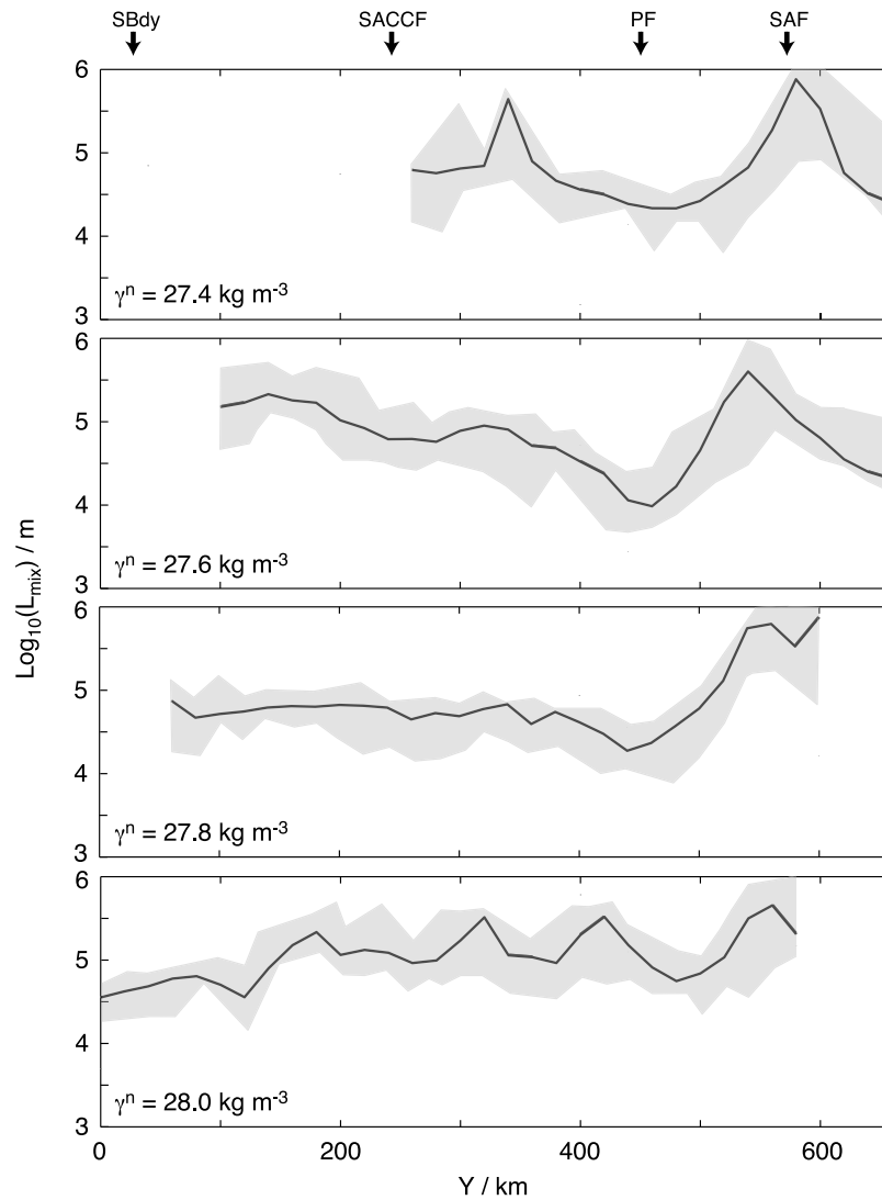
Figure A1. Distribution of \log_{10}(L_{mix}) as a function of Y for four neutral density surfaces ( \gamma^n values indicated in the lower left hand corner of each panel) along the WOCE SR1b section. The black line shows the L_{mix} distribution calculated from ten repeats of the section. The gray-shaded area indicates the one standard deviation envelope of the L_{mix} distributions calculated from all possible pairs of WOCE SR1b section repeats, centered around the mean of all such distributions. The positions of hydrographic fronts are indicated at the top of each set of panels and labeled as in Figures 1 and 2.
