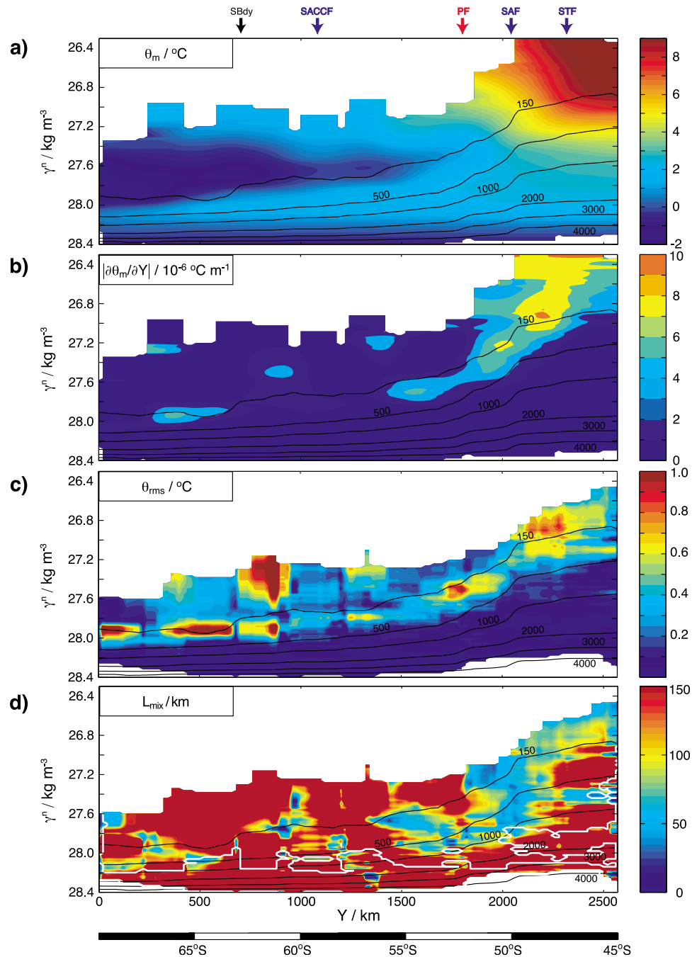
Figure 6. Distributions of (a) \theta_m ; (b) \nabla_n \theta_m ; (c) \theta_{rms} ; (d) L_{mix} ; (e) U_{geos} , the geostrophic velocity relative to the deepest common level; (f) U_e ; (g) c_e^{-1} \kappa and (h) the natural logarithm of (planetary) potential vorticity q , as a function of Y and \gamma^n along the WOCE I6S section. The black lines denote selected pressure contours, labeled in dbar. The white lines in Figures 6d and 6g show the upper boundary of the area of the deep Southern Ocean where \nabla_n \theta_m \approx 0 , and so L_{mix} and c_e^{-1} \kappa are ill-defined. The positions of hydrographic fronts are indicated at the top of each set of panels and labeled as in Figures 1 and 2. Frontal jets interpreted to exhibit (lack) mixing suppression in their upper and intermediate layers are labeled in blue (red), with ambiguous cases indicated in black. Our criterion for categorizing a jet as exhibiting (lacking) suppression is given in the caption of Figure 4.
