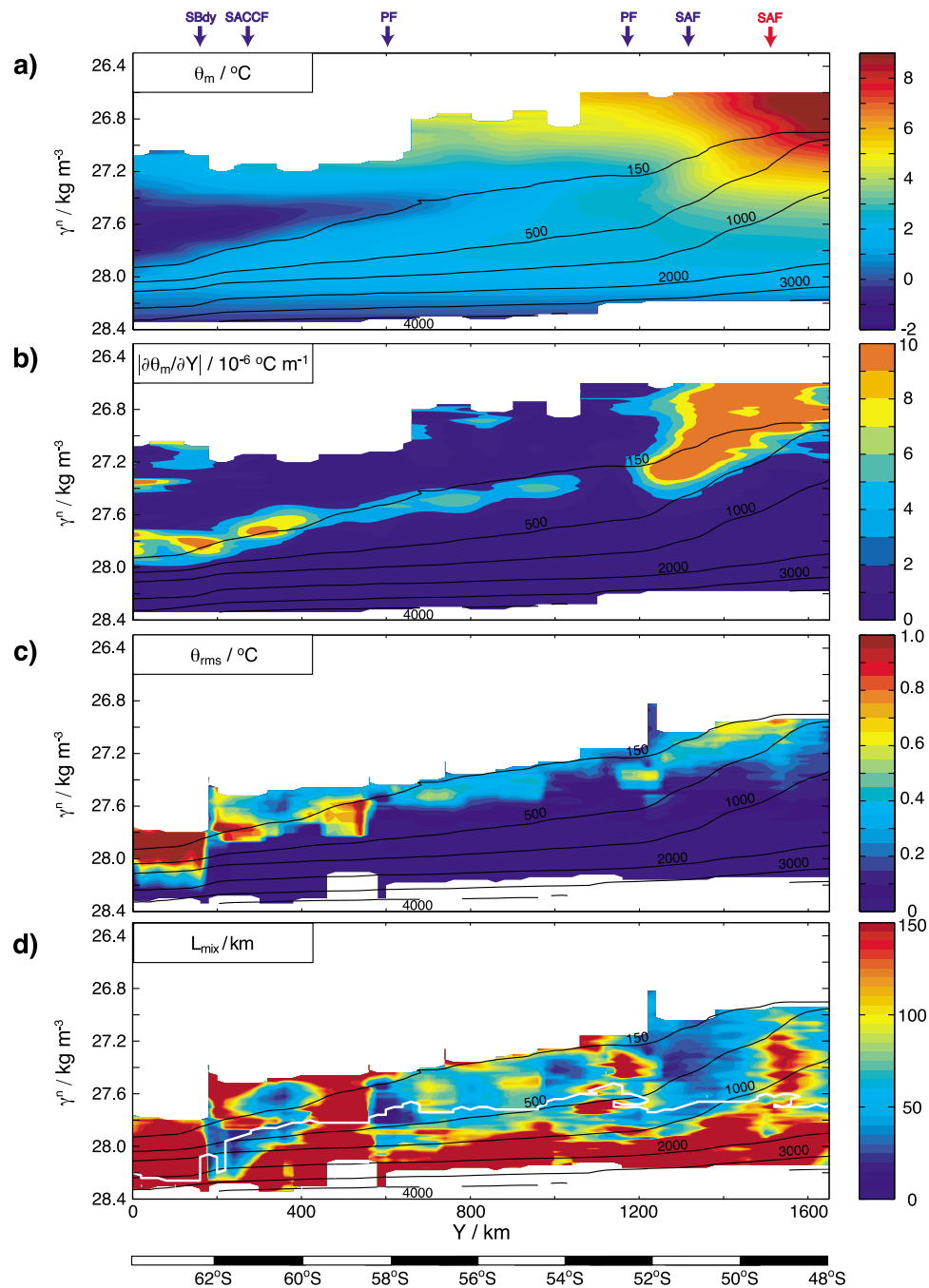
Figure 8. Distributions of (a) \theta_m ; (b) \nabla_n \theta_m ; (c) \theta_{rms} ; (d) L_{mix} ; (e) U_{geos} , the geostrophic velocity relative to the deepest common level; (f) U_e ; (g) c_e^{-1} \kappa and (h) the natural logarithm of (planetary) potential vorticity q , as a function of Y and \gamma^n along the WOCE SR3 section. The black lines denote selected pressure contours, labeled in dbar. The white lines in Figures 8d and 8g show the upper boundary of the area of the deep Southern Ocean where \nabla_n \theta_m \approx 0 , and so L_{mix} and c_e^{-1} \kappa are ill-defined. The positions of hydrographic fronts are indicated at the top of each set of panels and labeled as in Figures 1 and 2. Frontal jets interpreted to exhibit (lack) mixing suppression in their upper and intermediate layers are labeled in blue (red), with ambiguous cases indicated in black. Our criterion for categorizing a jet as exhibiting (lacking) suppression is given in the caption of Figure 4.
