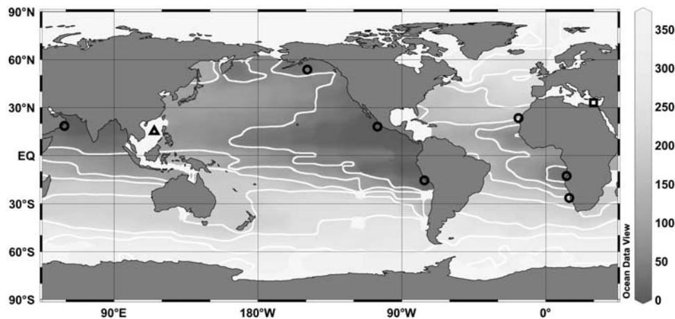
Figure 1. Dissolved O 2 (μmol/kg) on the 27.0 \sigma_{\theta} isopycnals; white contour lines are at 50 μmol/kg intervals. This potential density surface lies near the core of the AAIW and intersects the middepths of the world's WCD zones: the eastern tropical North Pacific, eastern tropical South Pacific, and Arabian Sea. Also visible are the low O 2 zones of Angola-Benguela, NW Africa, and the Subarctic Pacific. The locations of cores discussed in this paper are shown according to their dominant isotopic influence, as discussed in the text, indicated by a circle (denitrification), square (fixation), and triangle (mixed). Oxygen minima zones form where high oxidant demand, generated by the respiration of sinking organic matter from highly productive surface waters, coincides with low rates of oxygen renewal as determined by water mass circulation. Figure generated with Ocean Data View (R. Schlitzer, Ocean Data View, 2003; see http://www.awi-bremerhaven.de/GEO/ODV ) with the WOCE one-time data set.
