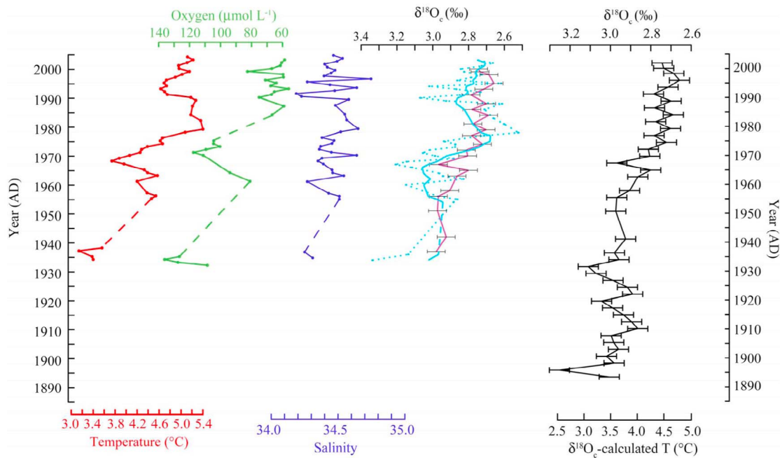
Figure 2. Available instrumental temperature (red), oxygen (green) and salinity (dark blue) records for the St. Lawrence bottom water at a depth >300\text{m} against age (from the CLIMATE database). Theoretical \delta^{18}\text{O}_e (dotted light blue) and smoothed theoretical \delta^{18}\text{O}_e (solid light blue) were calculated from the relationship between salinity, \delta^{18}\text{O}_w , and the instrumental temperature in the isotope paleotemperature equation (1) and is plotted beside \delta^{18}\text{O}_e measured in core CR02-23 (purple). \delta^{18}\text{O}_e measured in core CR02-23 was used to estimate paleotemperature with the equation (1) (black). Error bars report uncertainty for the estimated temperature calculation ( \pm 0.2^\circ\text{C} ), propagated from the analytical precision of the \delta^{18}\text{O}_e measurements ( \pm 0.05\text{‰} ), and for the analytical precision itself.
