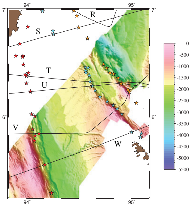
Figure 14. Shaded relief map of swath bathymetry collected by R/V Marion Dufresne (Sibuet 2005) across the Aceh Basin and Sumatran Fault System. Bathymetry is illuminated from the SW and the colour scale in metres is shown to the right of the map. Stars show the location of the West Andaman Fault (red), and the Aceh (teal) and Seulimeum (orange) strands of the Sumatran Fault System on shipboard profiles. Black lines show ship tracks for profiles shown in Fig. 5.
