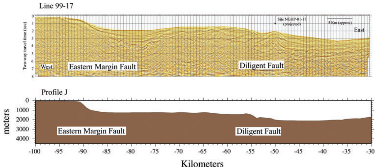
Figure 15. Multichannel seismic reflection line from just east of Little Andaman Island to the lower slope of Invisible Bank. The line was run W–E near 10^{\circ} 38'N , \sim 13 km south of Site NGHP-01-17 and its location is shown on Fig. 4. It is located roughly midway between profile L (Fig. 6) and profile J (Fig. 7). Vertical exaggeration is \sim 2:1 . Nearby bathymetric profile J (Fig. 7) is also shown at the same vertical exaggeration to demonstrate the effect of different vertical exaggerations on the appearance of the bathymetric features.
